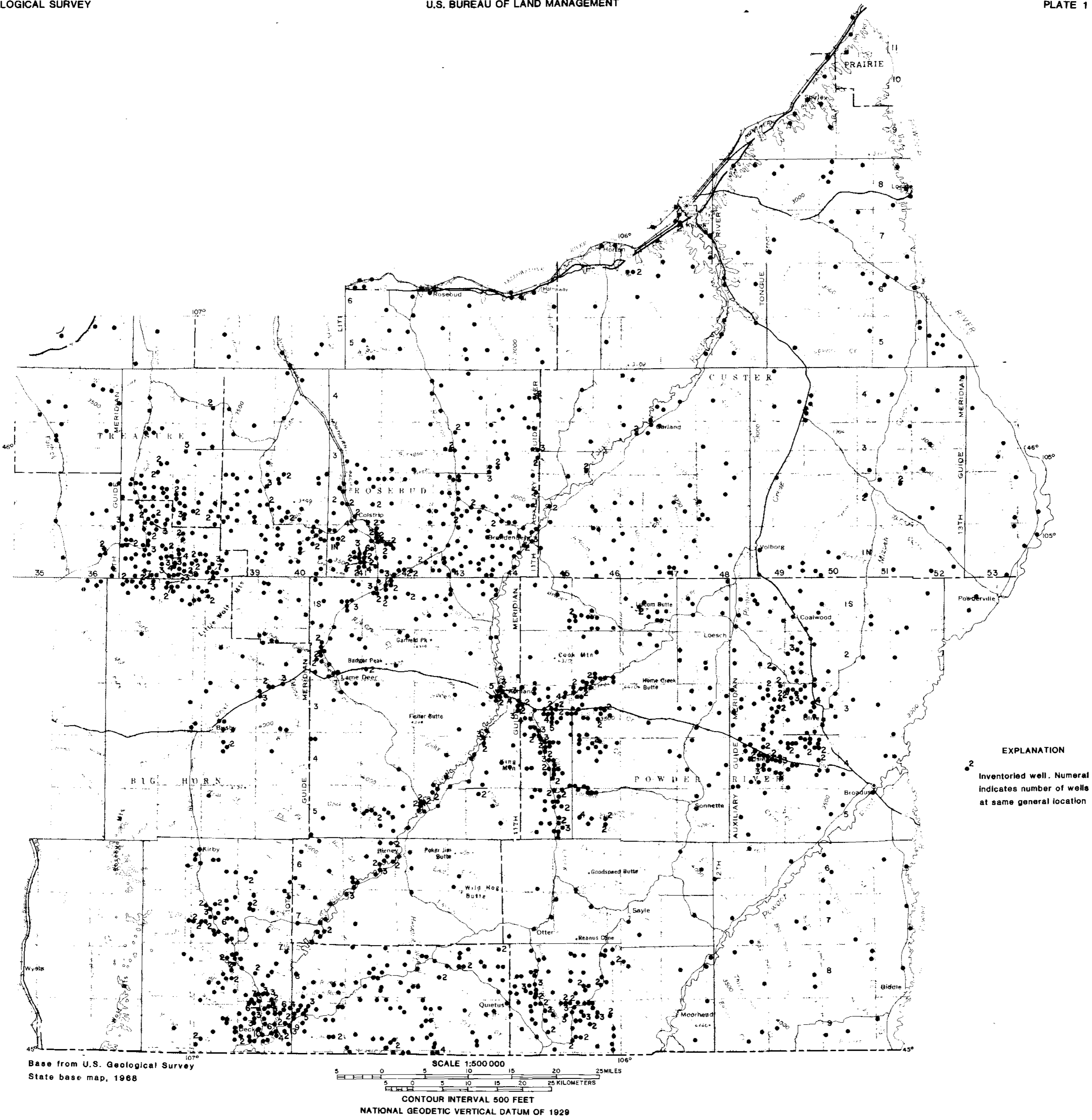
MAP SHOWING LOCATIONS OF INVENTORIED WELLS, NORTHERN POWDER RIVER BASIN, SOUTHEASTERN MONTANA
