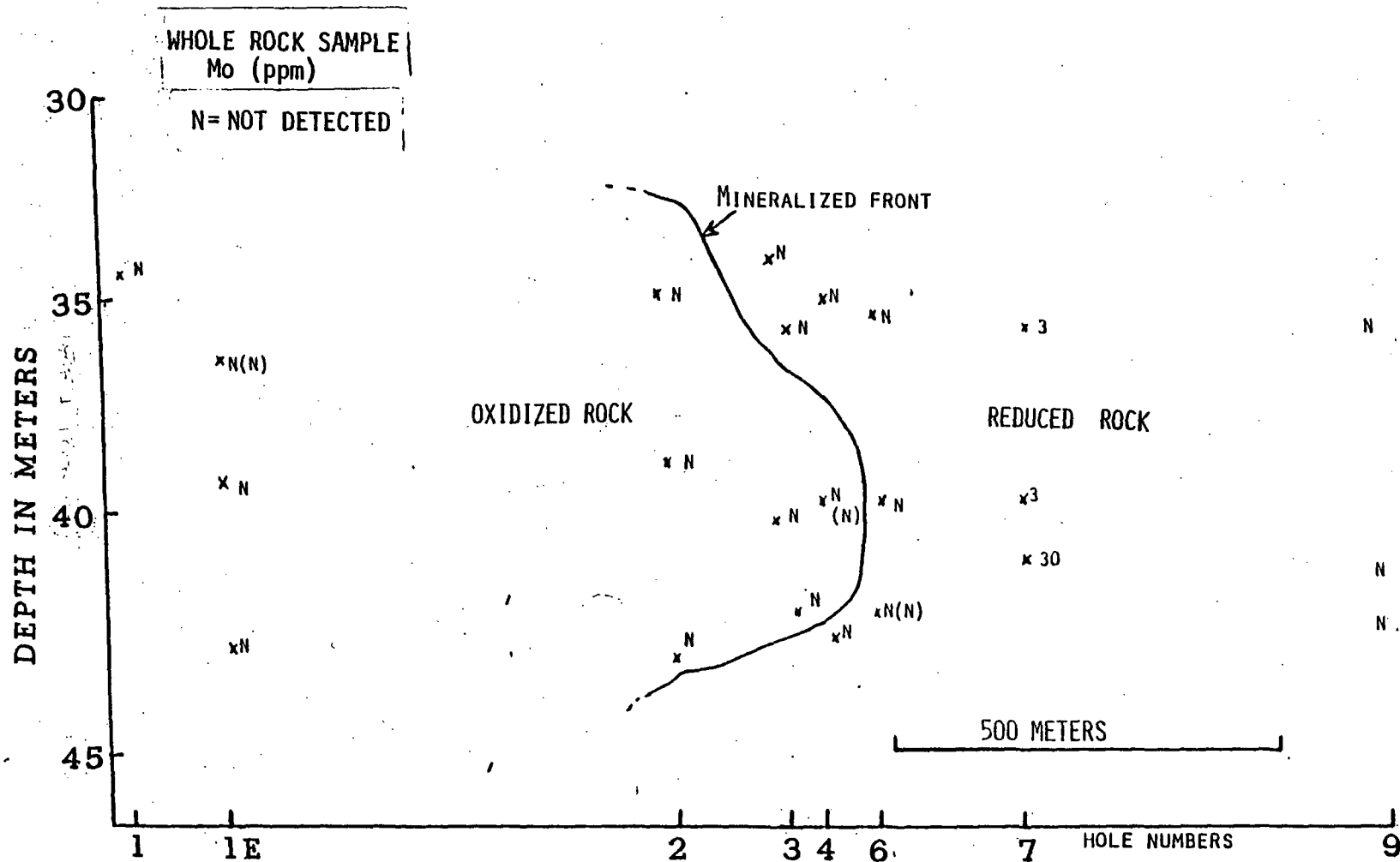
FIGURE 3.-CONCENTRATION OF Mo (PPM) PLOTTED ACCORDING TO THE RELATIVE POSITIONS OF THE SAMPLES. DATA IN PARENTHESES REPRESENT DUPLICATE SAMPLES.
