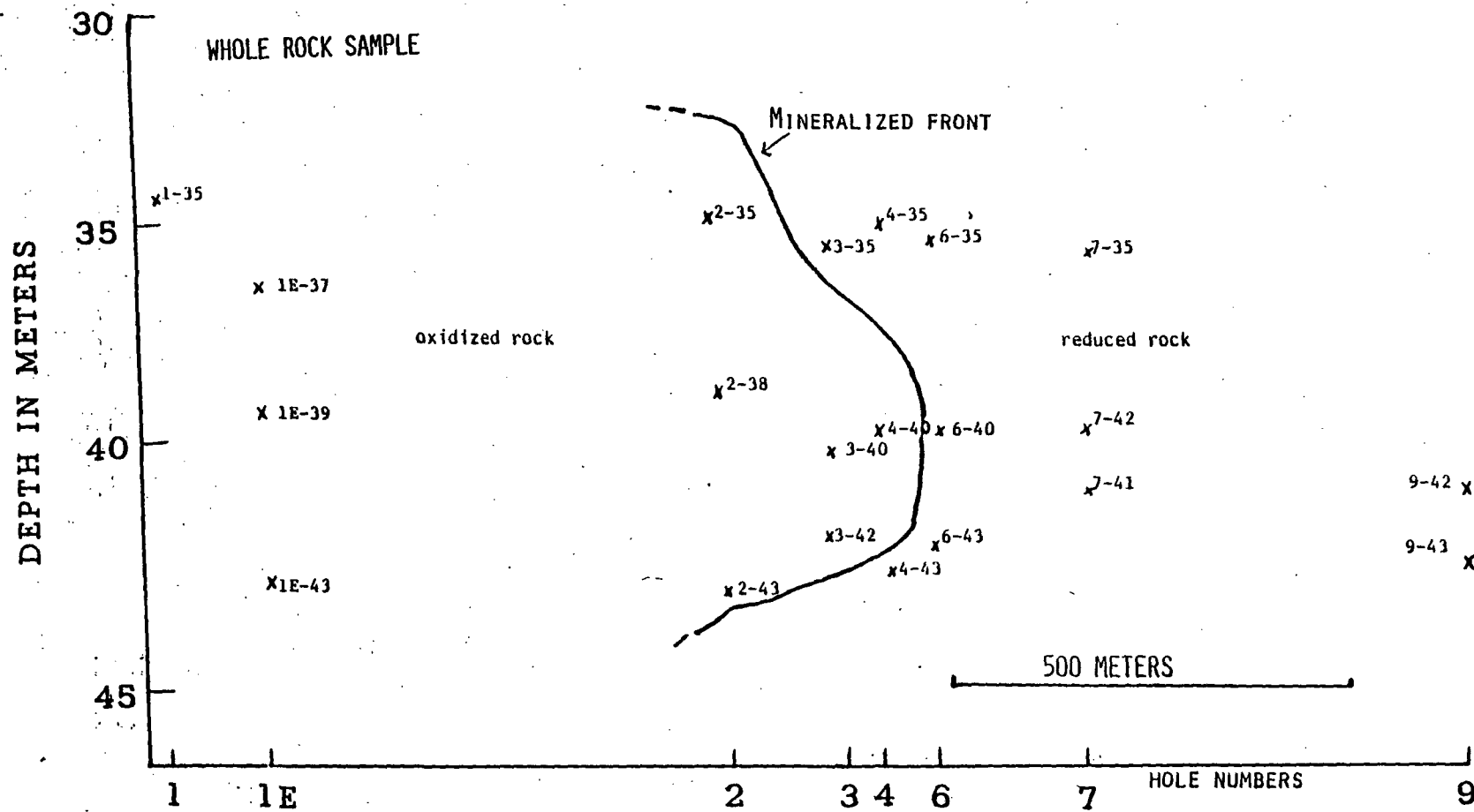
FIGURE 1.- LOCATION OF WHOLE-ROCK SAMPLES.
