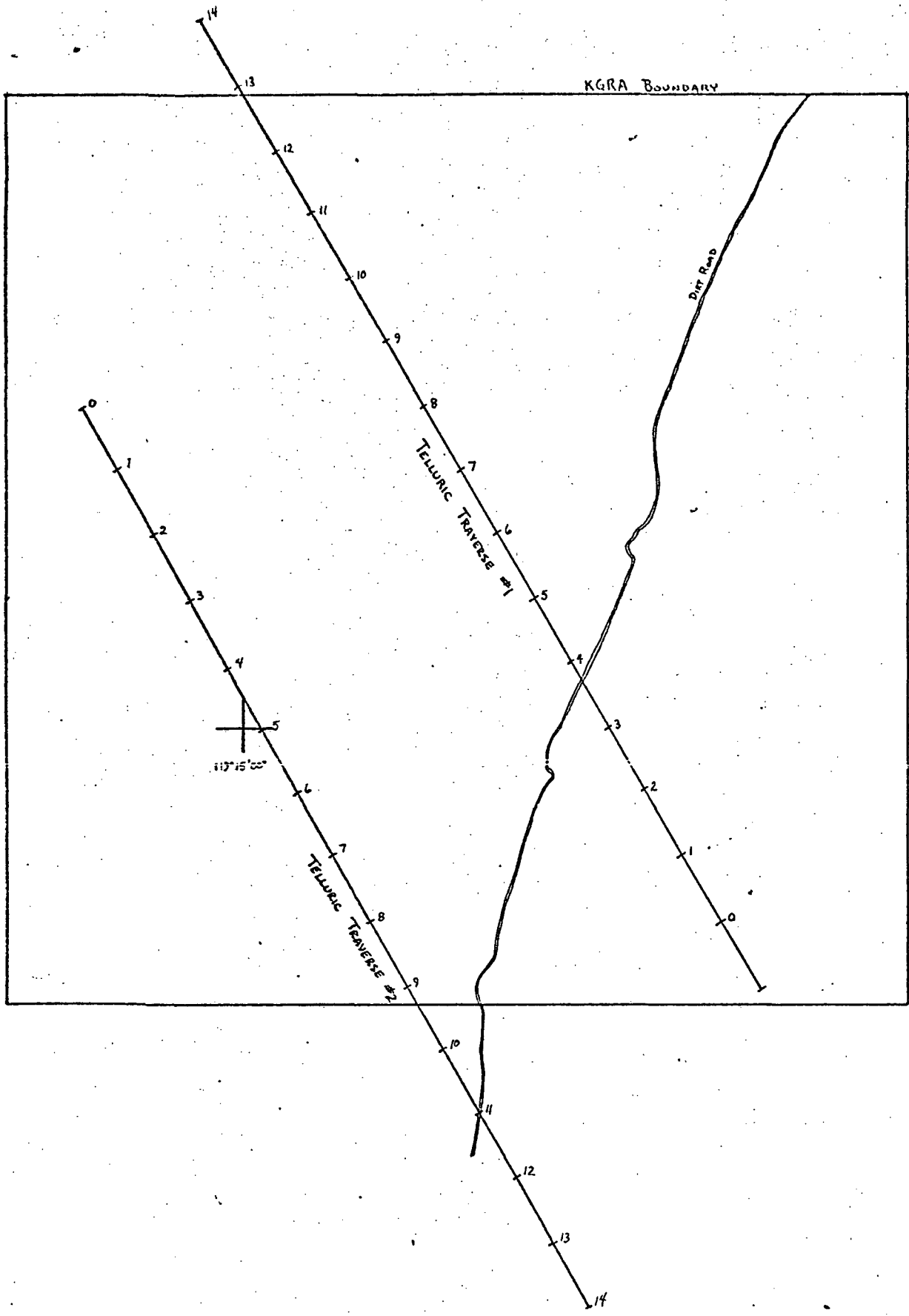
Figure 2. TELLURIC TRAVERSE STATION LOCATION MAP FLY RANCH NORTHEAST KGRA - NEVADA
