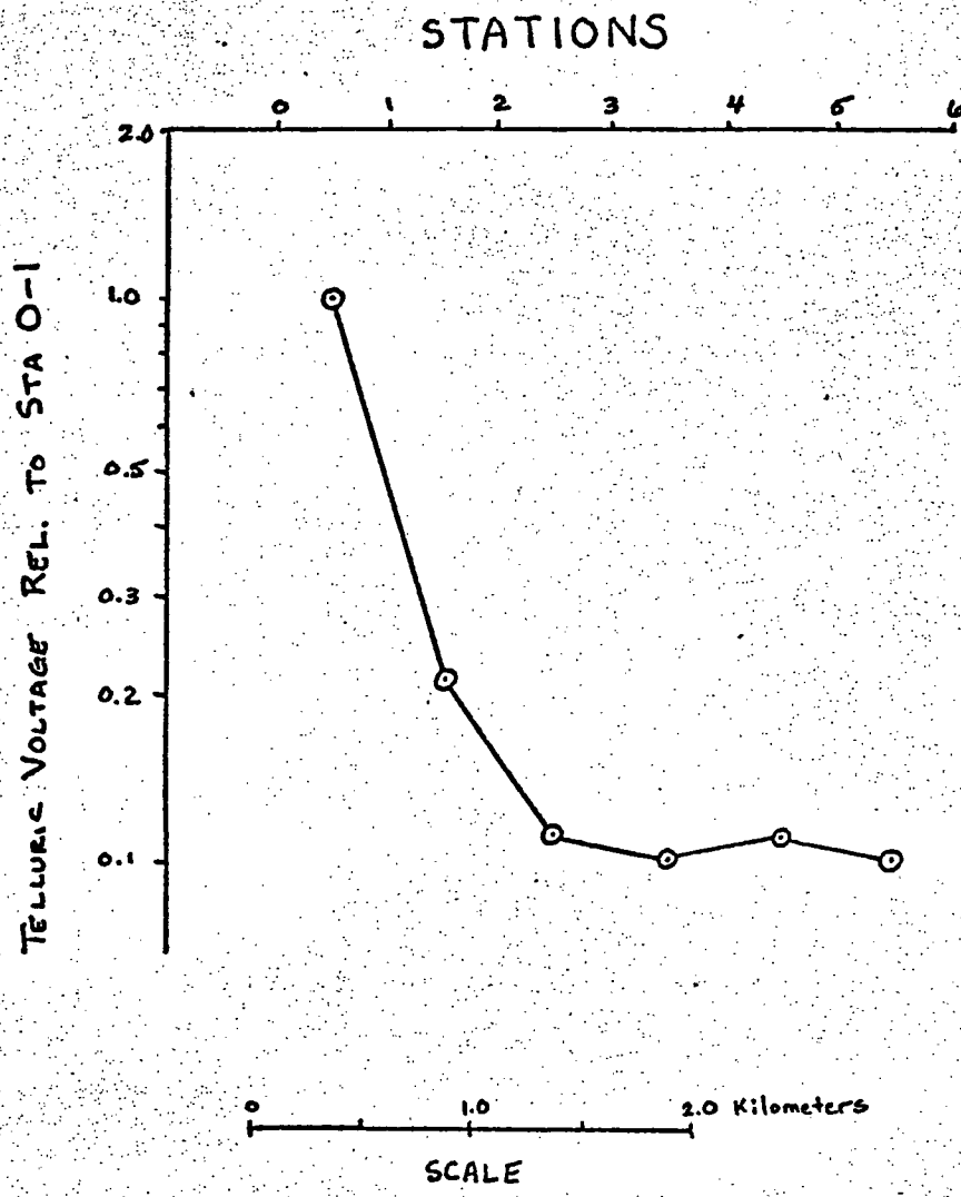
Figure 2. TELLURIC PROFILE GERLACH NORTHEAST KGRA NEVADA
