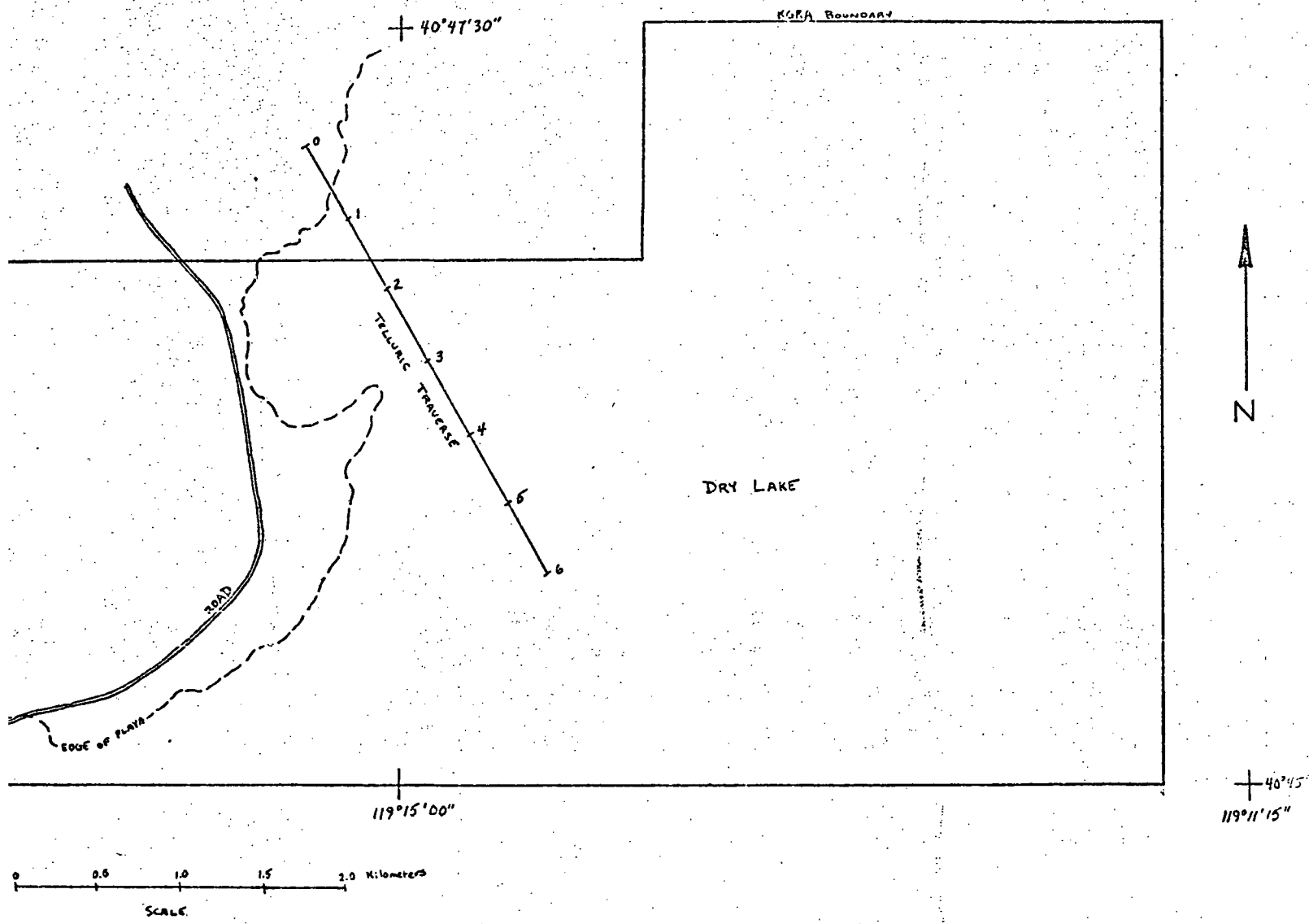
Figure 1. TELLURIC TRAVERSE STATION LOCATION MAP GERLACH NORTHEAST KGRA-NEVADA
