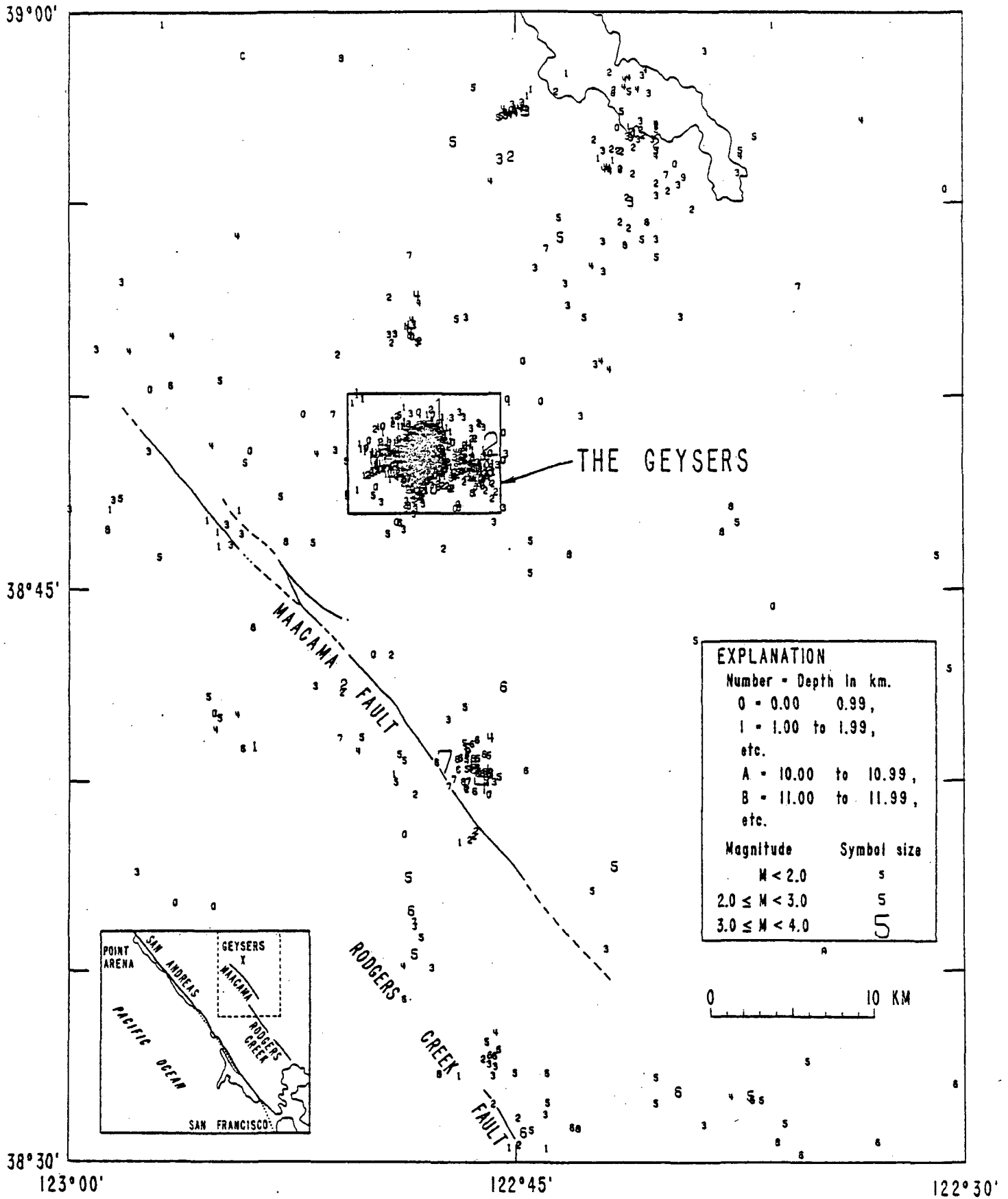
Fig. 1. Recent earthquakes (June 1975-Sept 1977) at The Geysers and along the Maacama and Rodgers Creek faults.
