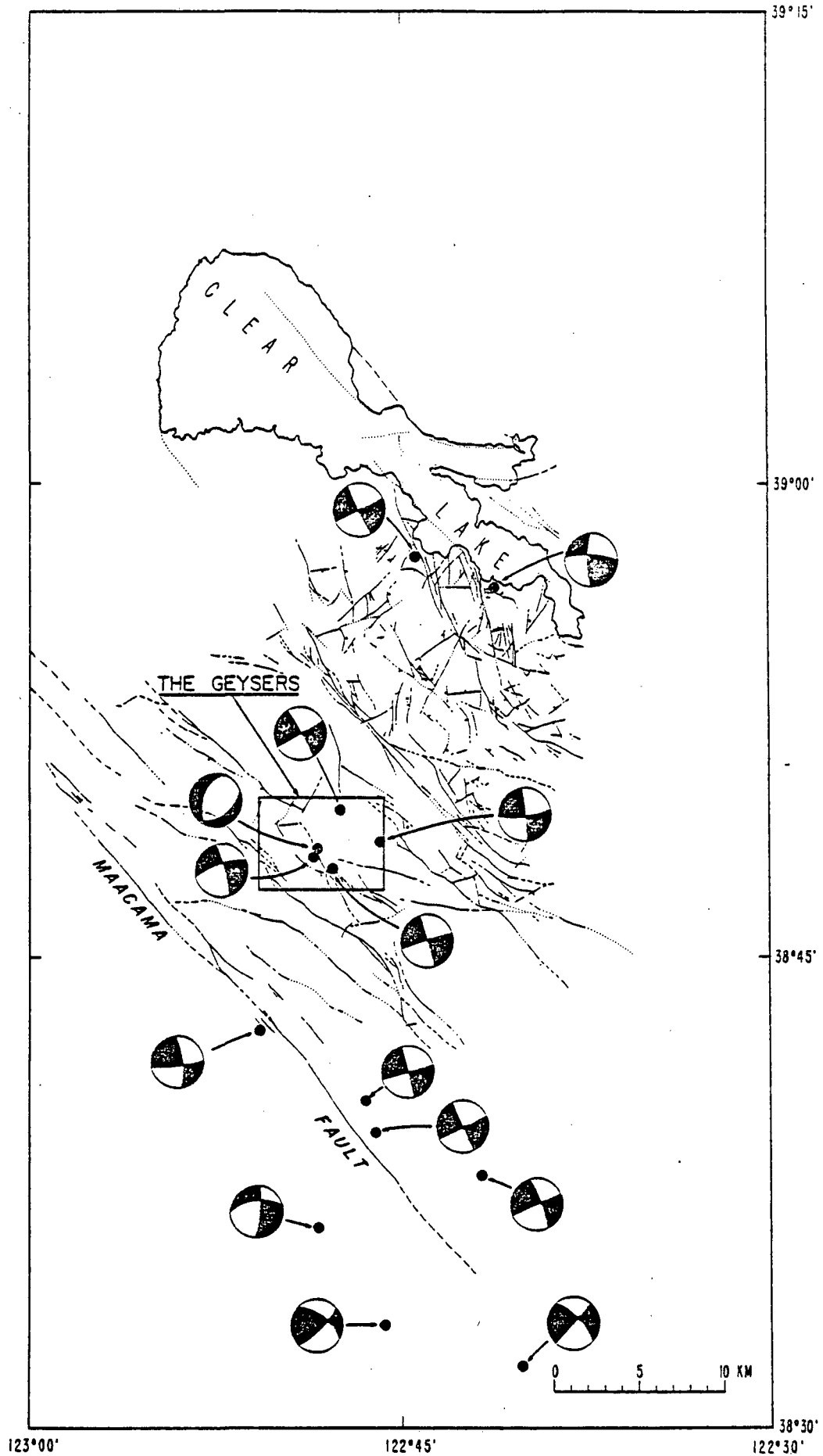
Fig. 8. Representative focal plane solutions for earthquakes at The Geysers and in the surrounding region. Preliminary faults are from McLaughlin and Hearn (unpublished data, 1978).
