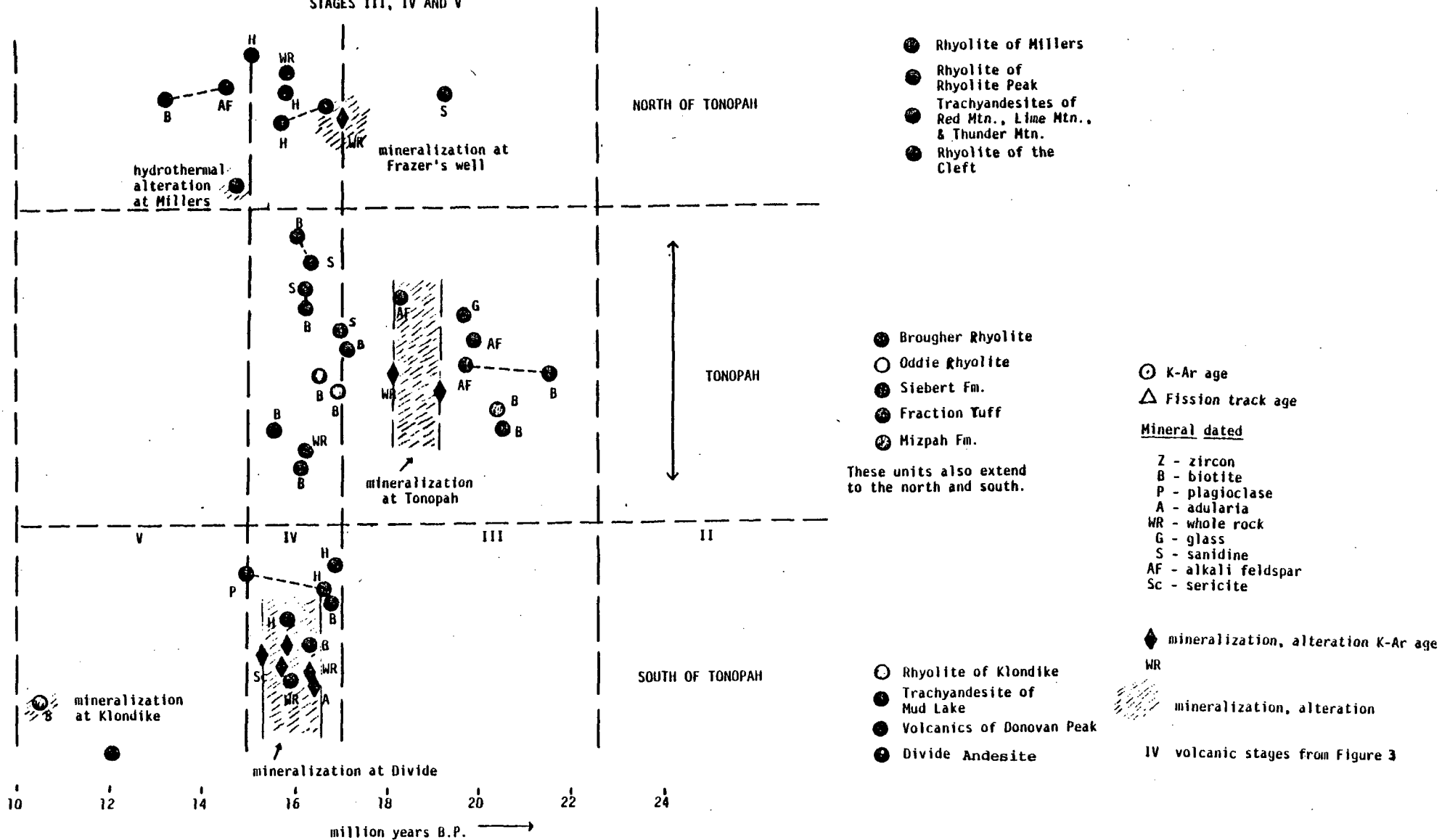
FIGURE 4--INTERPRETIVE HISTORY OF VOLCANIC ACTIVITY AND HYDROTHERMAL ACTIVITY IN AND NEAR TONOPAH, STAGES III, IV AND V
