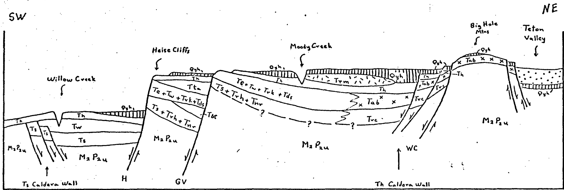
Figure 3.--Highly idealized cross section showing the general structural and stratigraphic relations across the best exposed portion of the Rexburg caldera complex.
