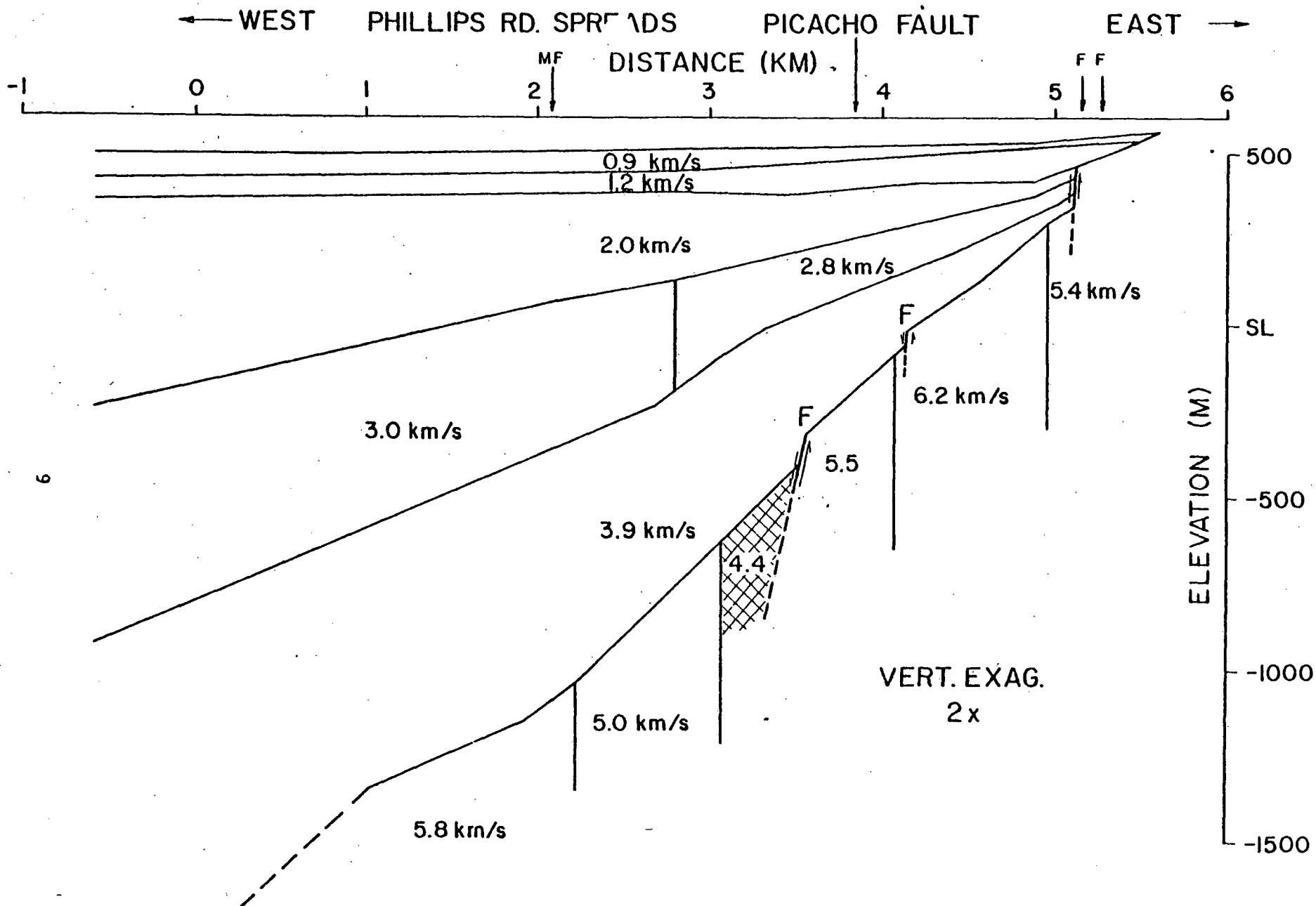
Figure 3.—Seismic velocity model derived from the Phillips Road spreads. Surface traces of the mapped fissures are labeled MF, F, and Picacho fault. Three high angle normal faults are indicated in the basement layer. The cross-hatched zone may represent fractured rock.
