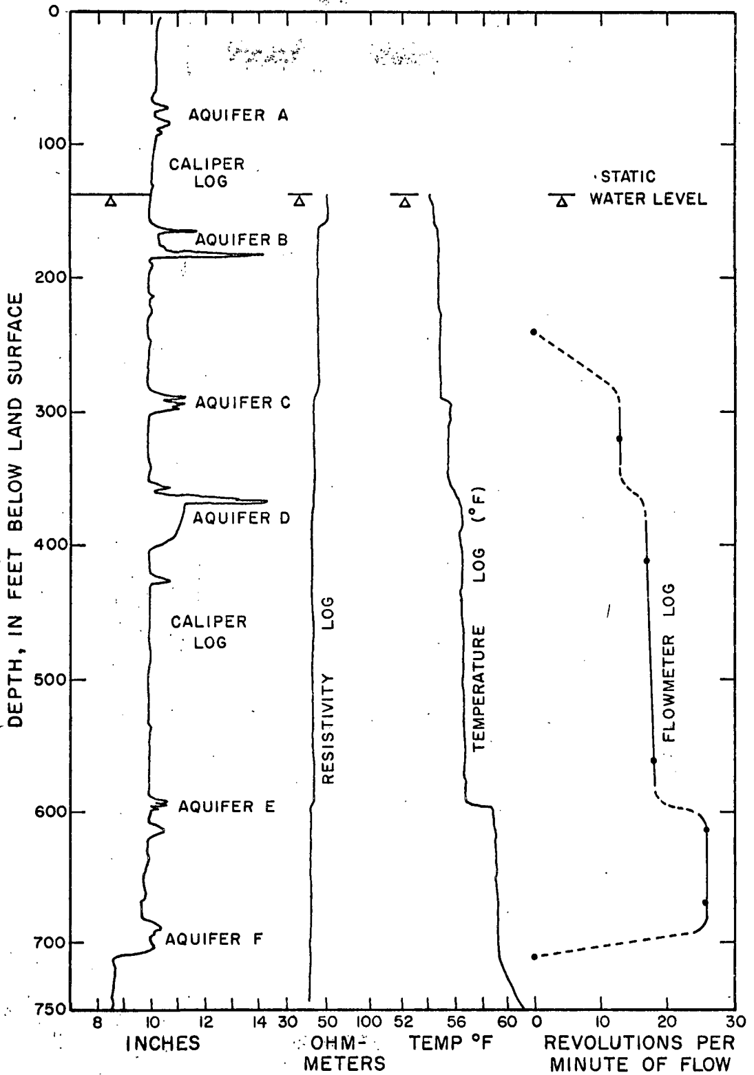
FIGURE 4.--Borehole geophysical logs of Odessa test-observation well, February 5, 1971.
