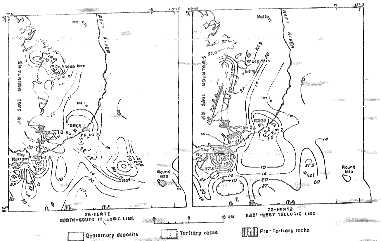
Figure 5.--Audiomagnetotelluric apparent resistivity maps of the southern Raft River Valley. Resistivity contours shown are a logarithmic interval in ohm-metres.
