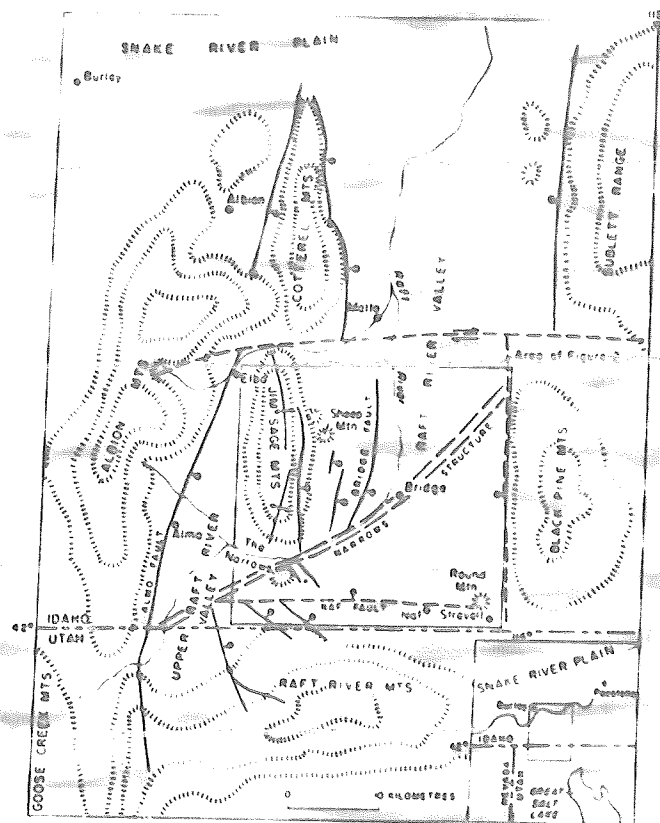
Figure 1.--Map of the Raft River Valley region, Idaho and Utah, showing major faults (bar and ball on downthrown side; arrows indicate relative direction of movement) and anticlines (Jim Sage Mountains only).
