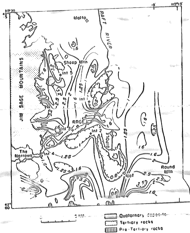
Figure 6.--Normalized bipole-dipole resistivity map of the southern Raft River Valley. Resistivity contours shown are a logarithmic interval in ohm-metres.
