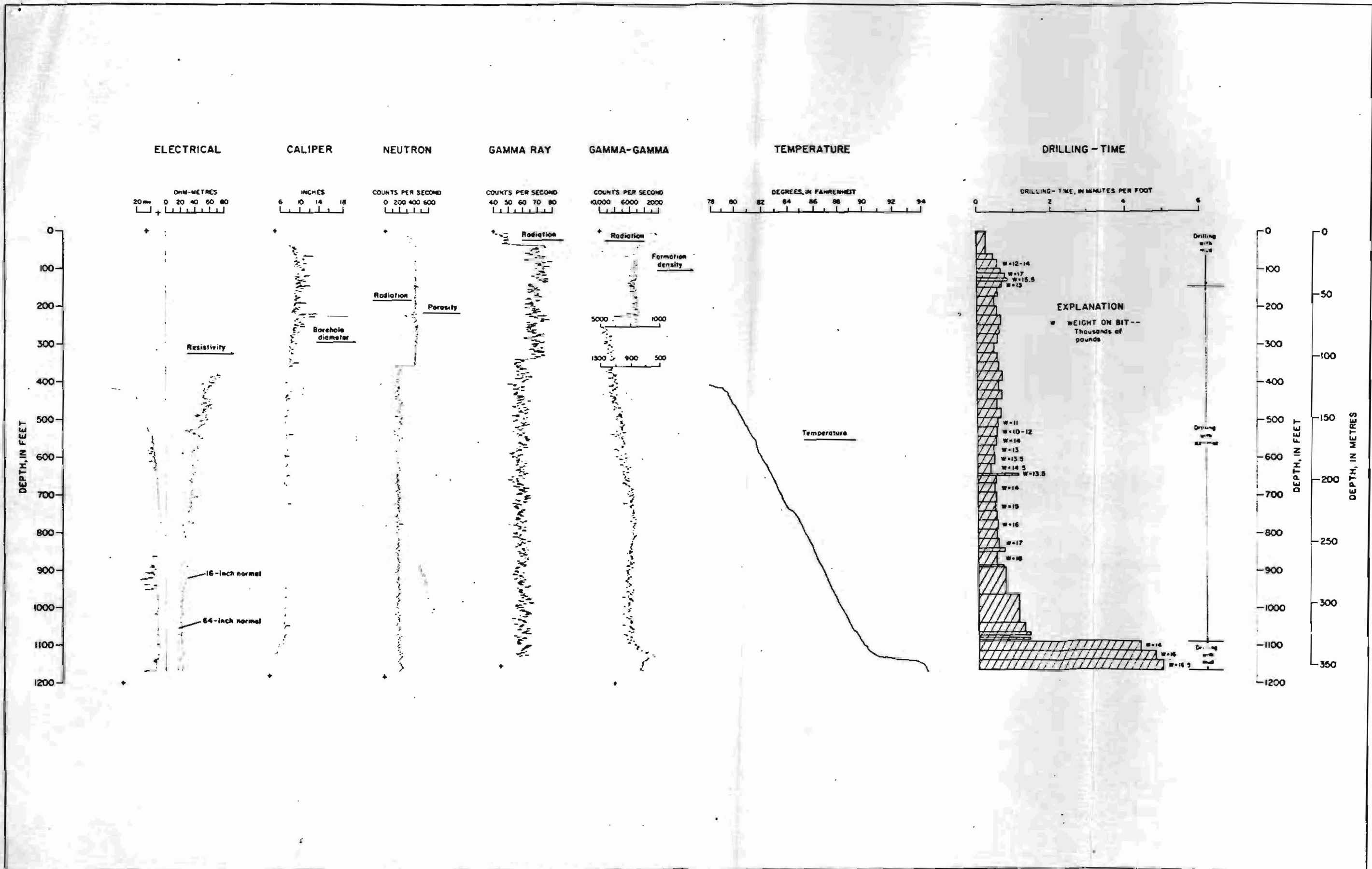
FIGURE 2. Geophysical and drilling-time logs for Leopold Guerra No. 1 test hole (PD-50-07-50), in Red Light Draw
