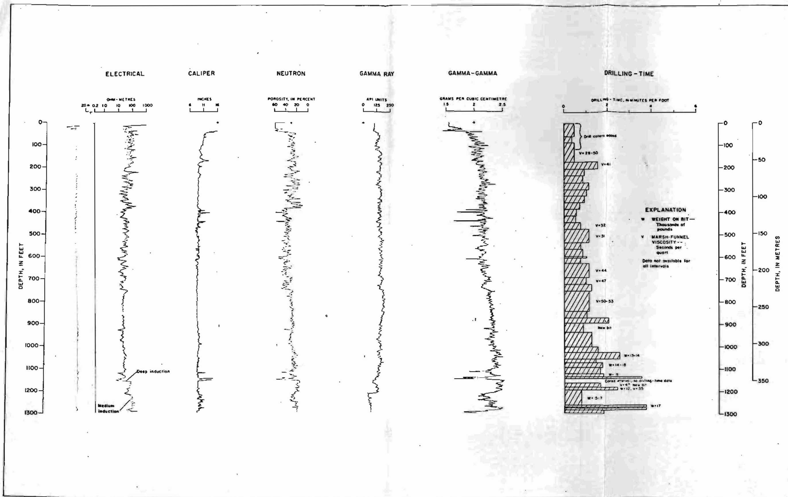
FIGURE 4.-Geophysical and drilling-time logs for Culberson County Airport No. 1 test hole (HL-47-58-603) on Wildhorse Flat
