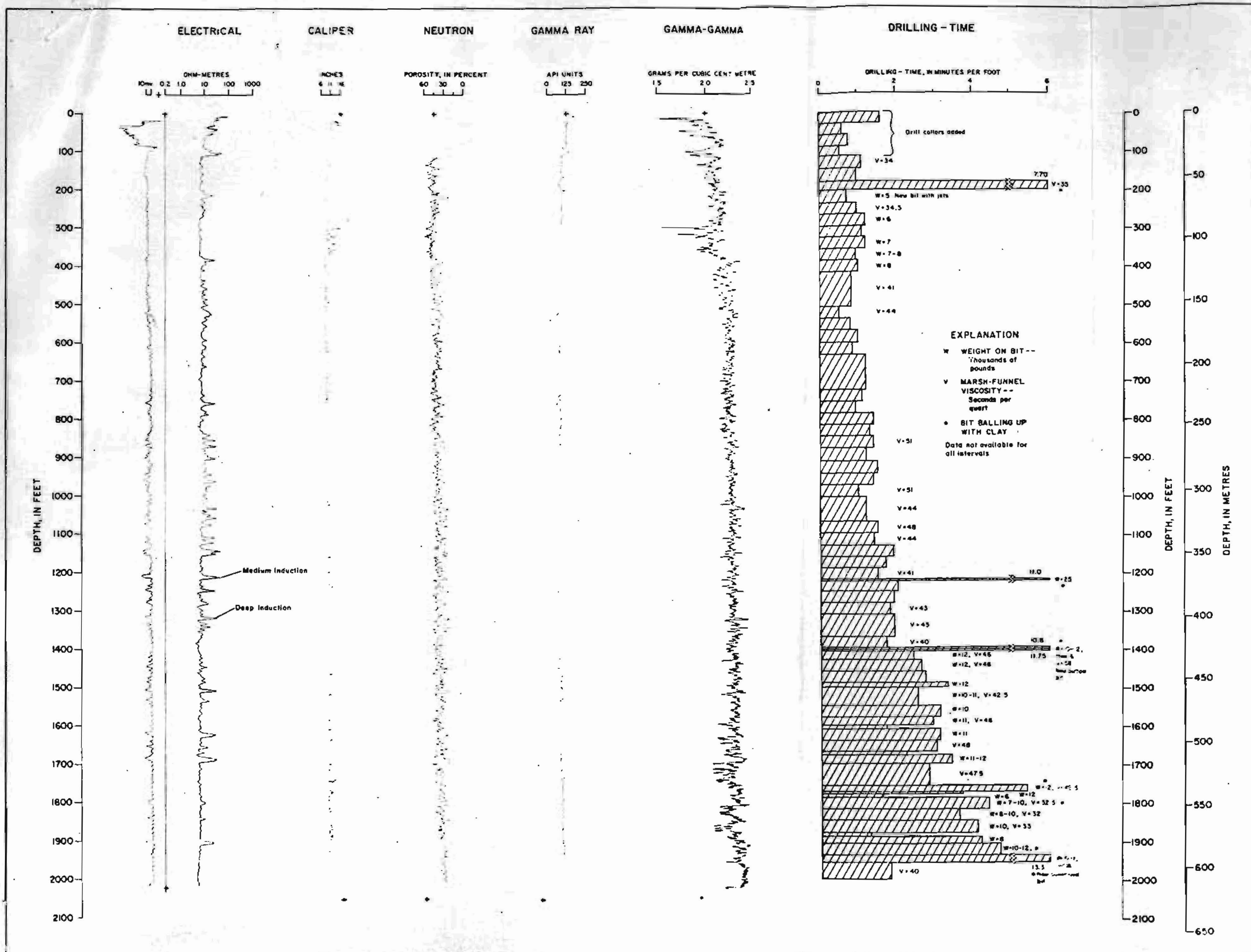
FIGURE 5 Geophysical and drilling time logs for J.C. Davis No. 1 test hole (PD-51 01 504) on Eag's Flat
