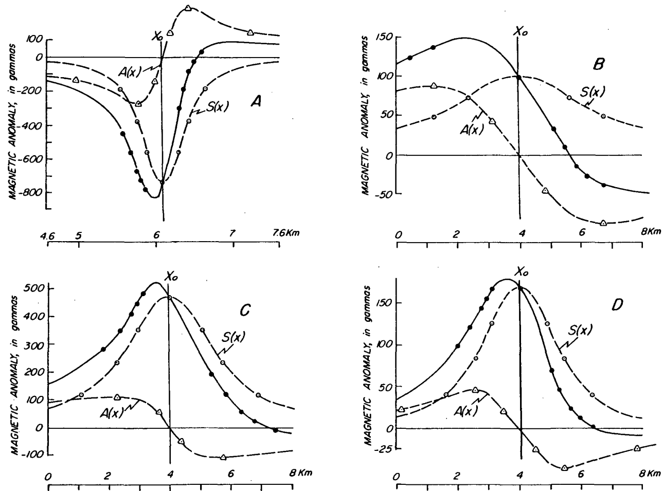
Figure 12.--Analysis of four measured magnetic anomalies by methods of Koulomzine, Lamontagne, and Nadeau (1970) to determine depth, width, and magnetization direction of buried magnetized rocks: A, anomaly along section of profile B-B' in figures 5 and 9; B, anomaly along section of profile A-A' in figures 7 and 10; C, anomaly along section of profile B-B' in figures 7 and 10; and D, anomaly along section of profile C-C' in figures 7 and 10. See figure 11 for explanation of symbols and P. 25 of text for results of analysis.
