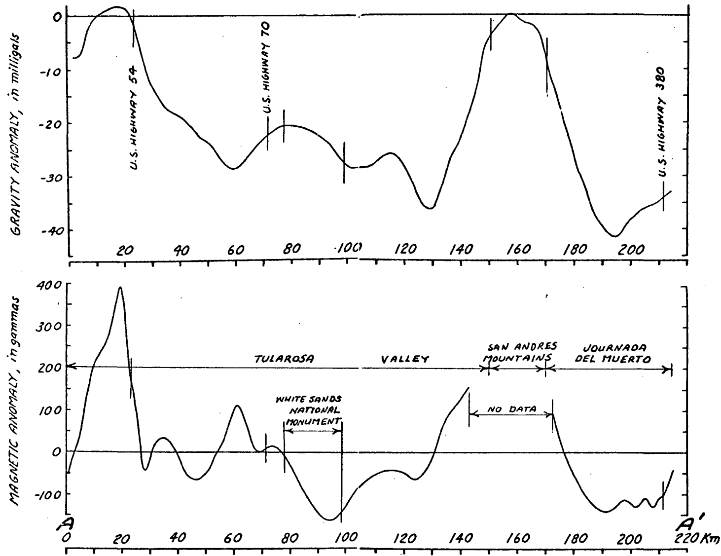
Figure 16.--Residual gravity and magnetic anomalies shown along profile A-A' of figure 1 for a distance of 215 km: starting at Texas-New Mexico line; extending northward across Tularosa Valley, White Sands National Monument, San Andres Mountains west of Mockingbird Gap, and Jornada del Muerto; and ending near U.S. Highway 380.
