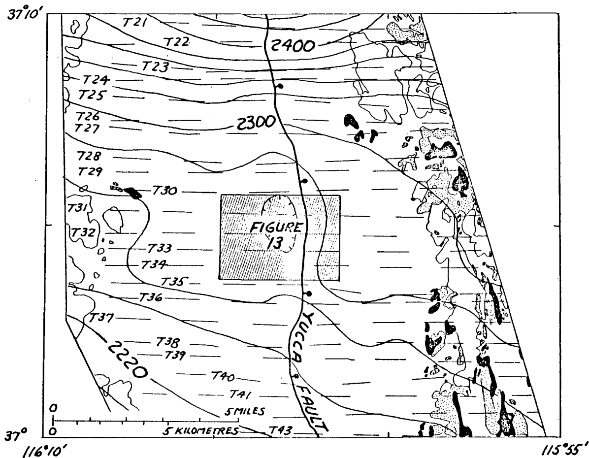
Figure 2.--Aeromagnetic and magnetization map of central part of Yucca Flat showing contours at a 20-gamma interval, flight-line paths, outlines (unshaded) of nonmagnetic Paleozoic sediments, outlines (dotted) of normally magnetized volcanic rock, outlines (black) of reversely magnetized Rainier Mesa Member, trace of Yucca fault, and outline of figure 13. Bar and ball are on the low-standing side of the Yucca fault.
