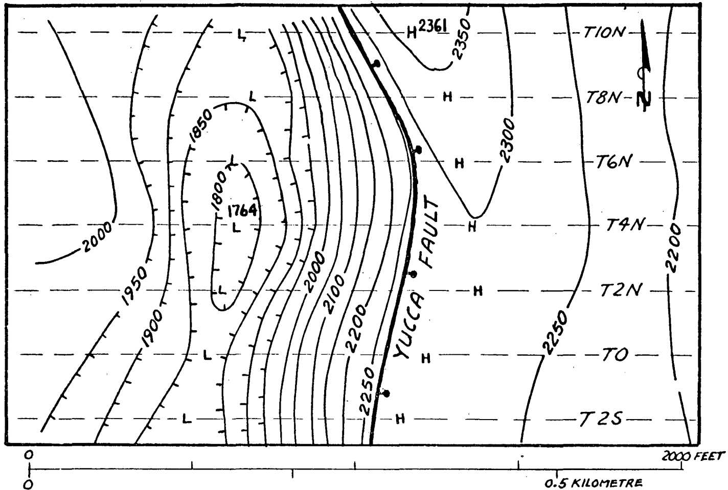
Figure 14.--Ground magnetic map of area outlined on figure 13, showing contours at a 50-gamma interval; flight-line paths, with H marking points of maximum anomaly and L marking points of minimum anomaly; and trace of Yucca fault.
