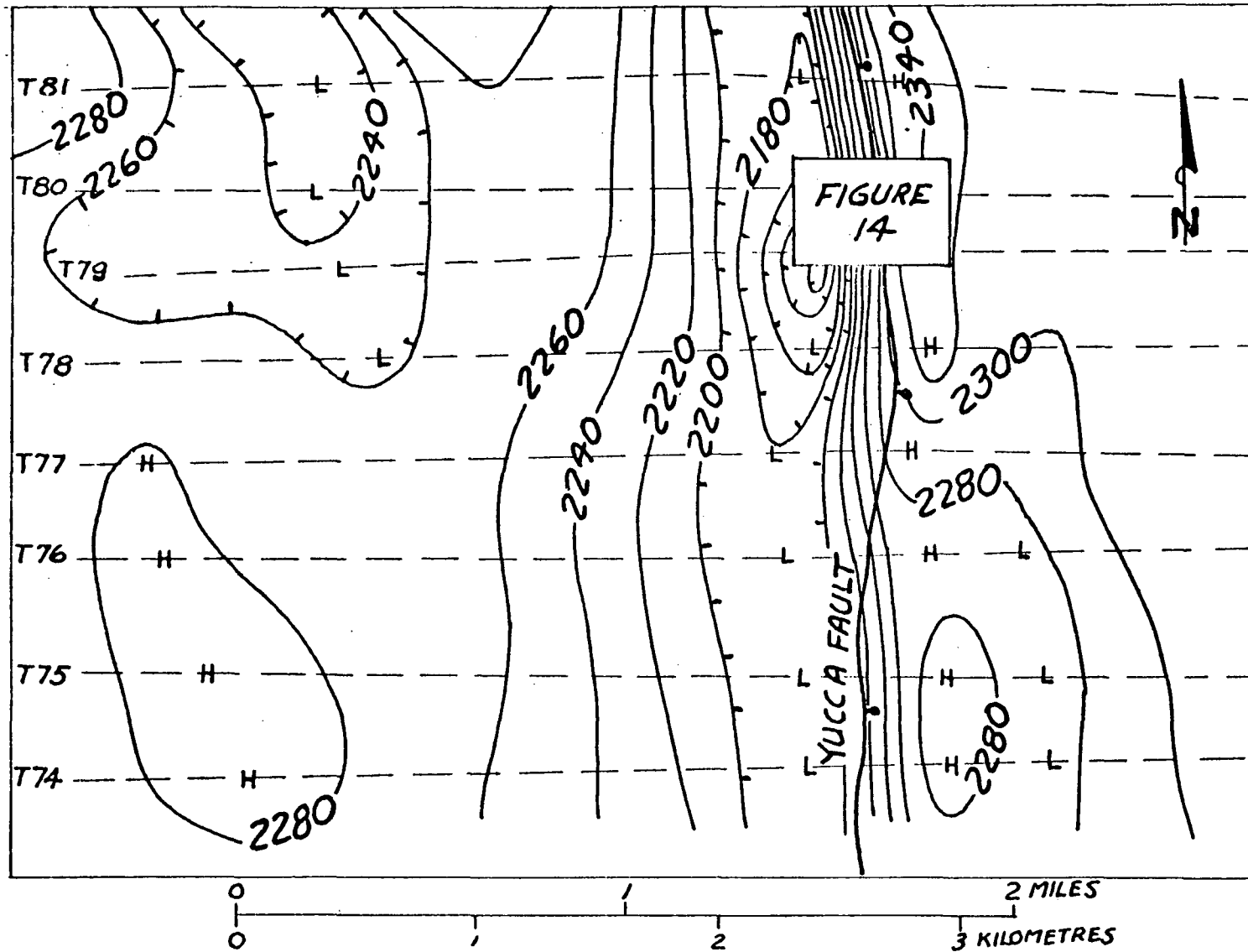
Figure 13.--Aeromagnetic map of area outlined on figure 2, showing contours at a 20-gamma interval; flight-line paths, with H marking points of maximum anomaly and L marking points of minimum anomaly; trace of Yucca fault; and outline of figure 14.
