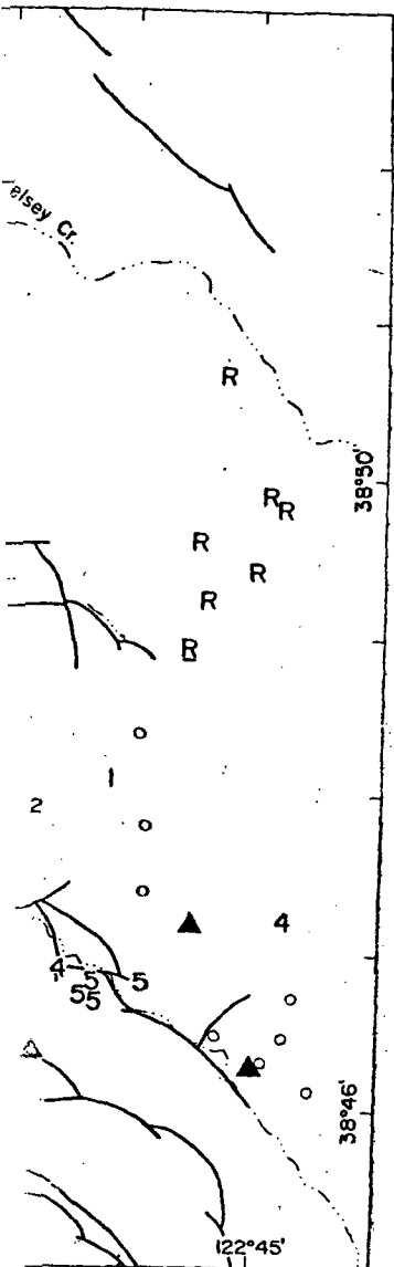
a locations (triangles), epicenters (circles), steam wells (circles), in McNitt [1968]. Possible extension faults.
