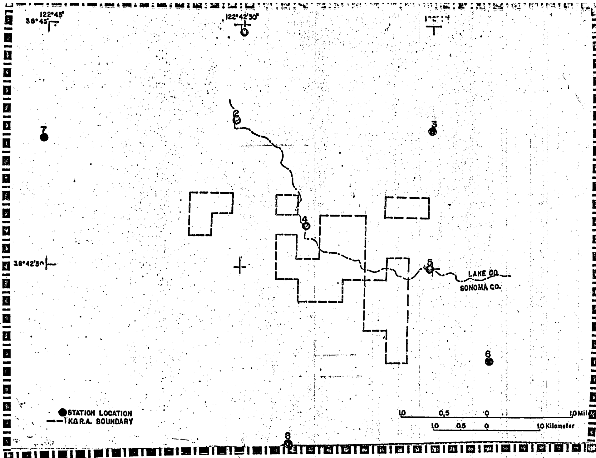
AUDIO-MAGNETOTELLURIC STATION LOCATION MAP GEYSERS-CALISTOGA CALIFORNIA
