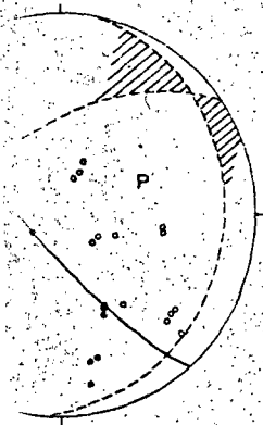
Figure 1. First-motion radiation pattern for an earthquake from The Geysers and (b) in the nodal plane and dilatational first motions (b) in the compressional and dilatational first motions (a) in the dilatational first motions (b) in the compressional first motions, respectively.
