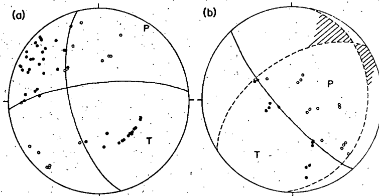
Fig. 2. Lower hemisphere equal-area projections of the first-motion radiation pattern for earthquakes (a) in the main epicenter trend running westward from The Geysers and (b) in the cluster 3\frac{1}{2} km SE of power plants 1 and 2. Compressional and dilatational first motions are represented by dots and circles, respectively. Bisectors of the compressional and dilatational quadrants are plotted at T (tension axis) and P (pressure axis), respectively.
