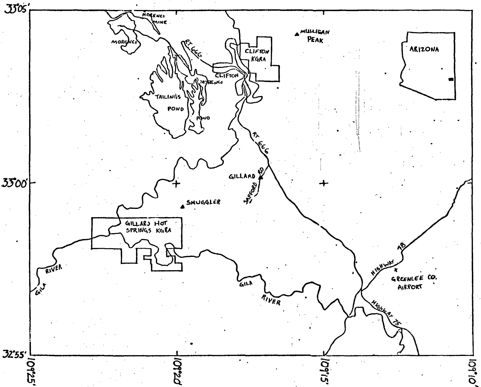
Fig. 1 Location map of the general region of gravity data and KGRA's.
