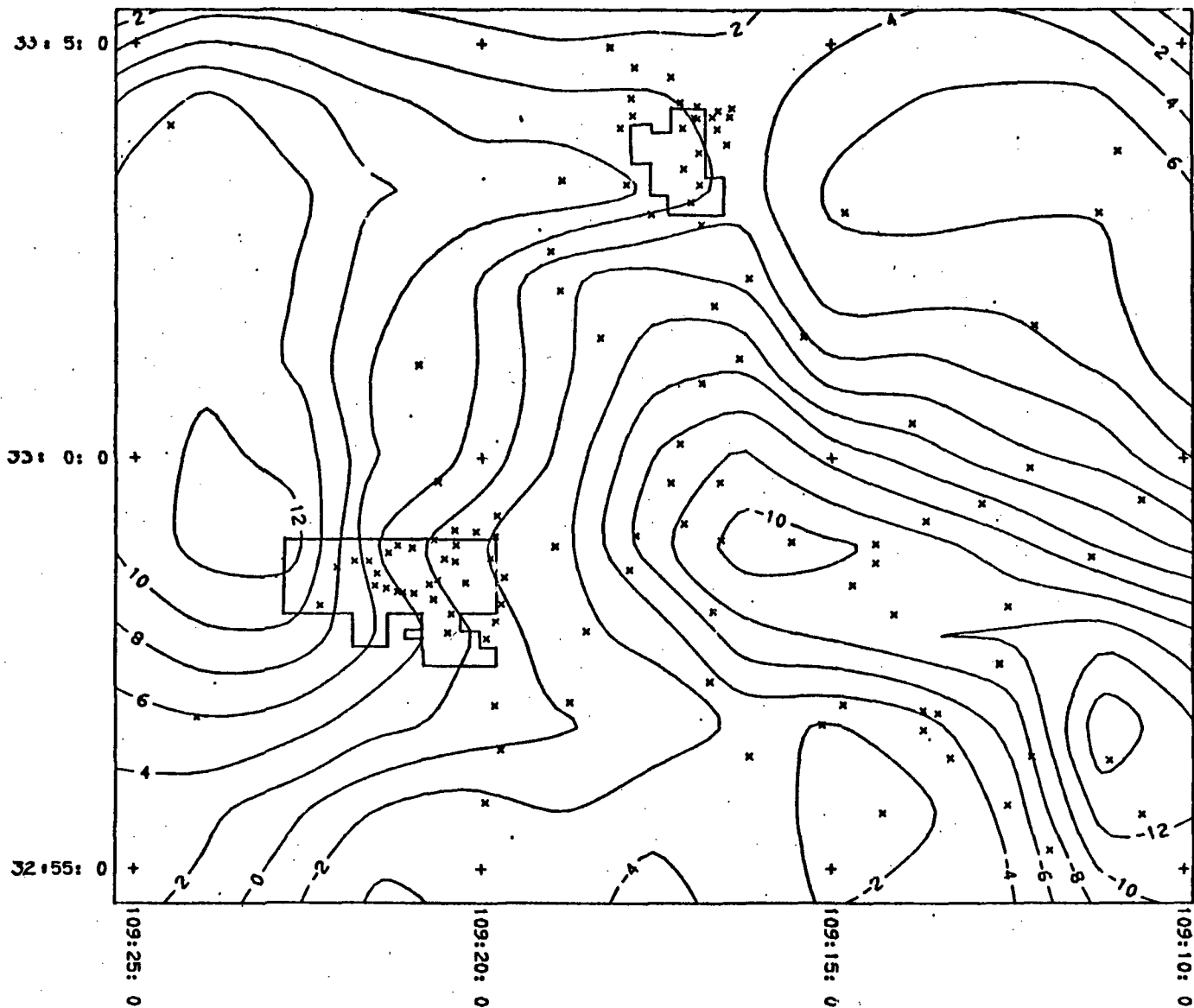
Fig. 2 Residual complete Bouguer anomaly contour map, derived by removing the second order polynomial fit from the regional field extending from 32°45' to 33°15'N latitude and 109°00' to 109°30' W longitude. Contour interval, 2 mgal. X, gravity station.
