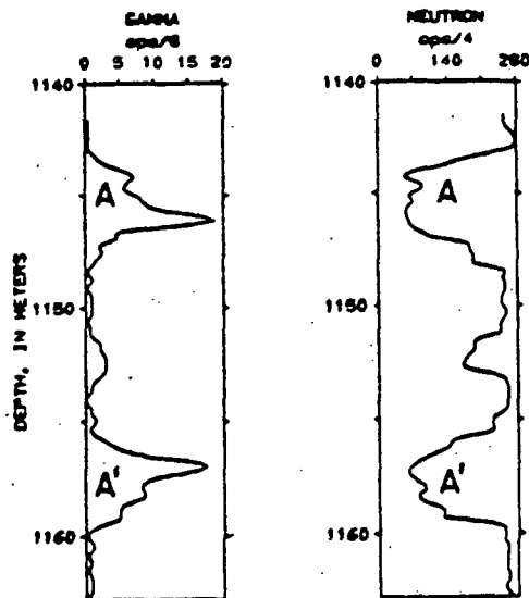
Figure 6.--A section of the Salt Valley well showing the gamma-ray and neutron-neutron well log responses for the limbs (A and A') of a fold.
