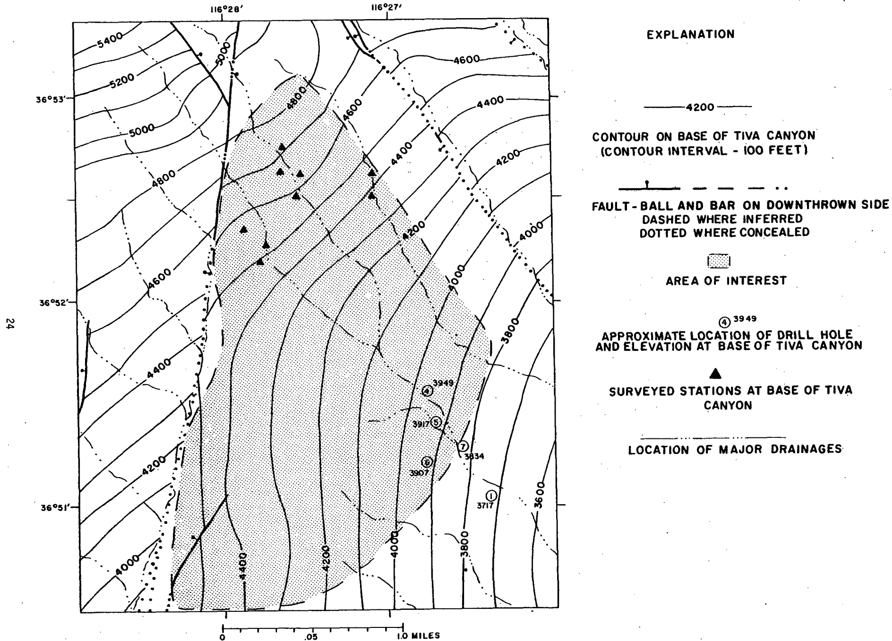
FIGURE 6-- STRUCTURE CONTOUR MAP OF BASE OF TIVA CANYON MEMBER AT NORTHERN YUCCA MOUNTAIN
