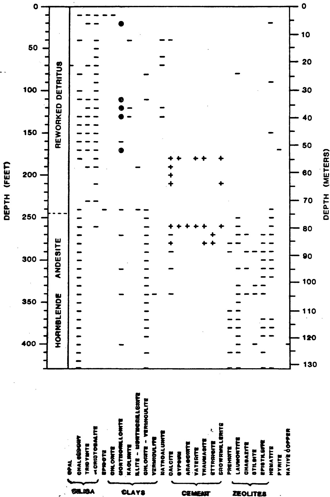
Figure 2. Distribution of vapor-phase minerals, hydrothermal alteration minerals, and drilling cement "+" and drilling mud "•" contaminants in drill cuttings from Lost Creek drill hole.
