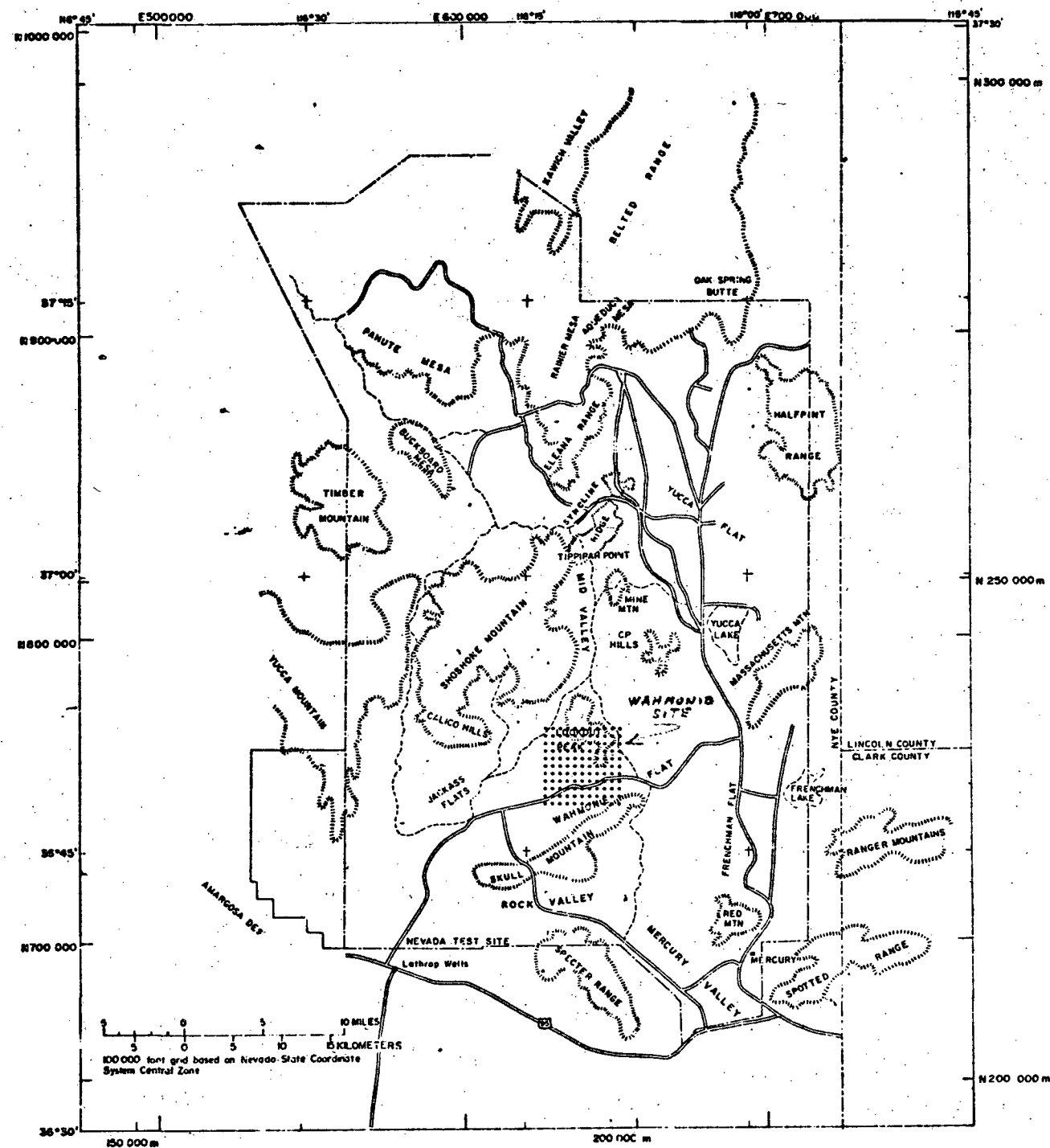
Figure 1. Index map showing the location of the Nevada Test Site and the Wahmonie area
