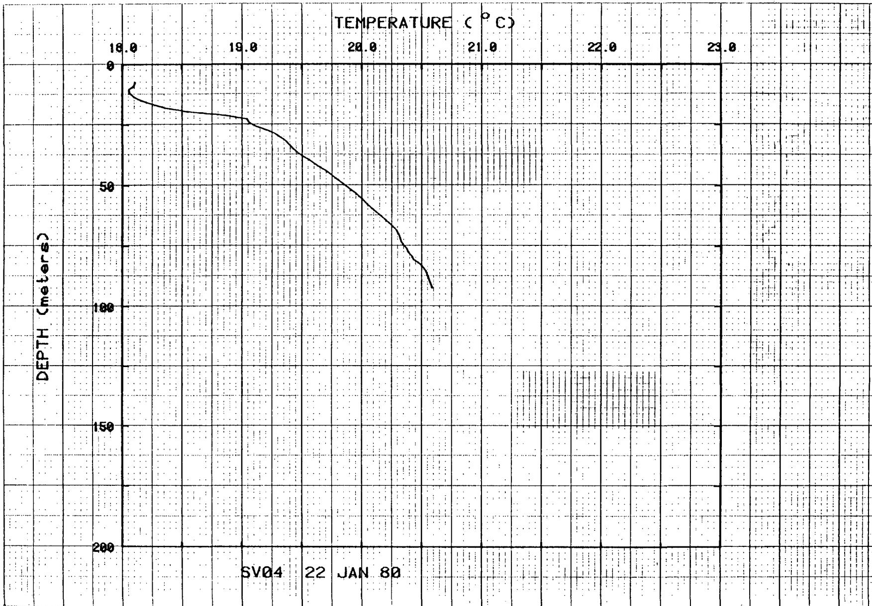
Figure 69. Temperatures for hole SV04.
