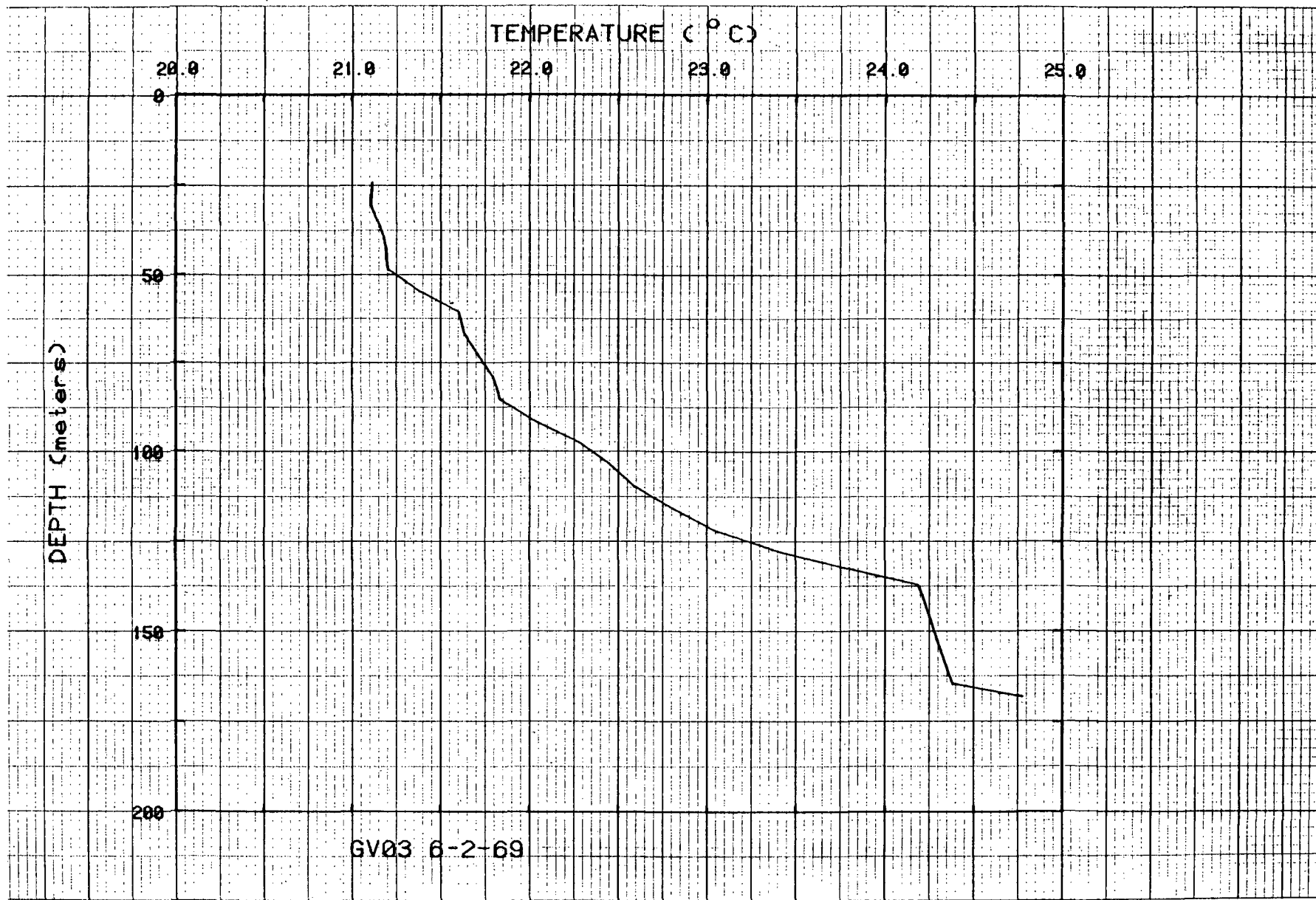
Figure 12. Temperatures for hole GV03.
