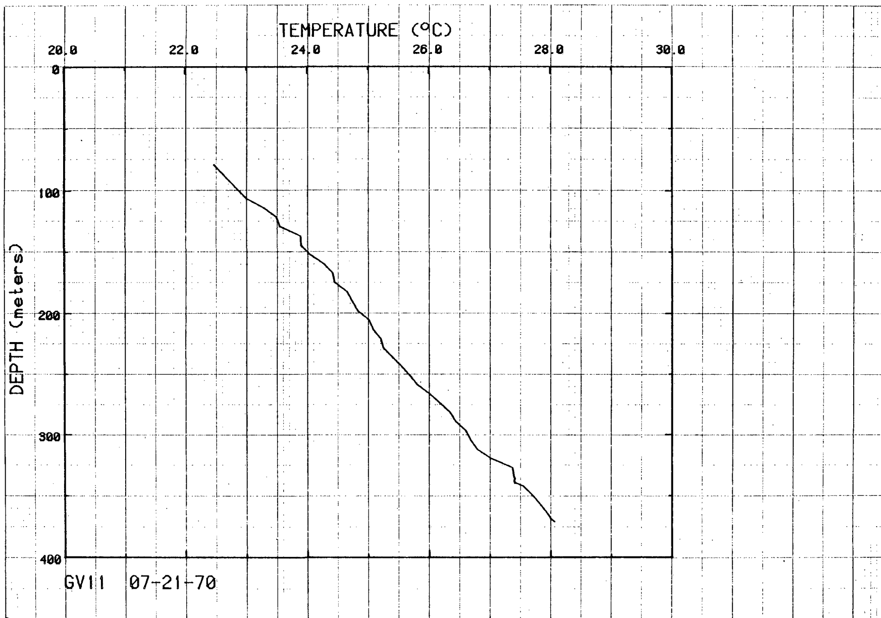
Figure 19. Temperatures for hole GV11.
