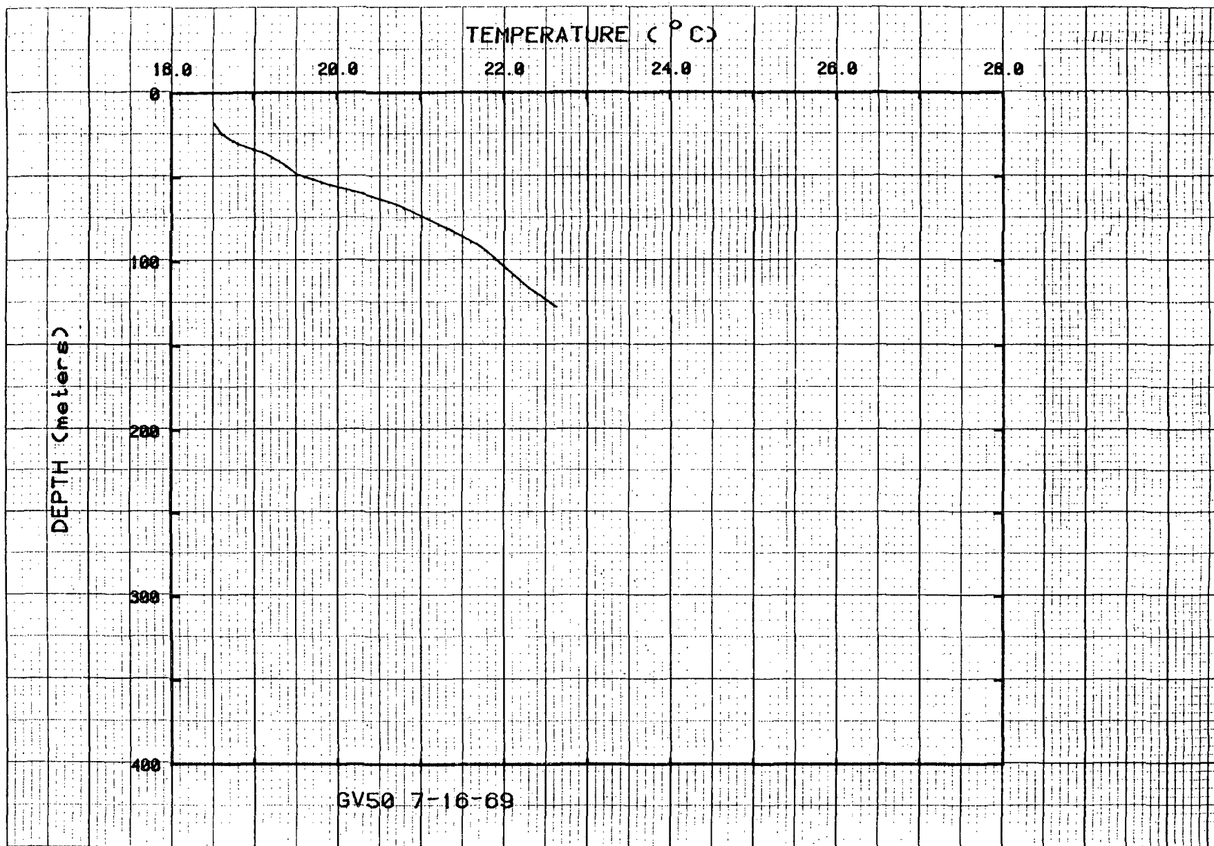
Figure 57. Temperatures for hole GV50.
