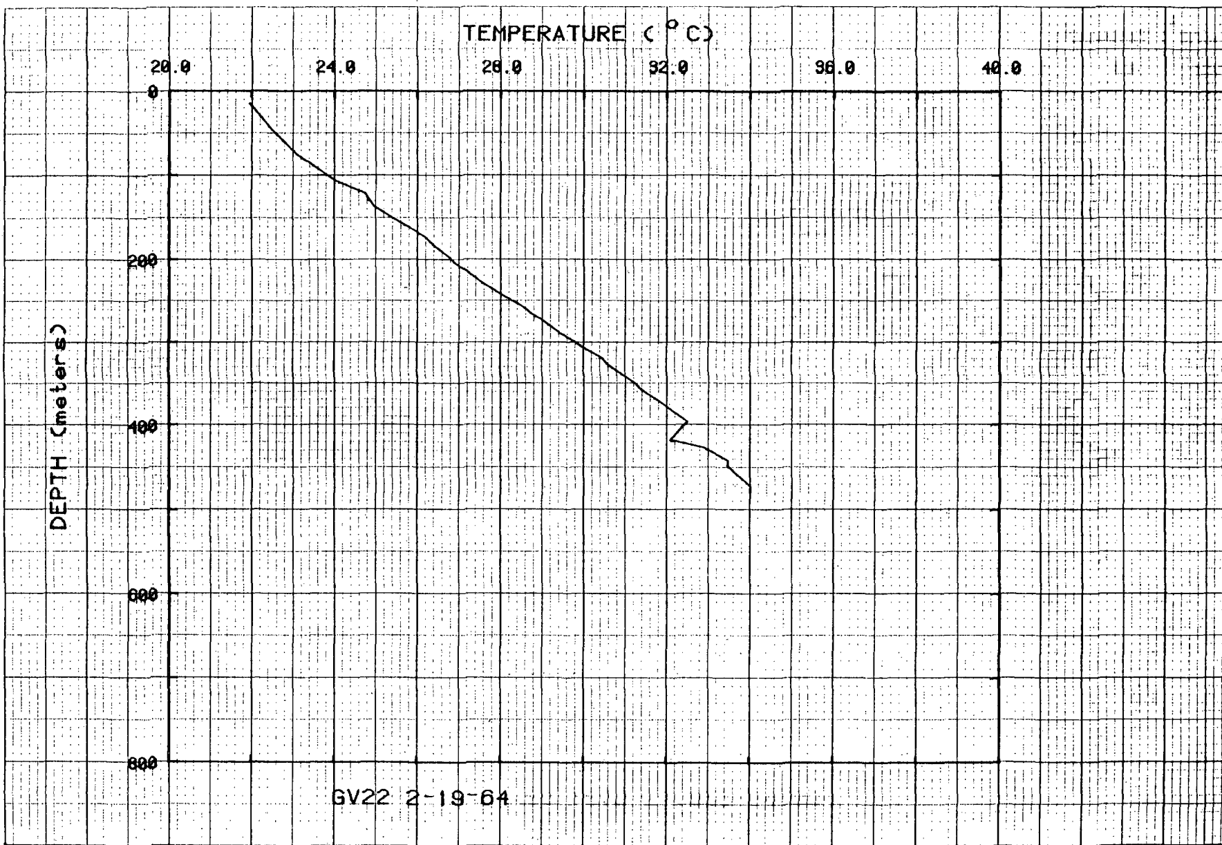
Figure 30. Temperatures for hole GV22.
