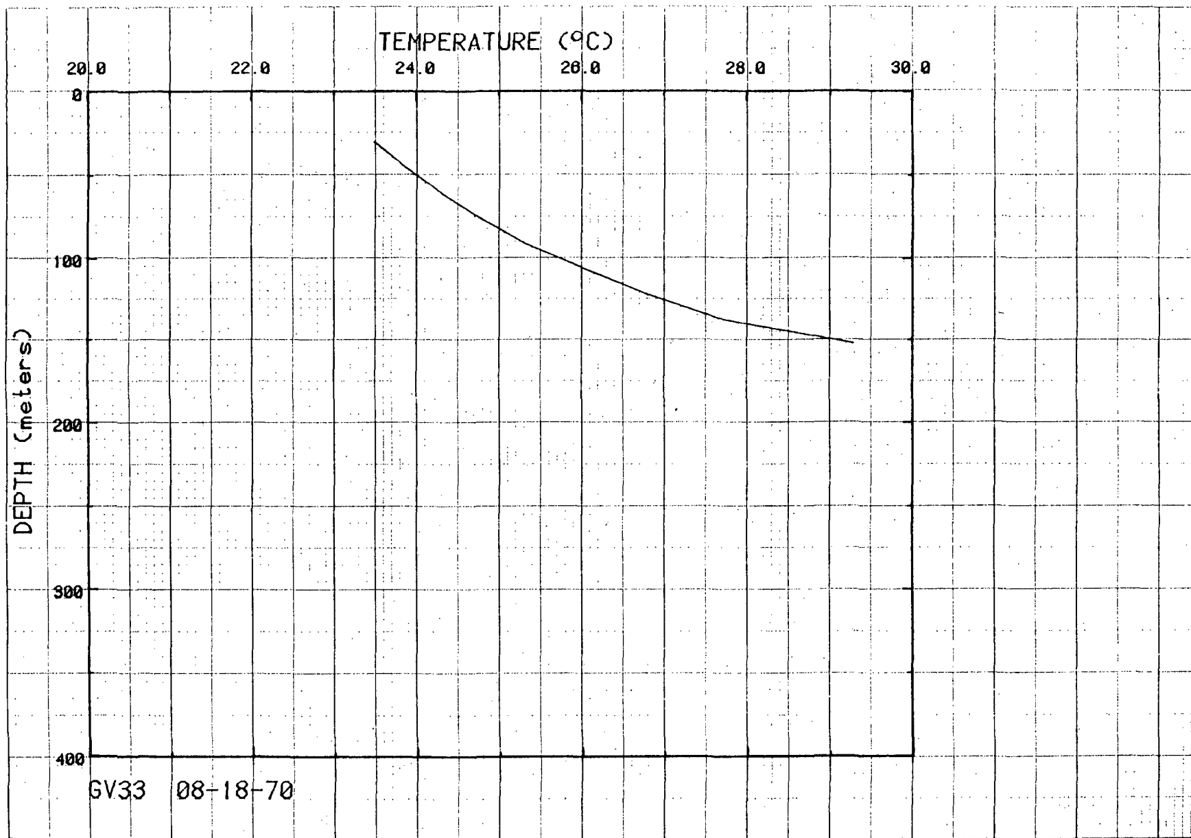
Figure 40. Temperatures for hole GV33.
