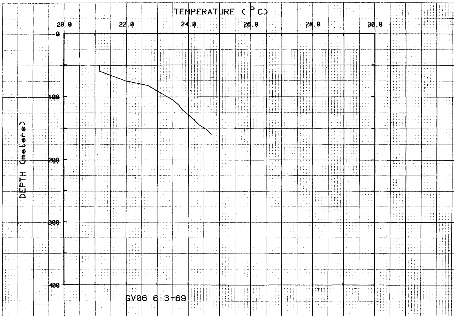
Figure 15. Temperatures for hole GV06.
