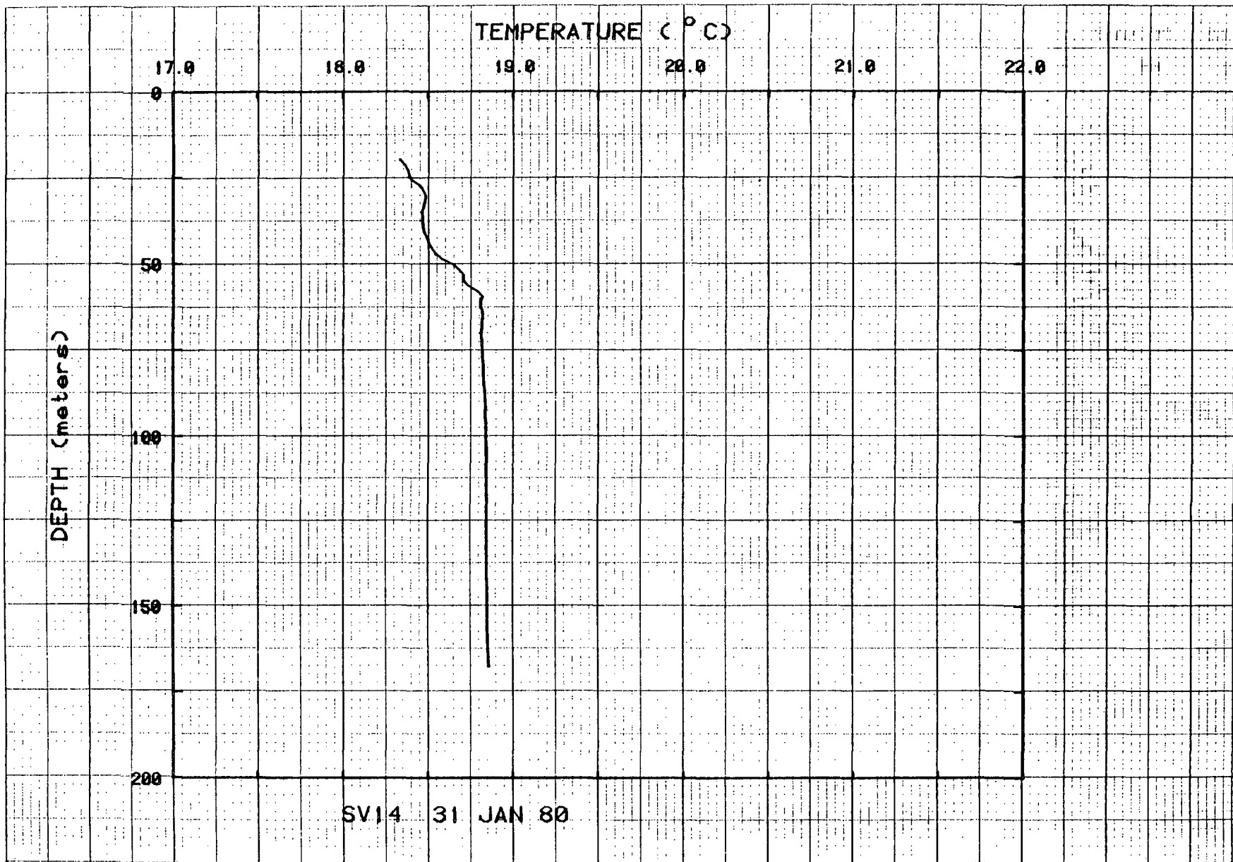
Figure 65. Temperatures for hole SV14.
