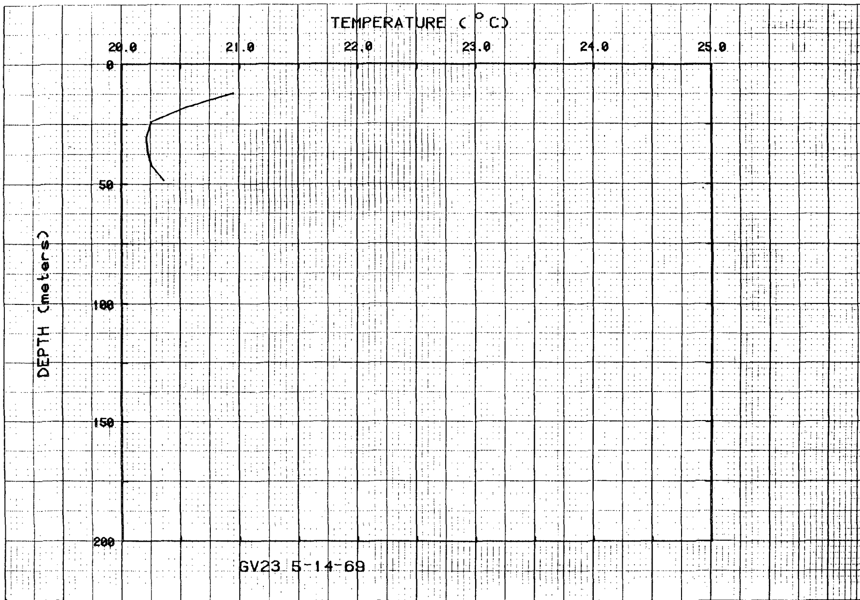
Figure 31. Temperatures for hole GV23.
