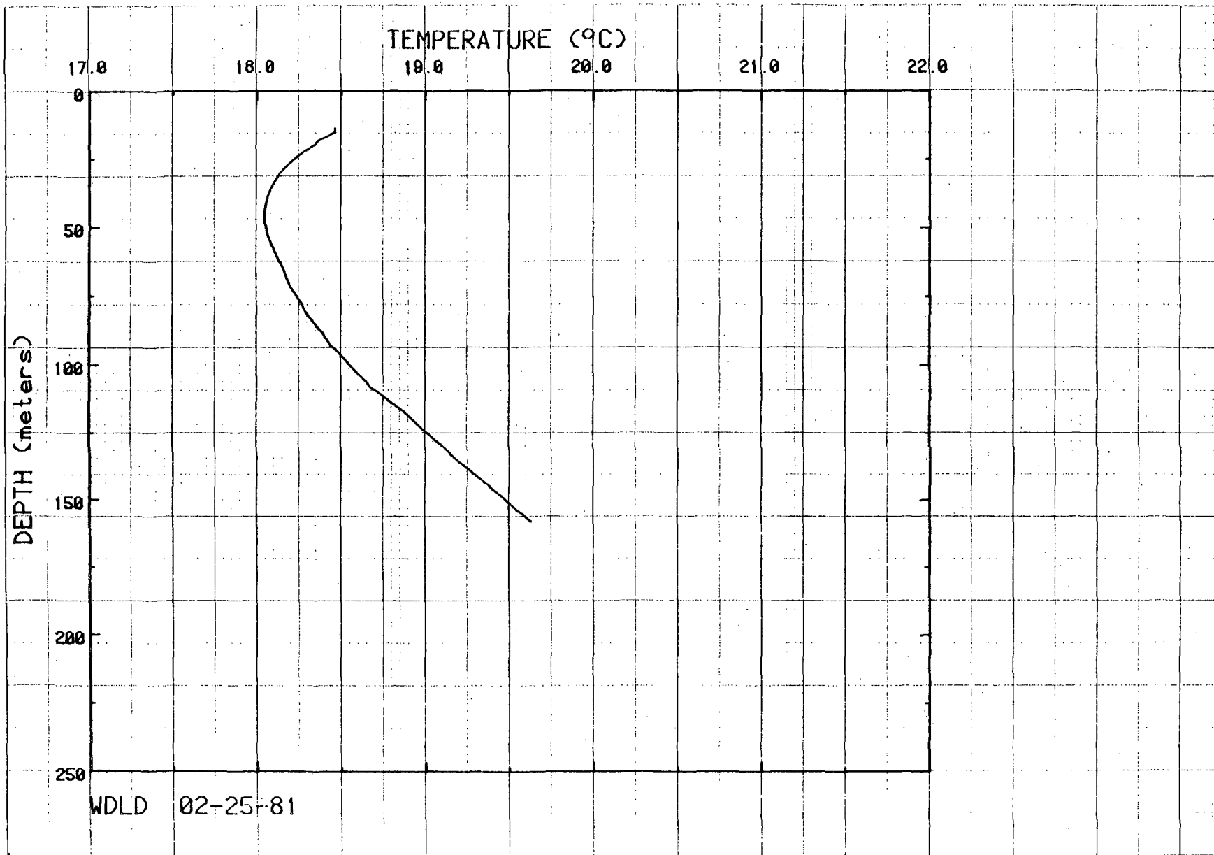
Figure 61. Temperatures for hole WDL D.
