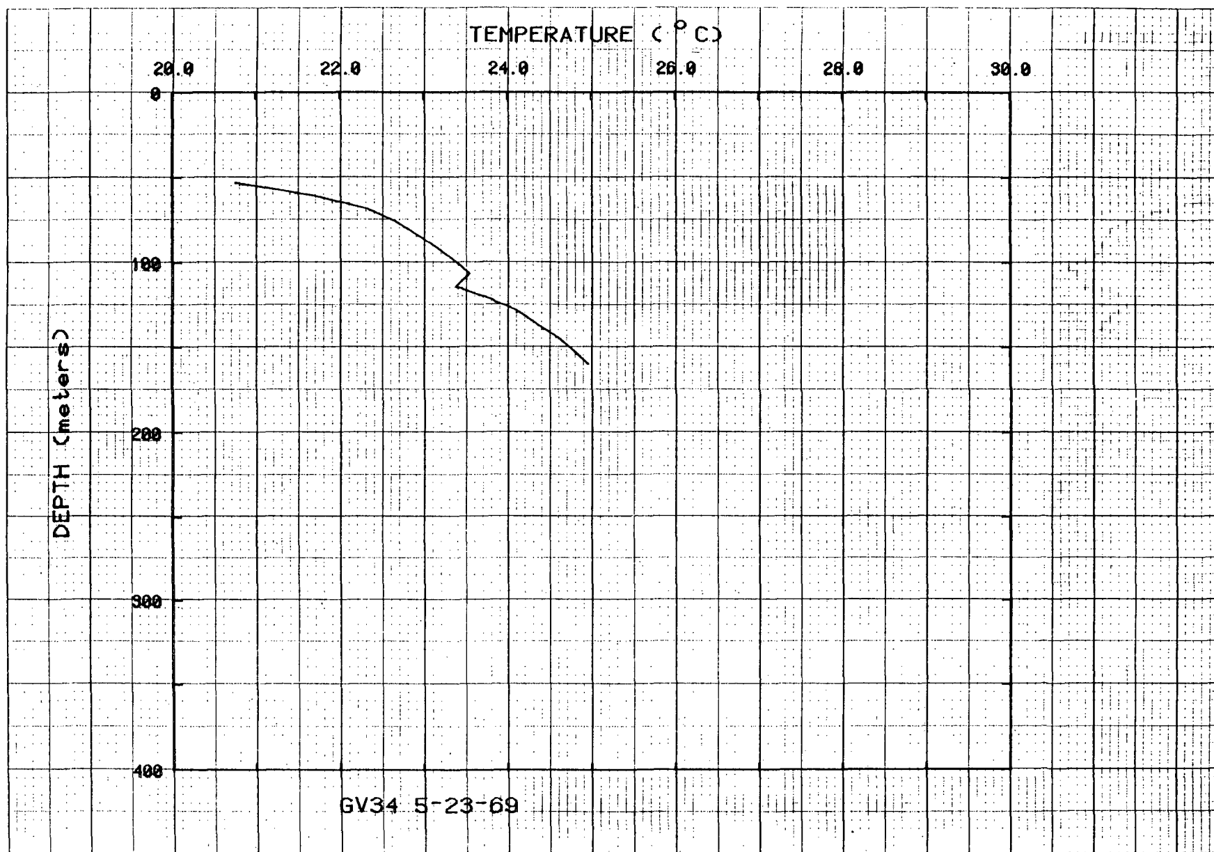
Figure 41. Temperatures for hole GV34.
