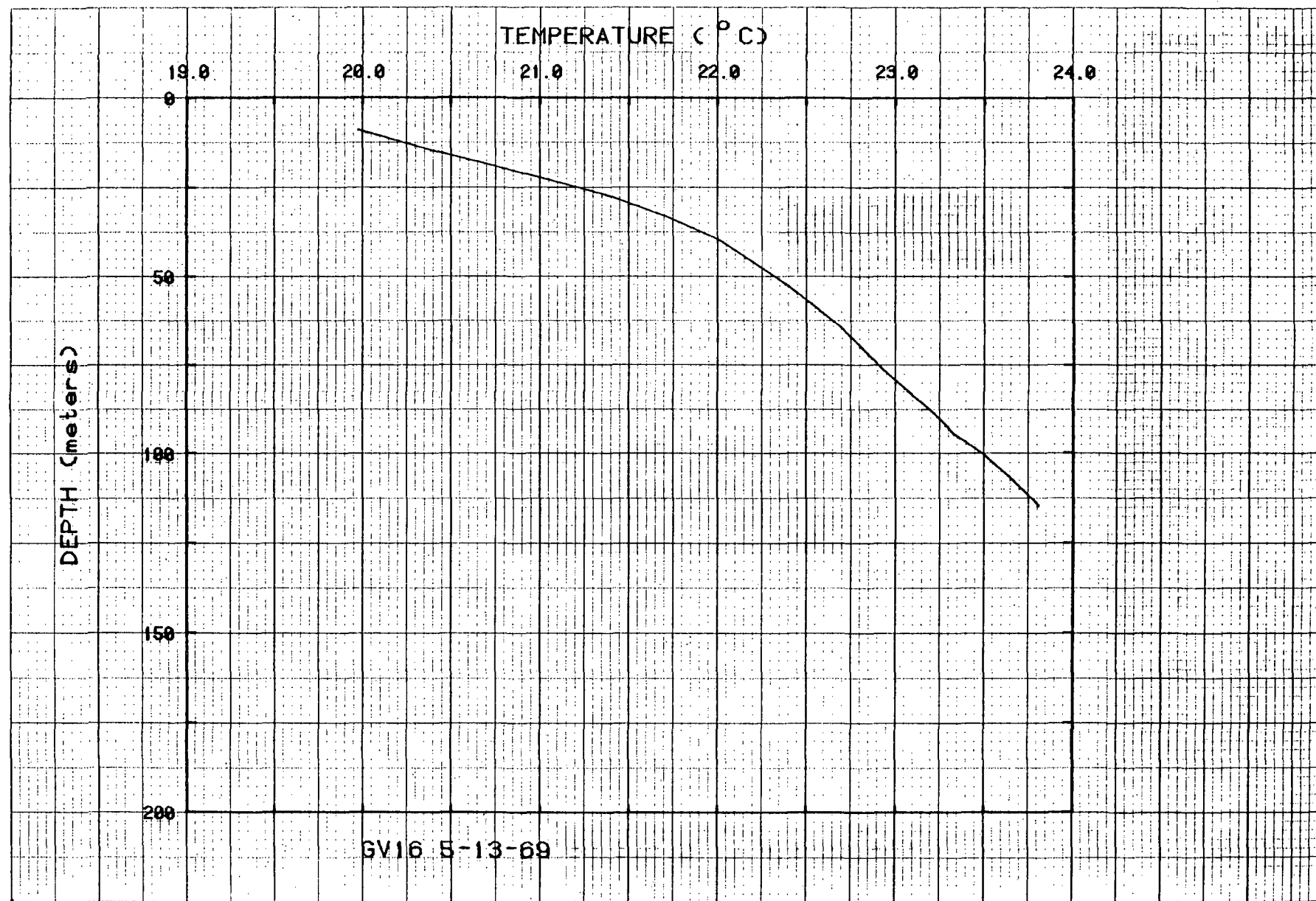
Figure 24. Temperatures for hole GV16.
