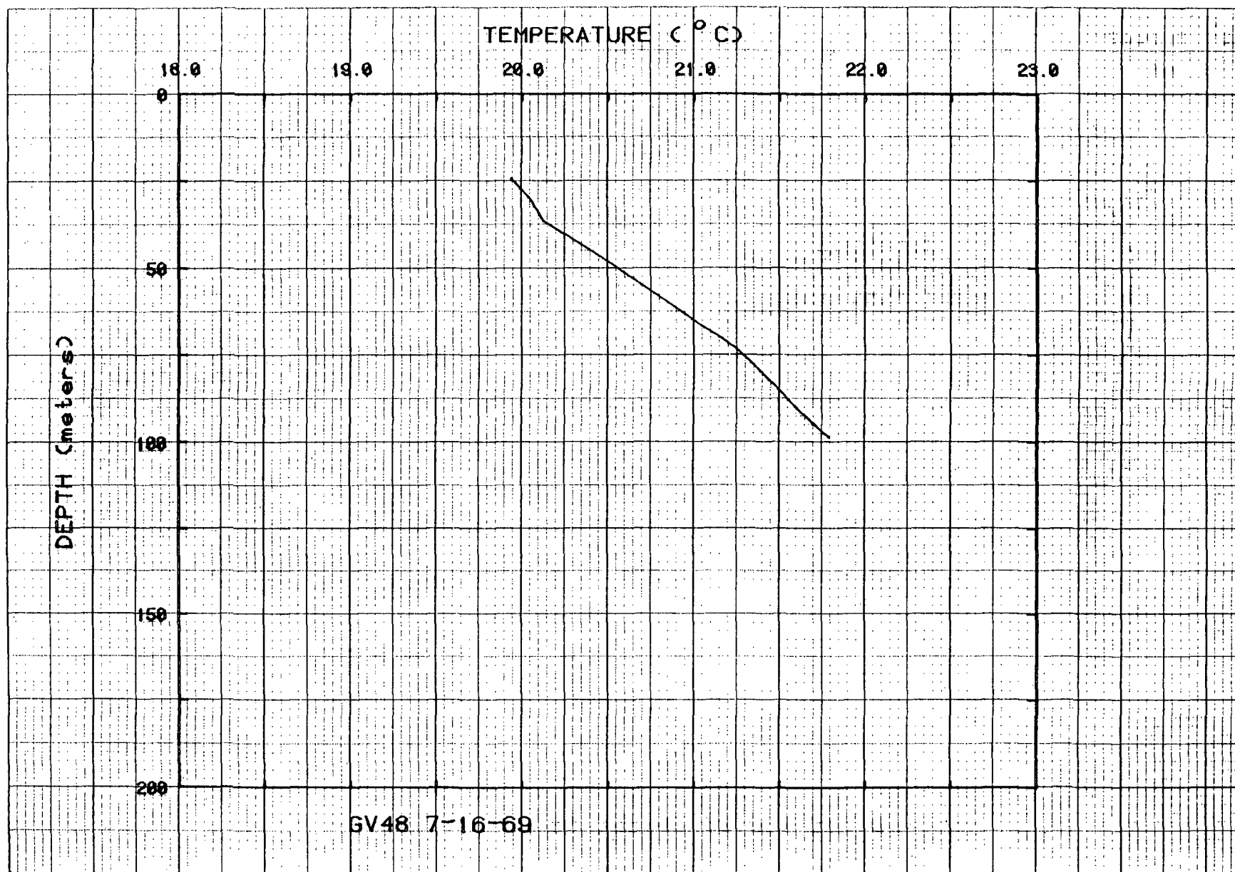
Figure 55. Temperatures for hole GV48.
