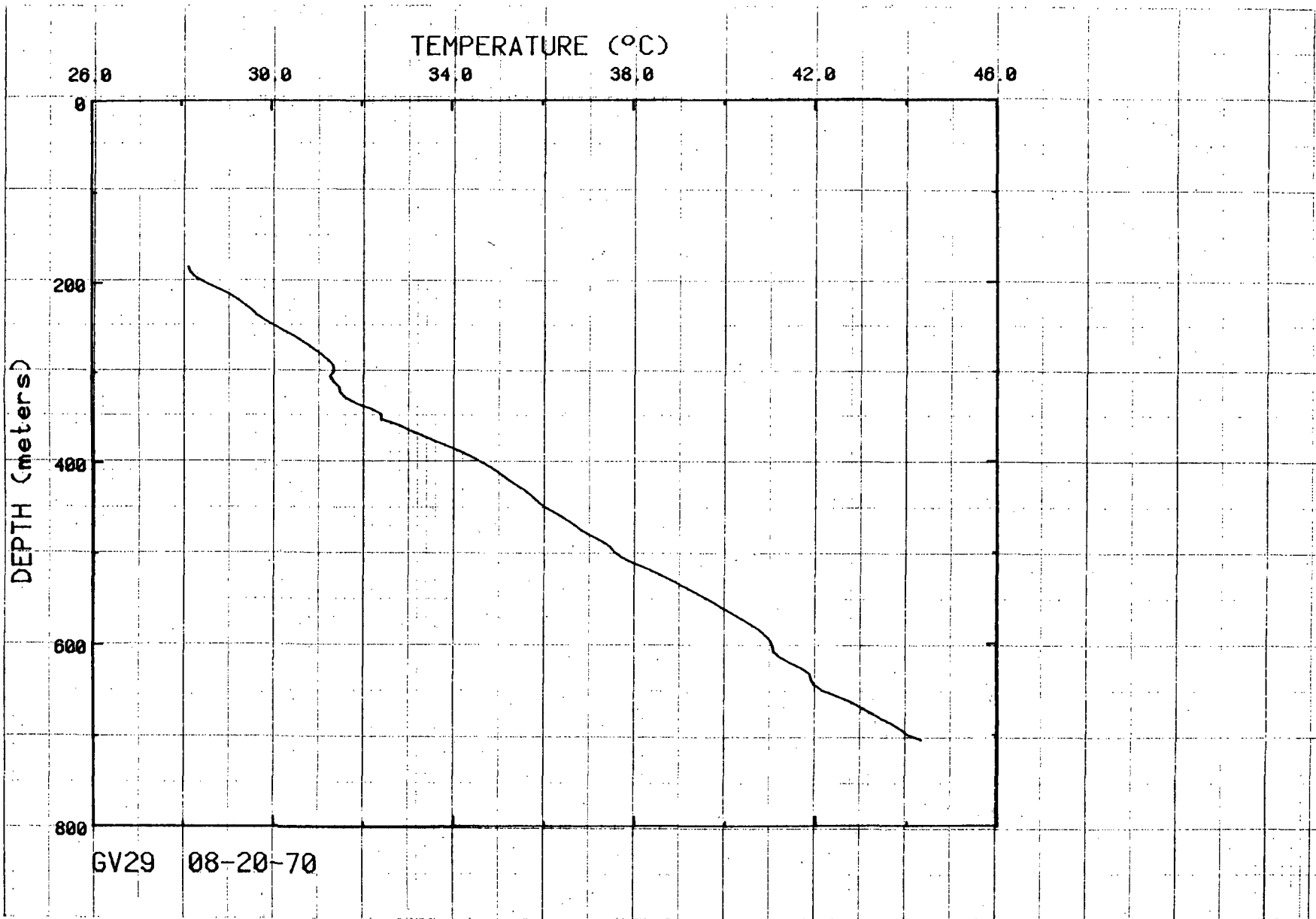
Figure 36. Temperatures for hole GV29.
