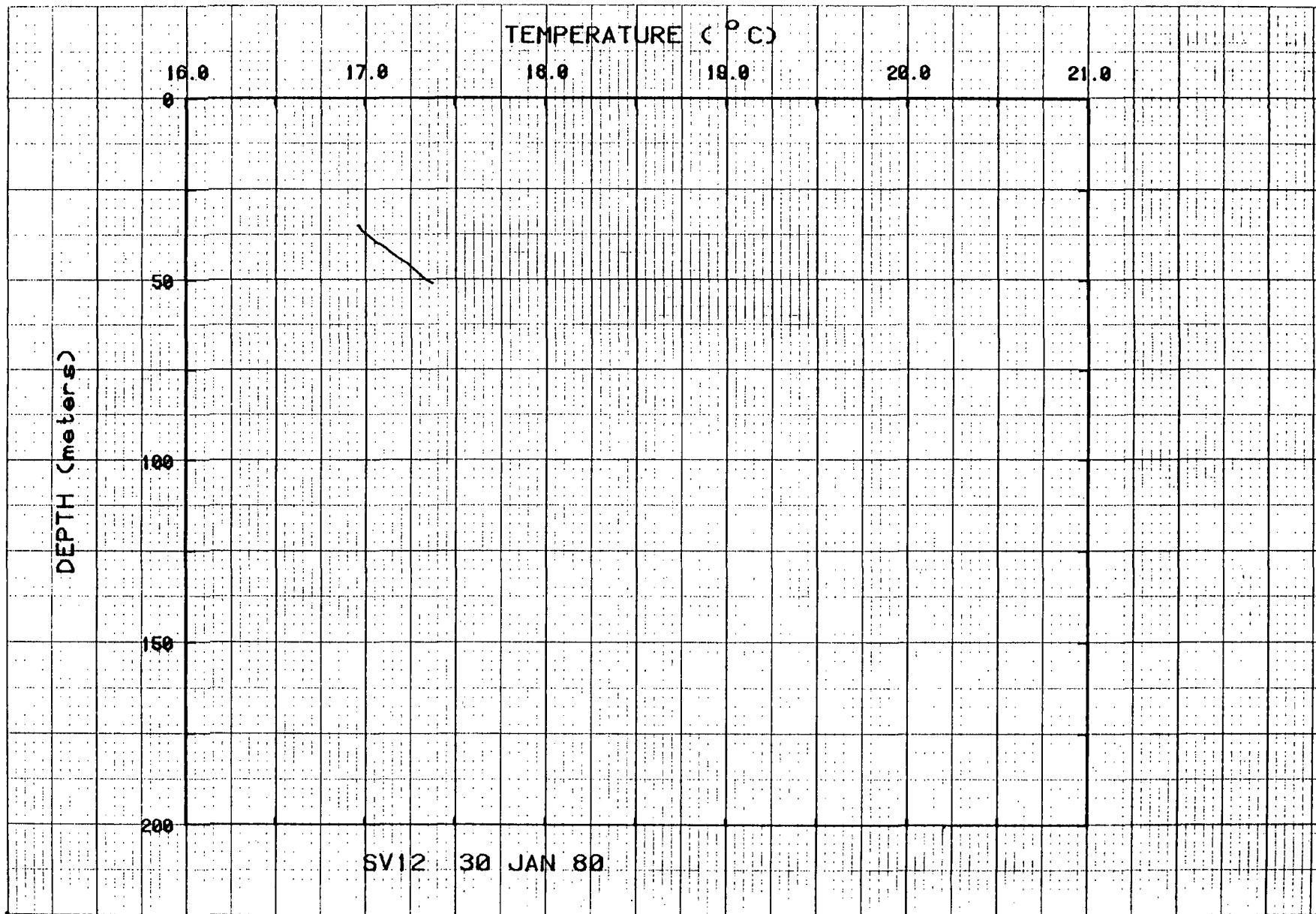
Figure 68. Temperatures for hole SV12.
