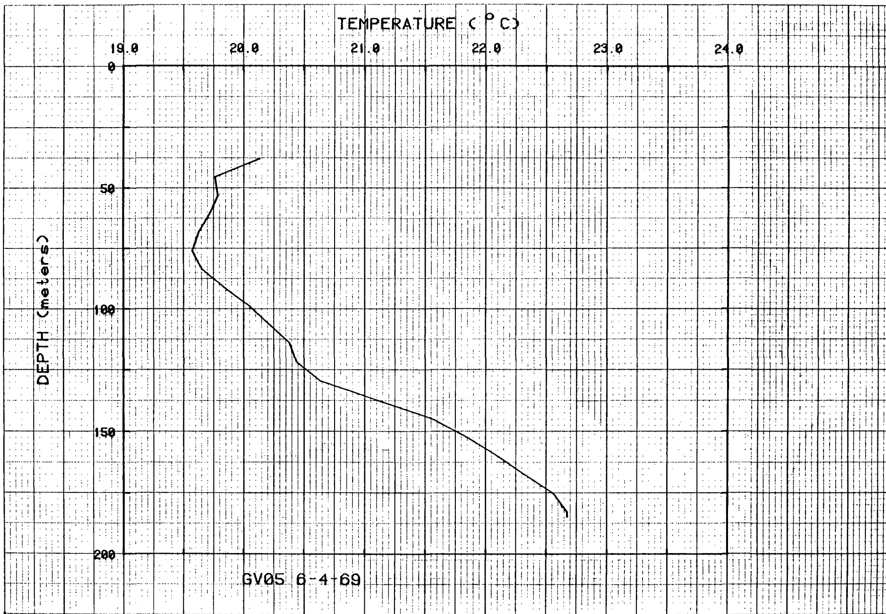
Figure 14. Temperatures for hole GV05.
