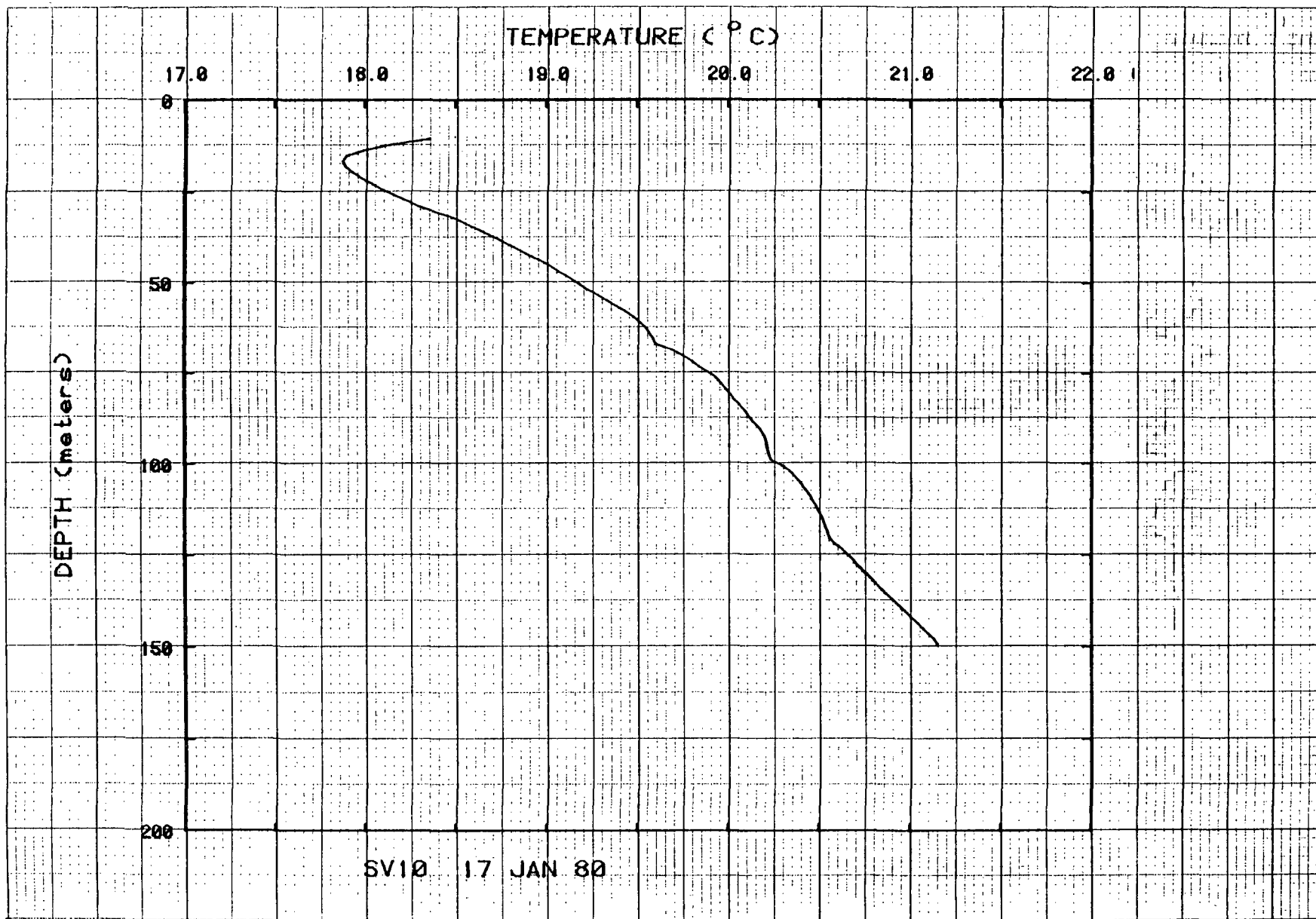
Figure 72. Temperatures for hole SV10.
