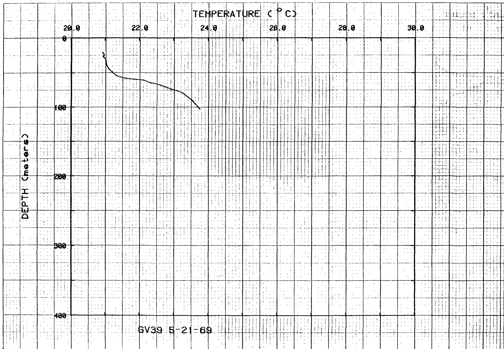
Figure 46. Temperatures for hole GV39.
