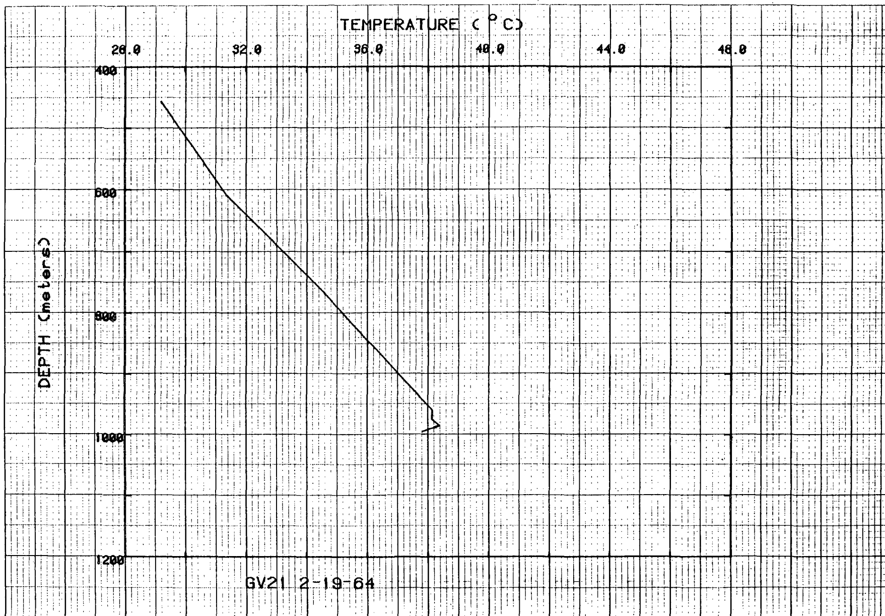
Figure 29. Temperatures for hole GV21.
