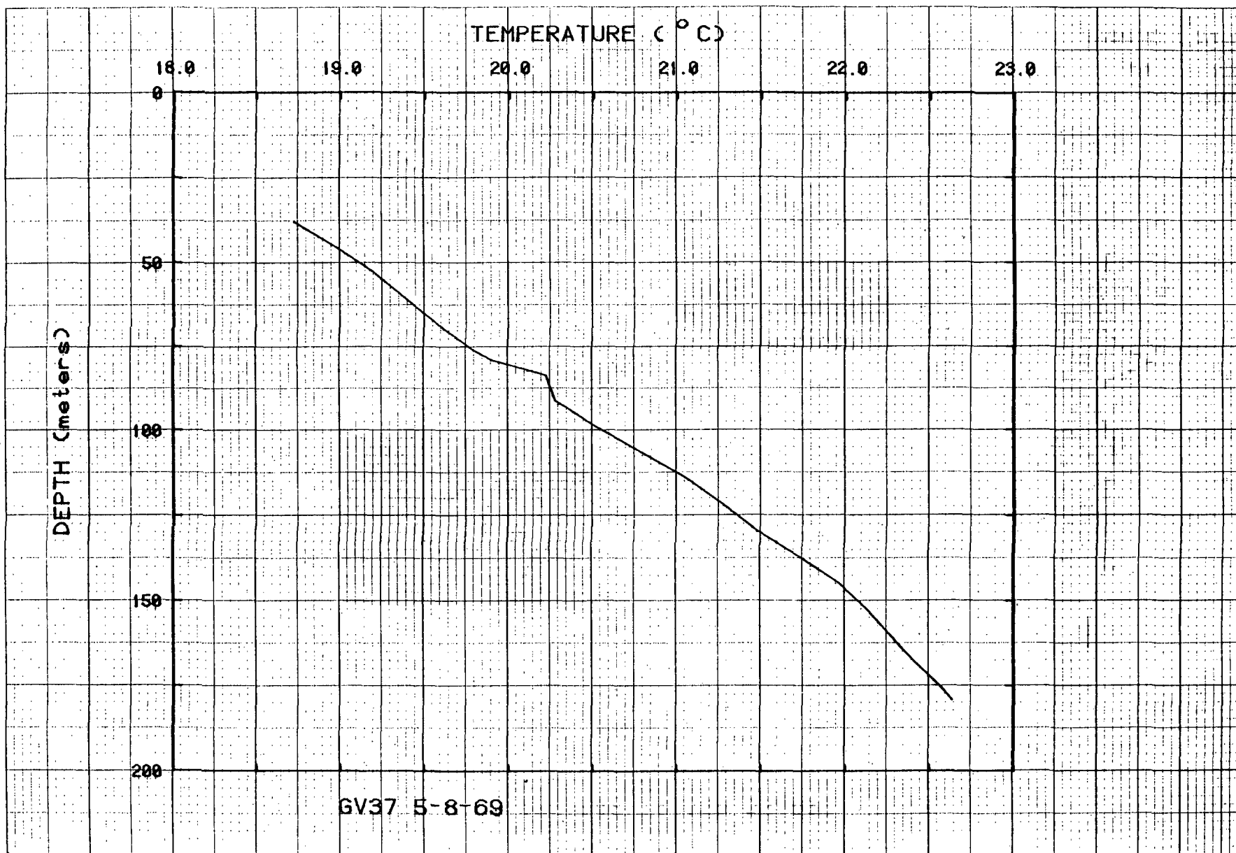
Figure 44. Temperatures for hole GV37.
