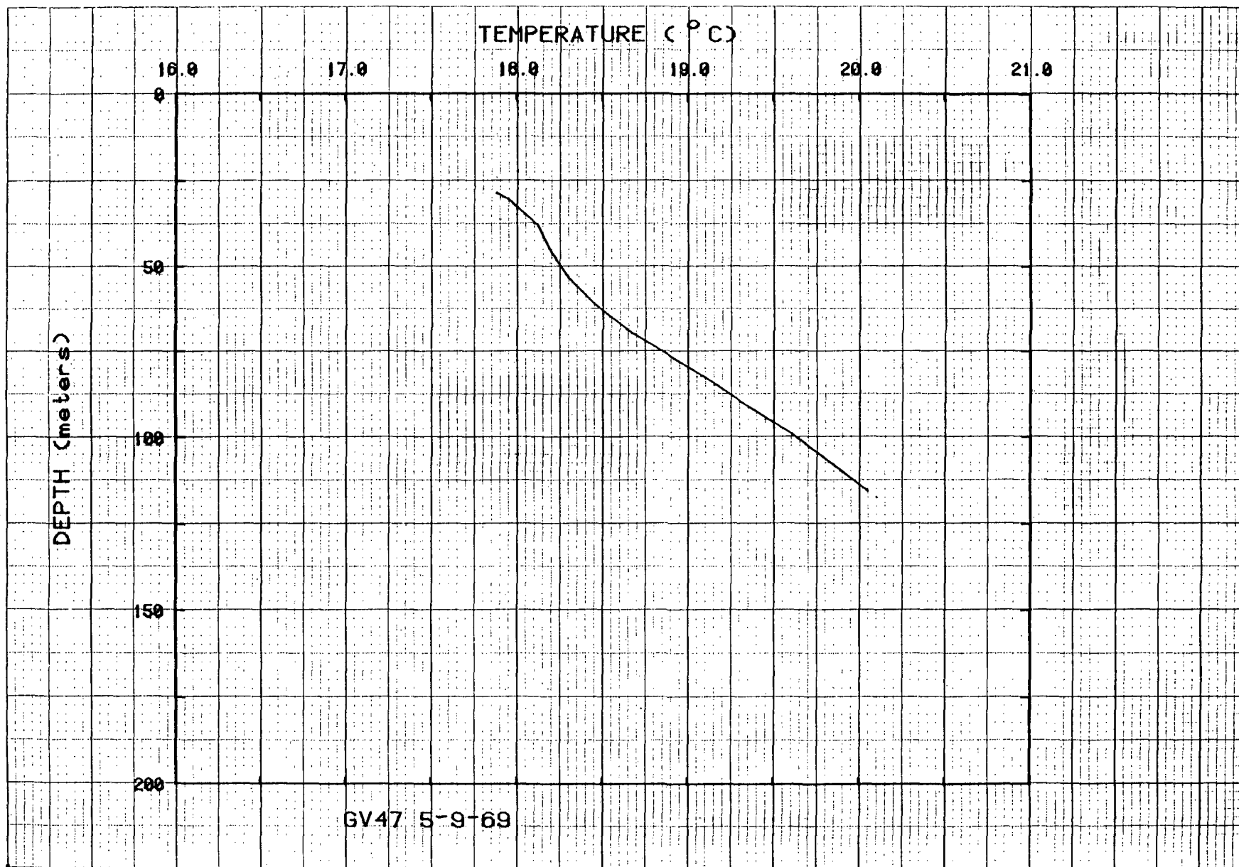
Figure 54. Temperatures for hole GV47.
