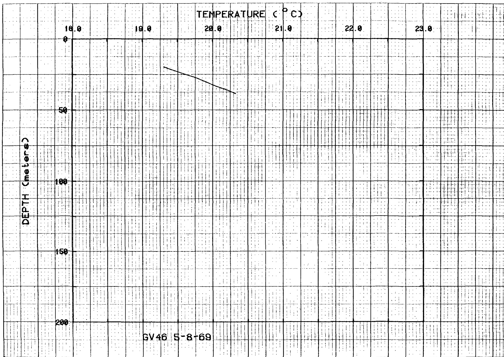
Figure 53. Temperatures for hole GV46.
