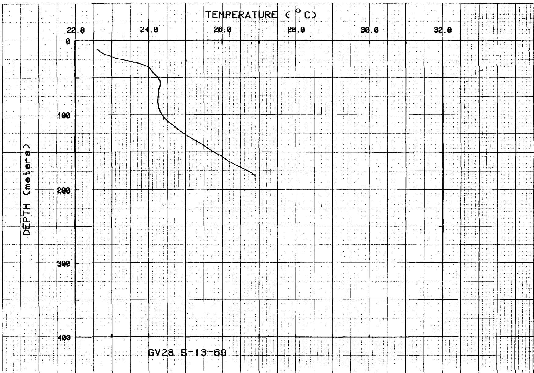
Figure 35. Temperatures for hole GV28.
