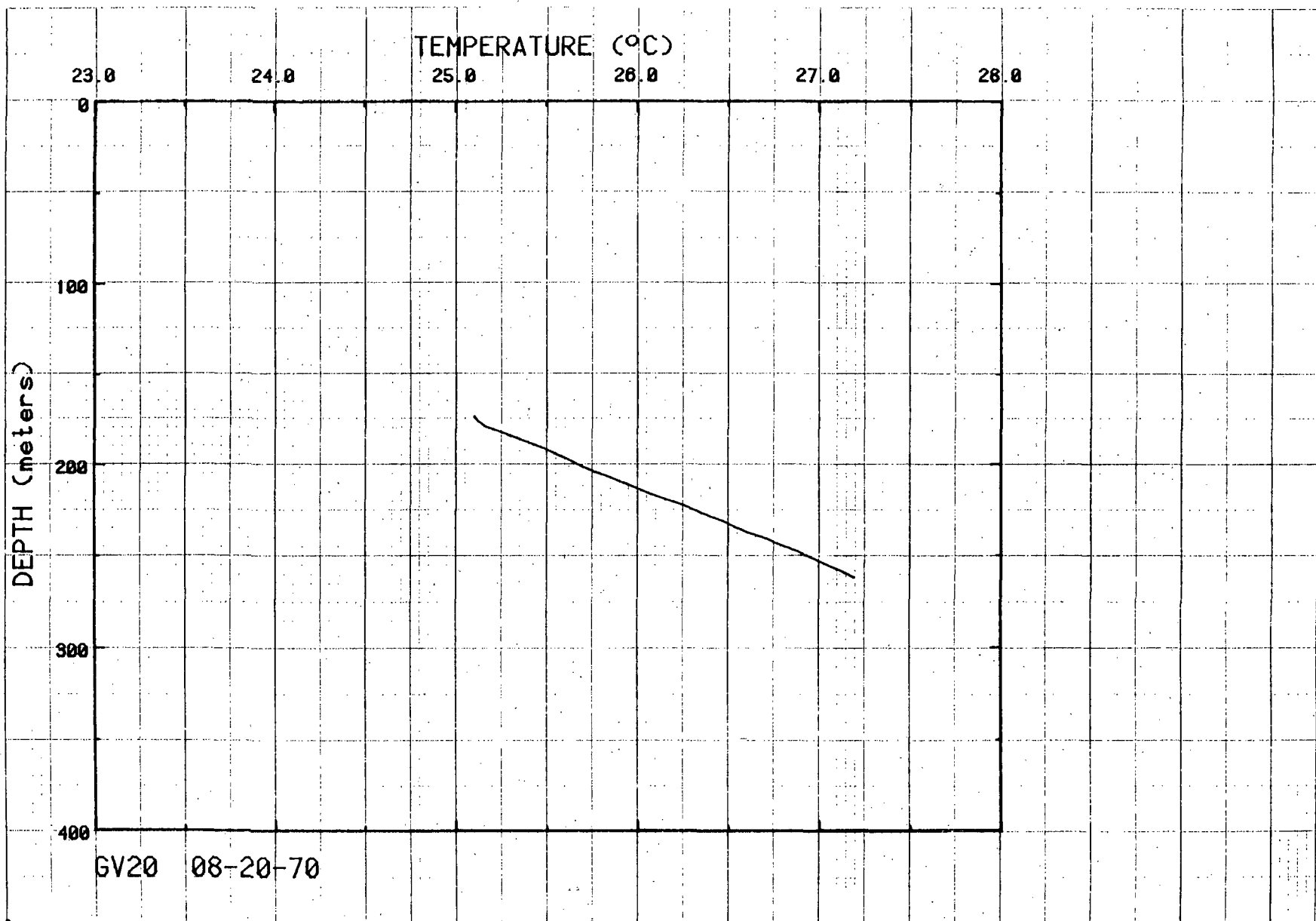
Figure 28. Temperatures for hole GV20.
