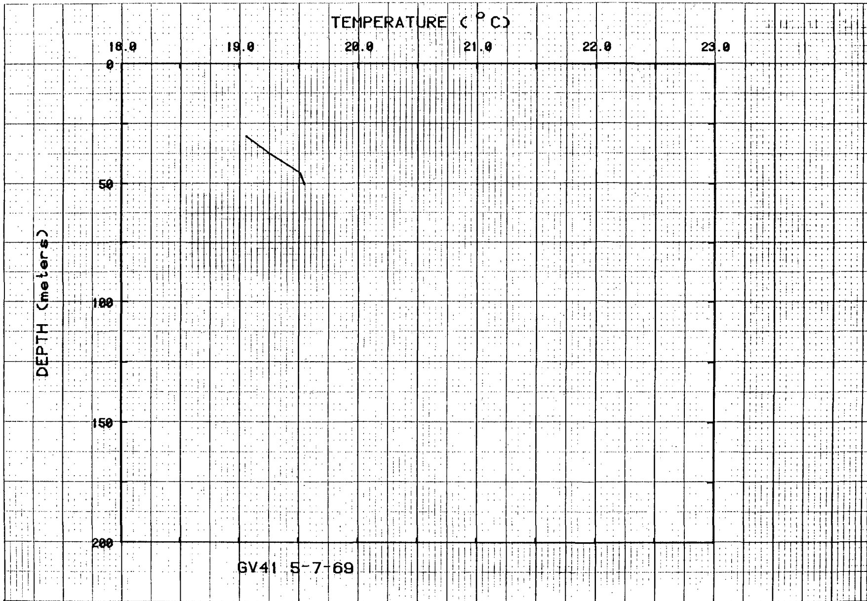
Figure 48. Temperatures in hole GV41.
