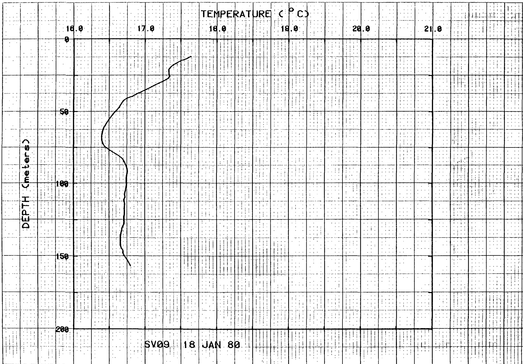
Figure 70. Temperatures for hole SV09.
