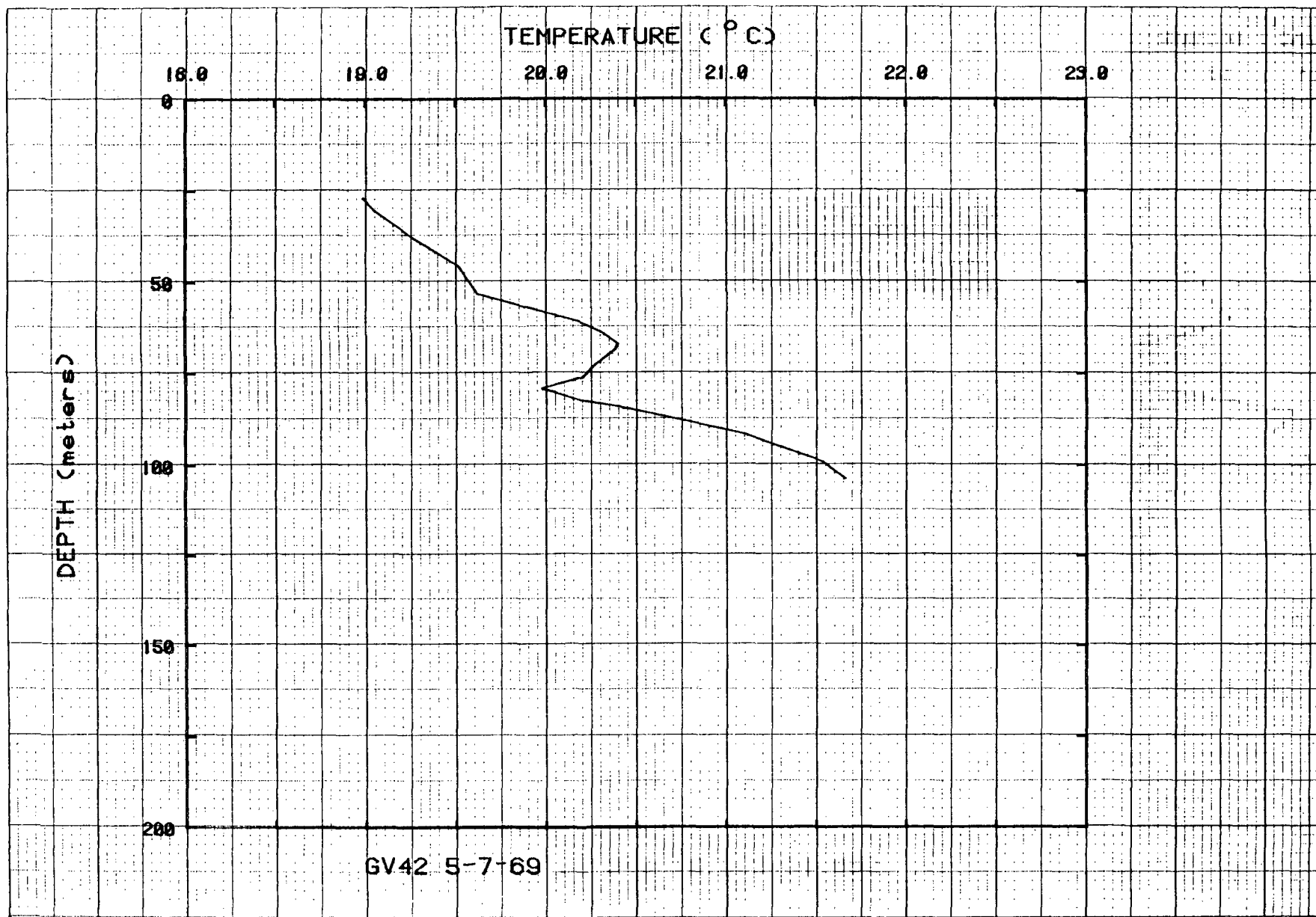
Figure 49. Temperatures for hole GV42.
