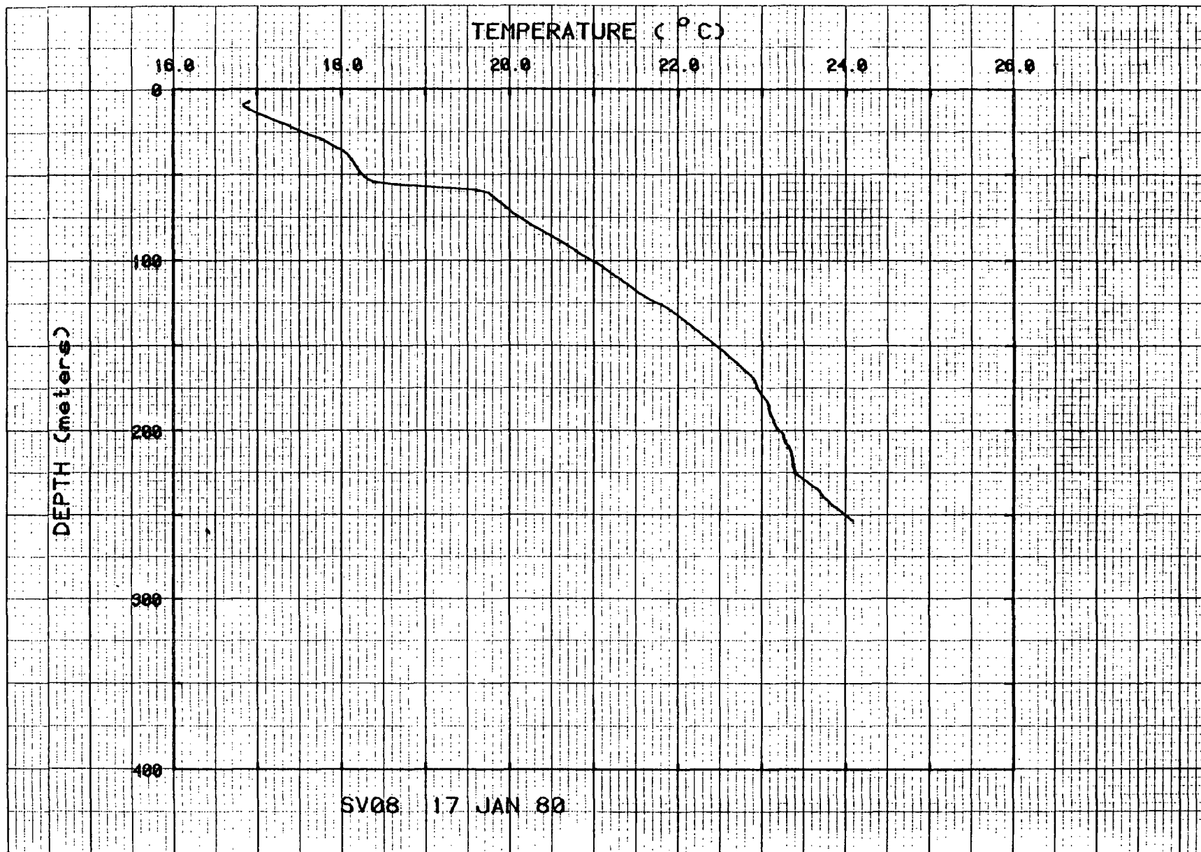
Figure 73. Temperatures for hole SV08.
