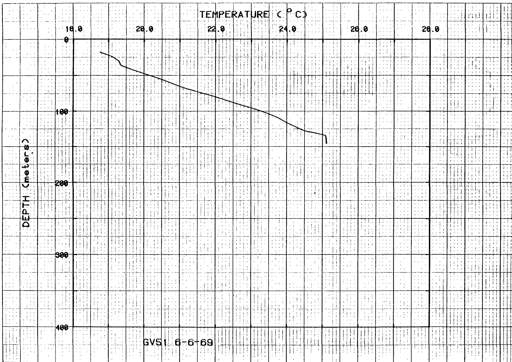
Figure 58. Temperatures for hole GV51.
