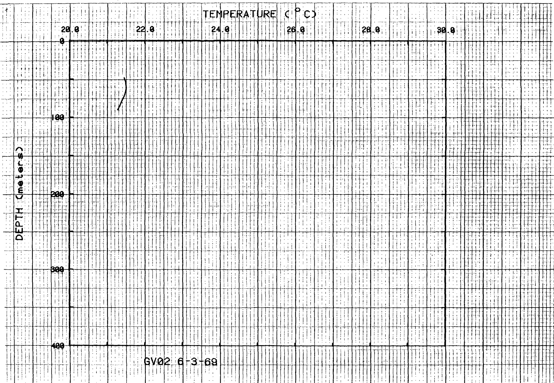
Figure 11. Temperatures for hole GV02.
