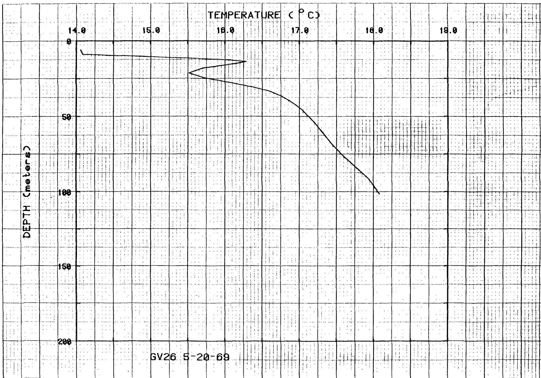
Figure 33. Temperatures for hole GV26.
