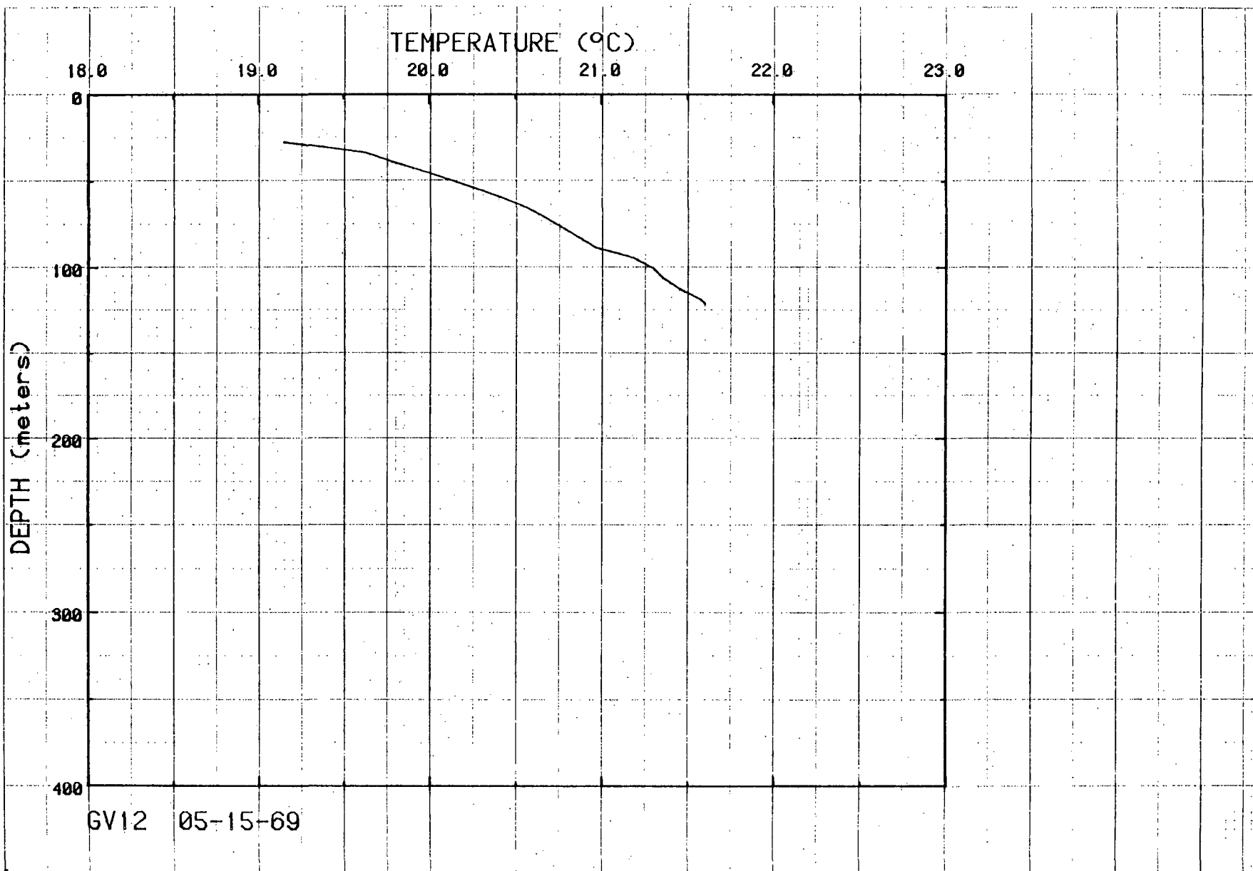
Figure 20. Temperatures for hole GV12.
