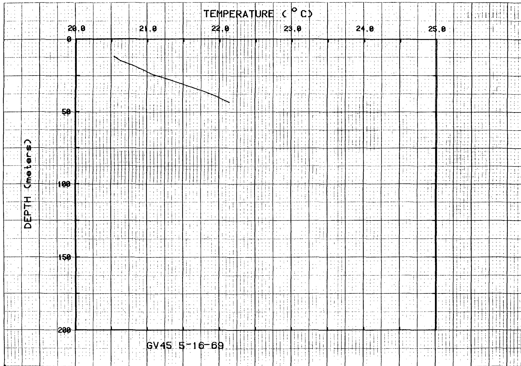
Figure 52. Temperatures for hole GV45.
