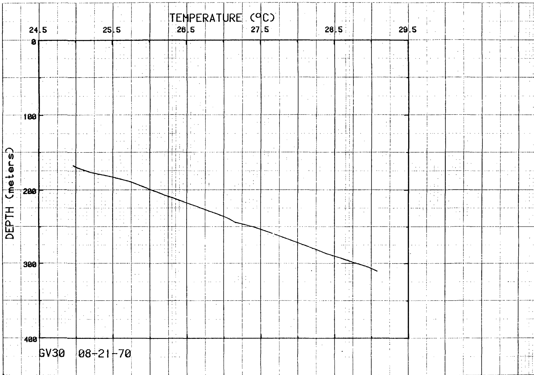
Figure 37. Temperatures for hole GV30.
