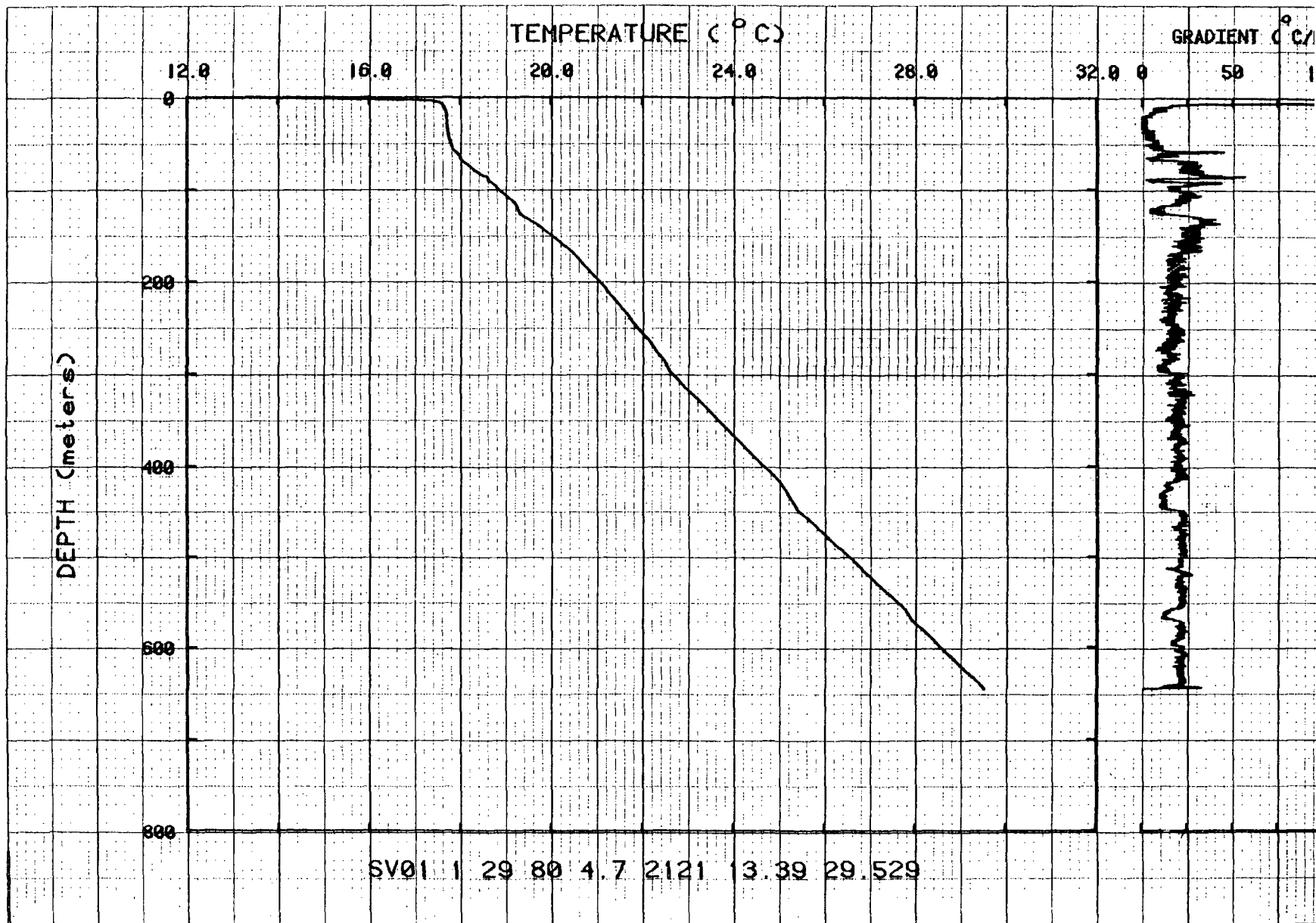
Figure 3. Temperatures and gradients for hole SV01.
