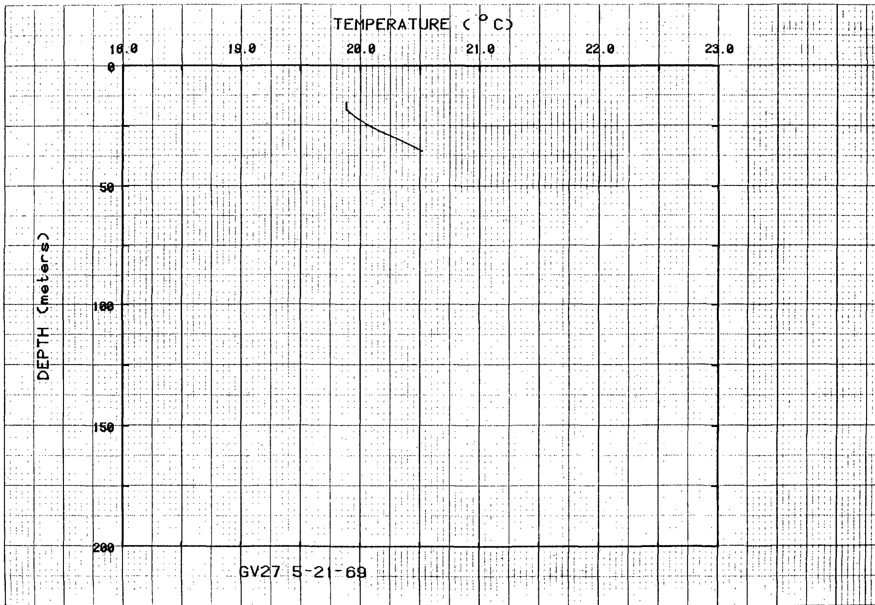
Figure 34. Temperatures for hole GV27.
