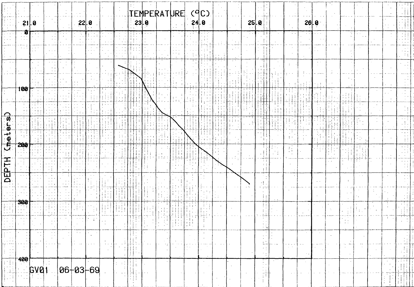
Figure 10. Temperatures for hole GV01.
