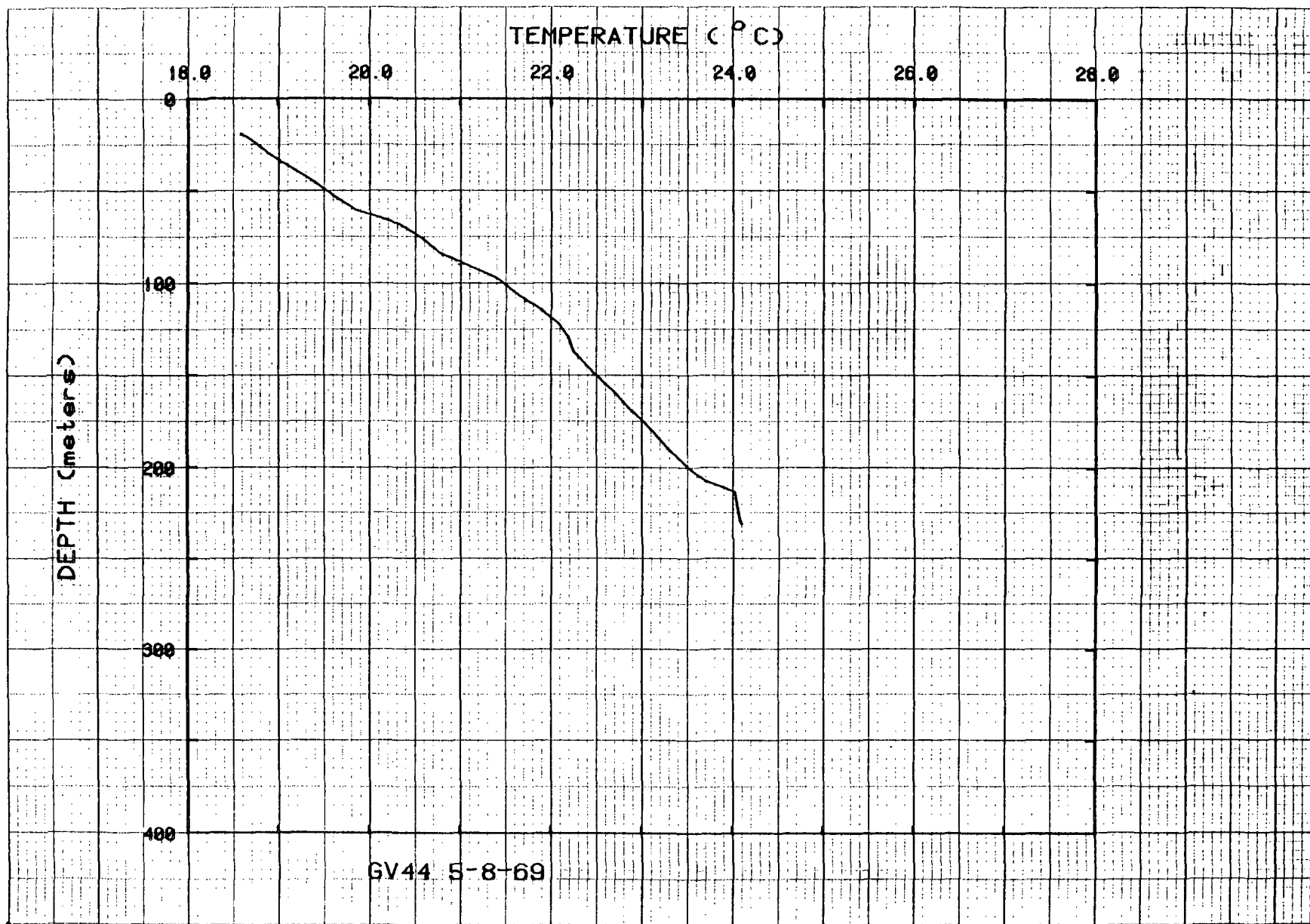
Figure 51. Temperatures for hole GV44.
