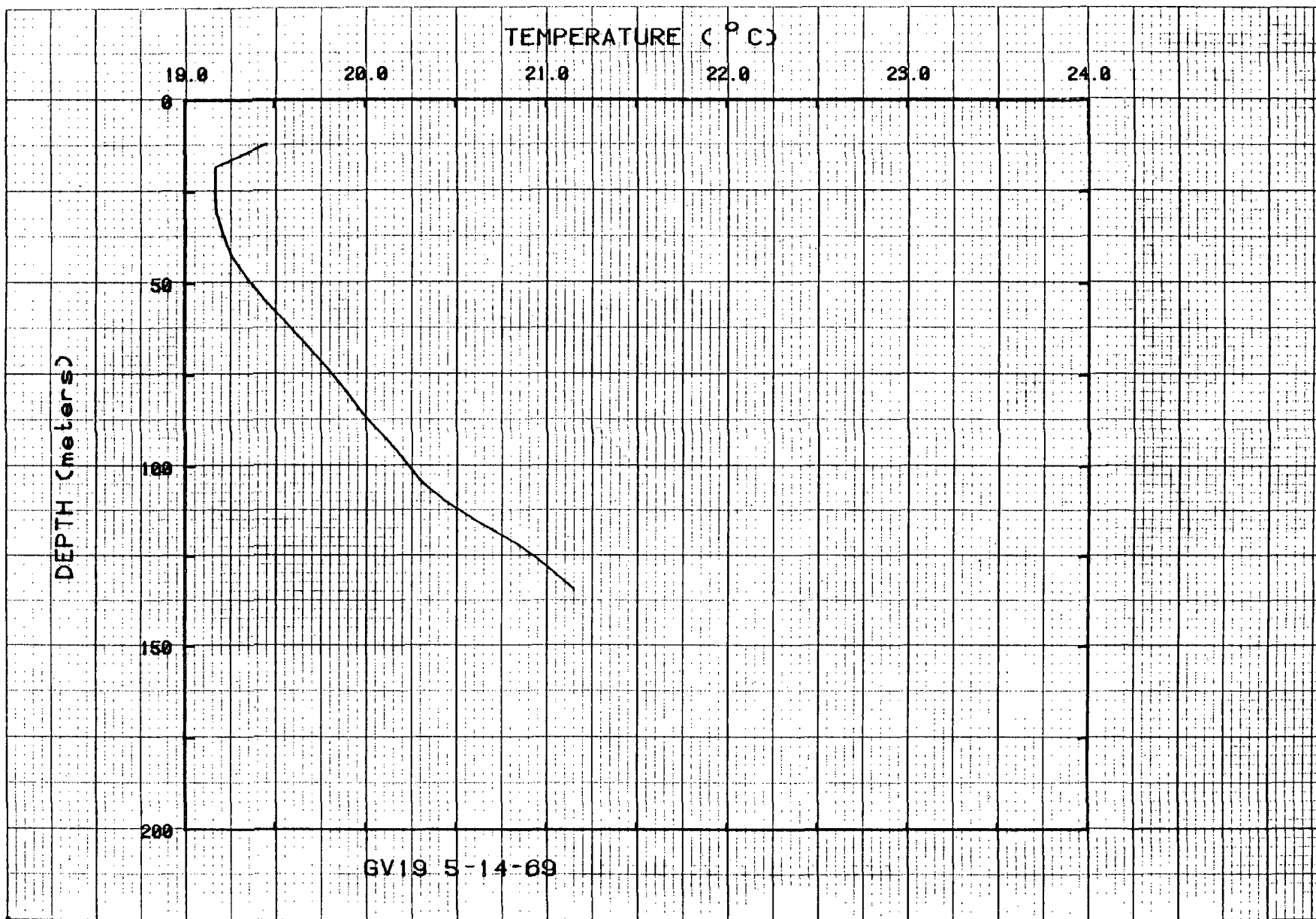
Figure 27. Temperatures for hole GV19.
