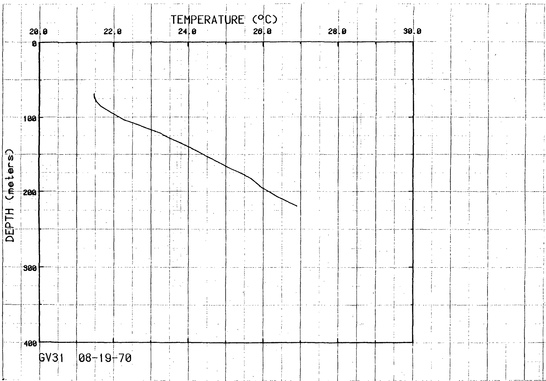
Figure 38. Temperatures for hole GV31.
