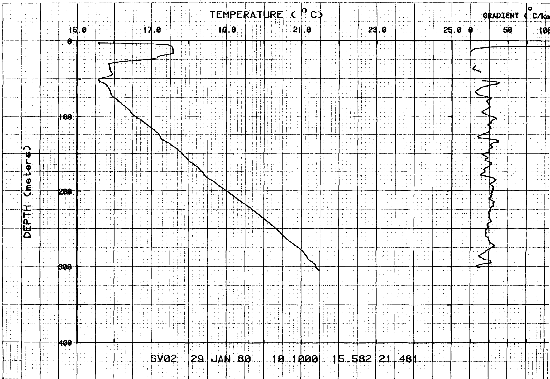
Figure 4. Temperatures and gradients for hole SV02.
