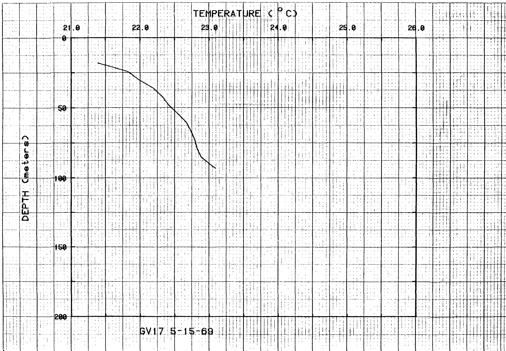
Figure 25. Temperatures for hole GV17.
