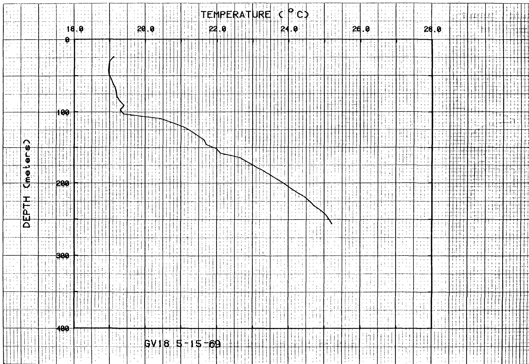
Figure 26. Temperatures for hole GV18.
