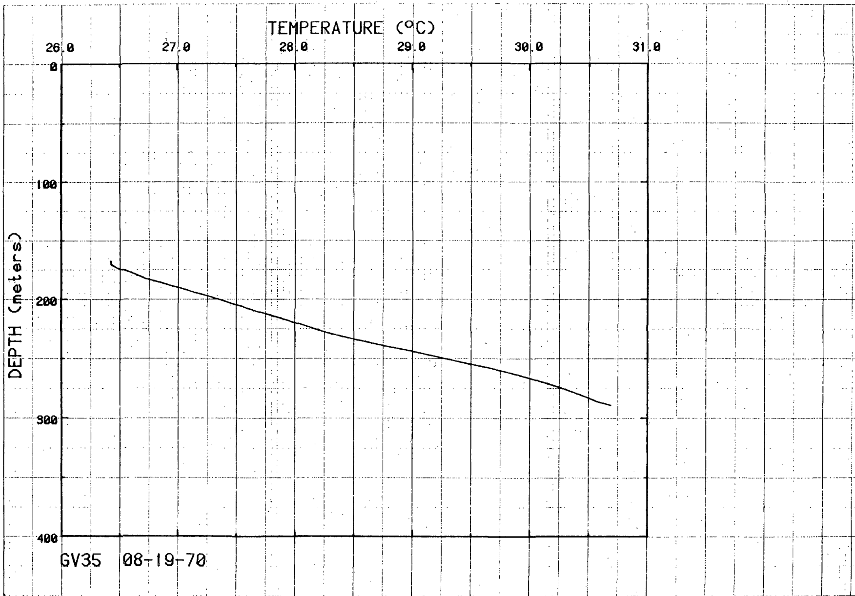
Figure 42. Temperatures for hole GV35.
