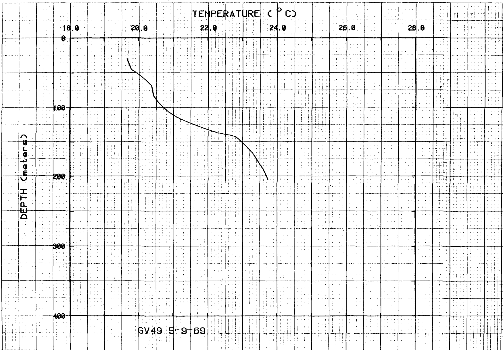
Figure 56. Temperatures for hole GV49.
