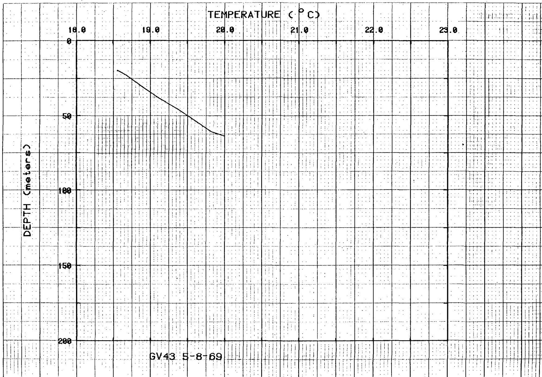
Figure 50. Temperatures for hole GV43.
