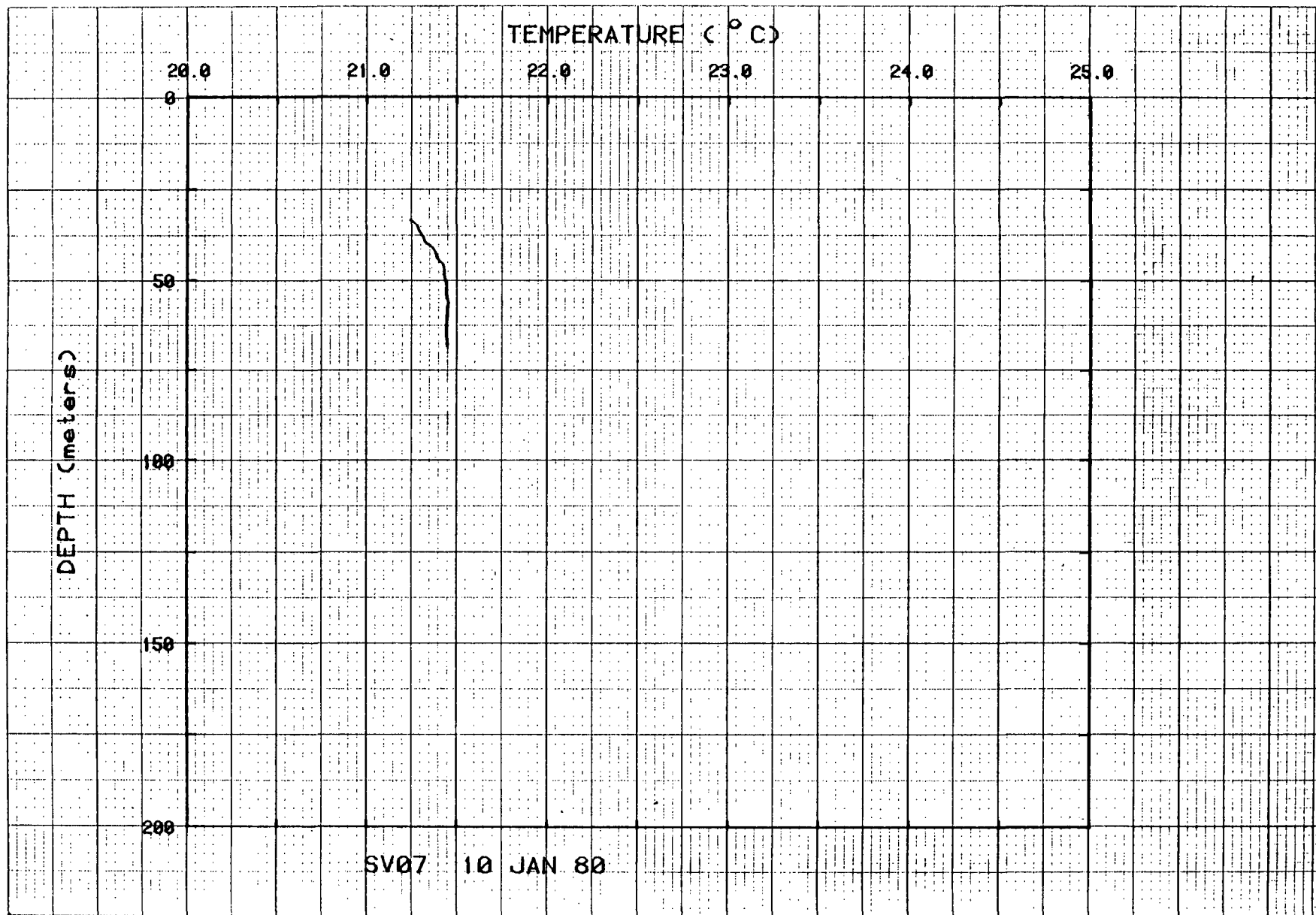
Figure 66. Temperatures for hole SV07.
