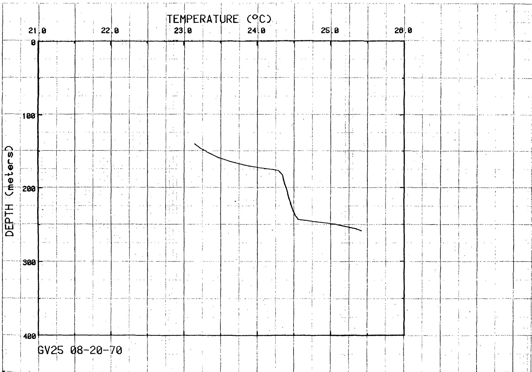
Figure 32. Temperatures for hole GV25.
