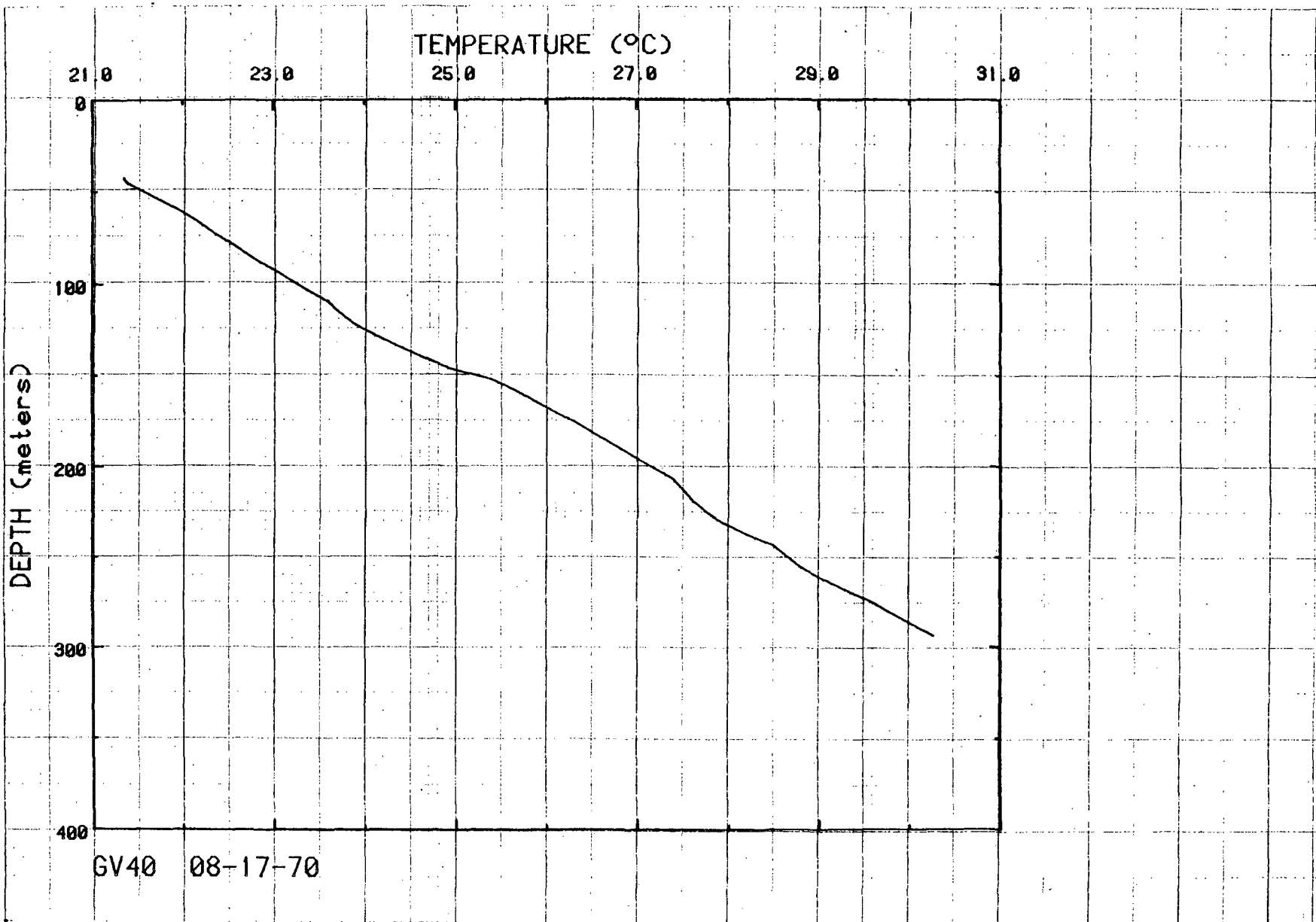
Figure 47. Temperatures for hole GV40.
