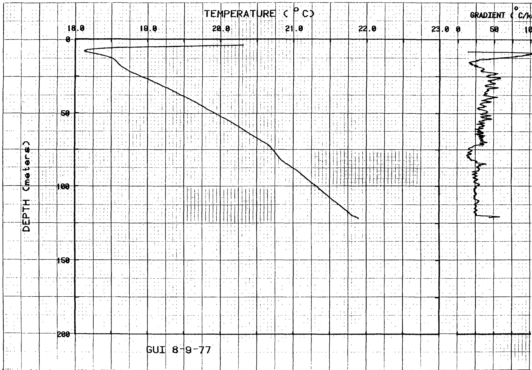
Figure 62. Temperatures and gradients for hole GUI.
