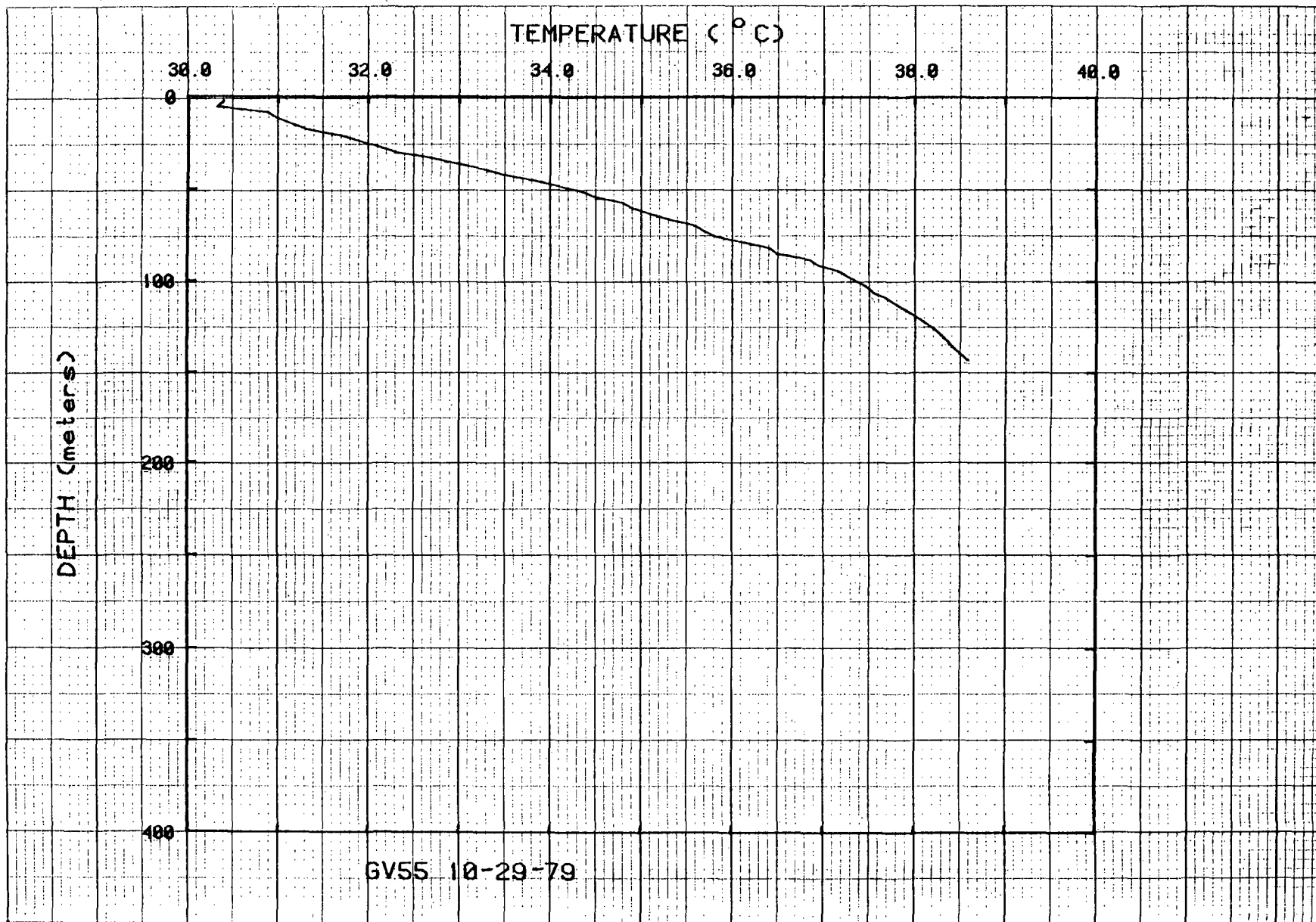
Figure 60. Temperatures for hole GV55.
