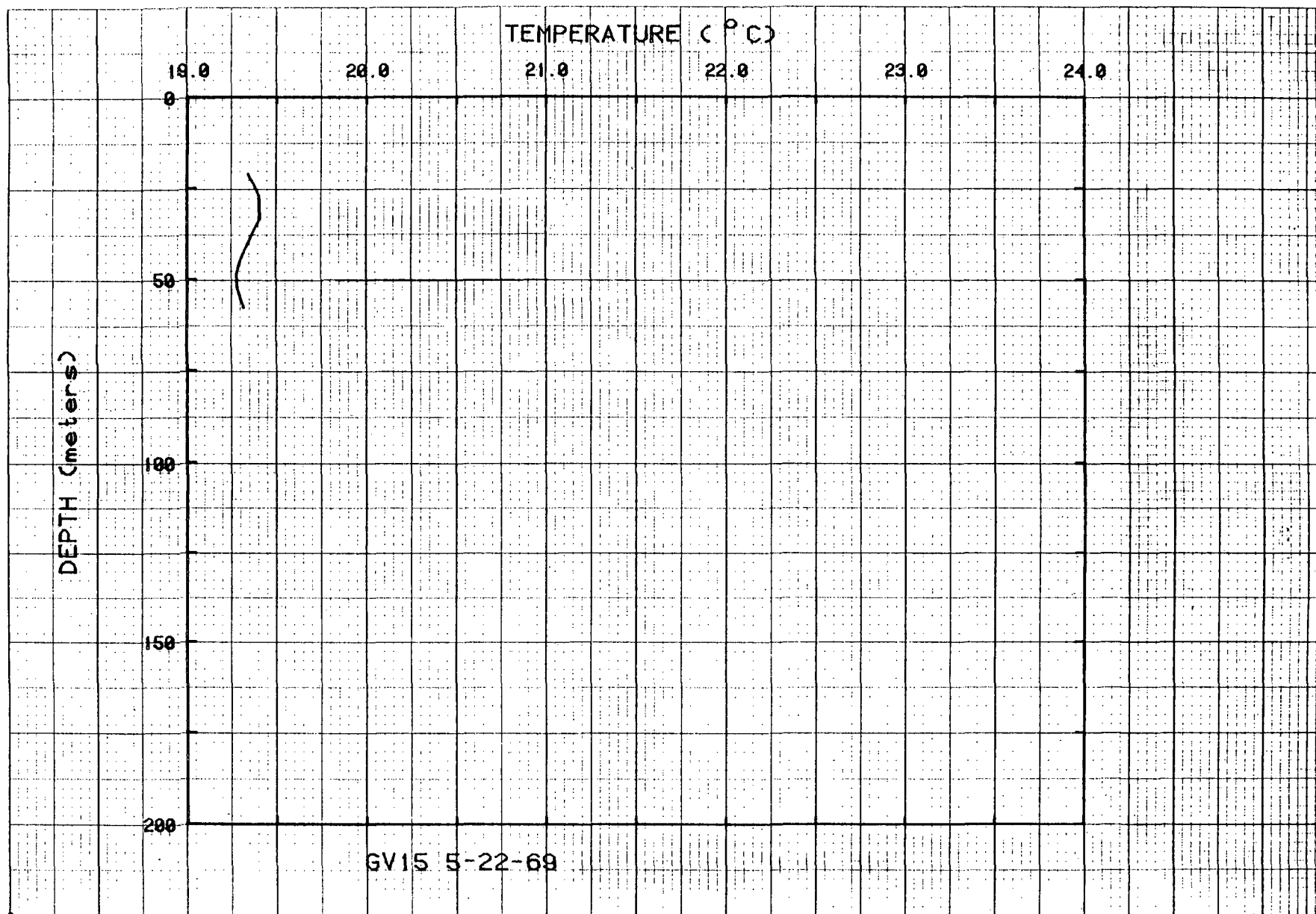
Figure 23. Temperatures for hole GV15.
