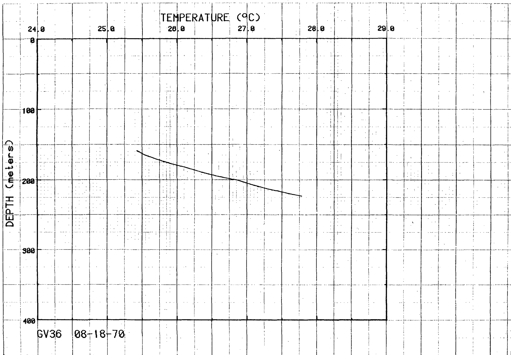
Figure 43. Temperatures for hole GV36.
