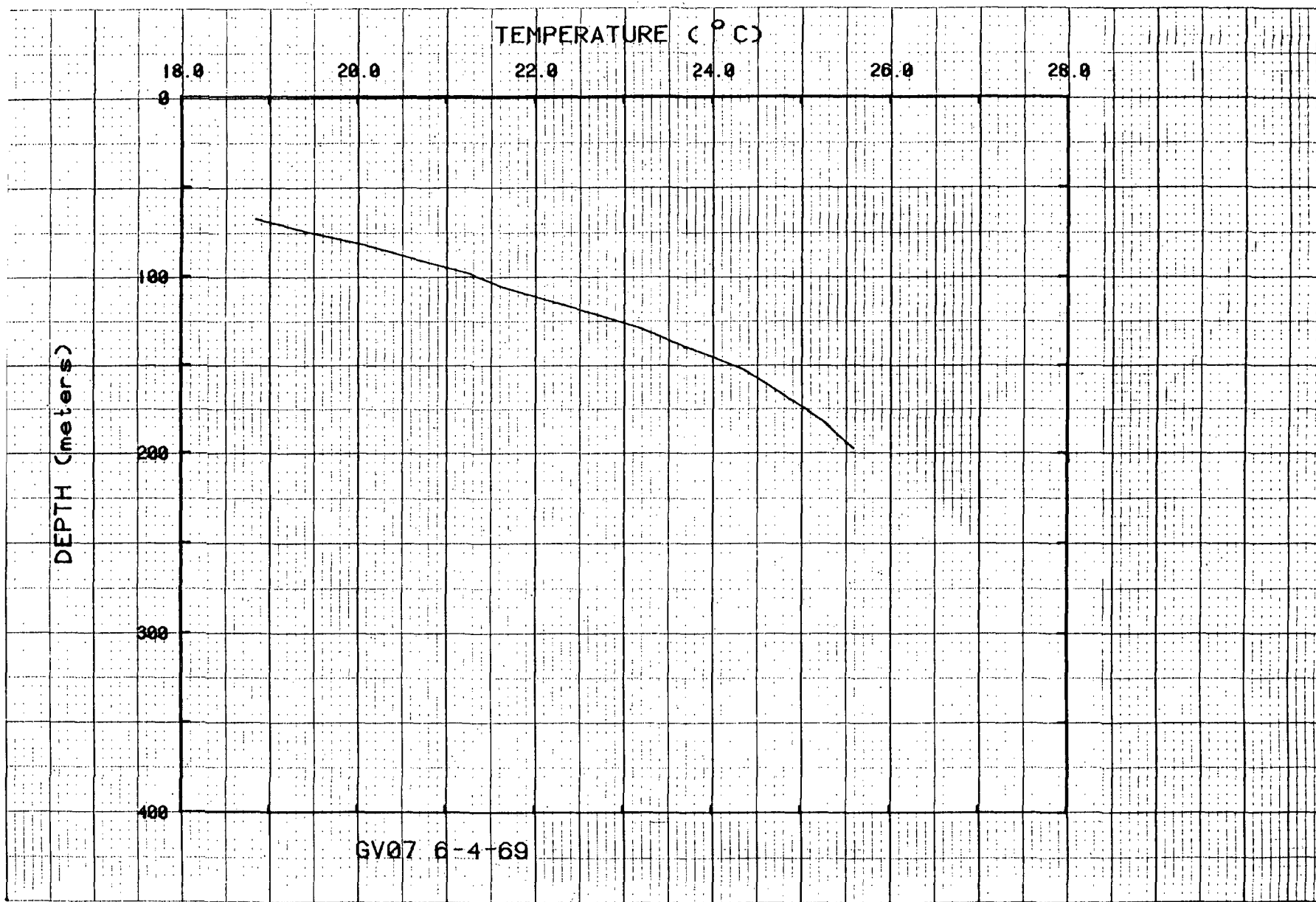
Figure 16. Temperatures for hole GV07.
