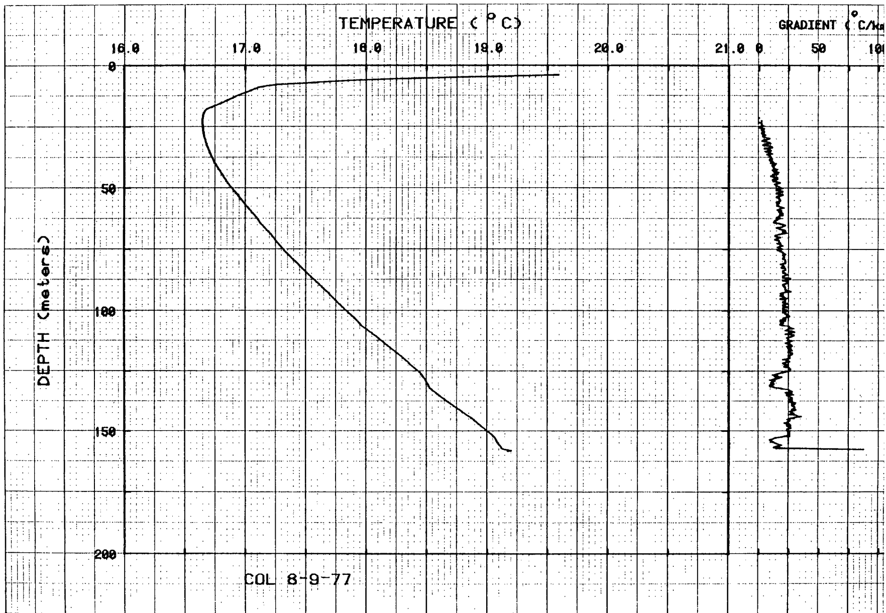
Figure 63. Temperatures and gradients for hole COL.
