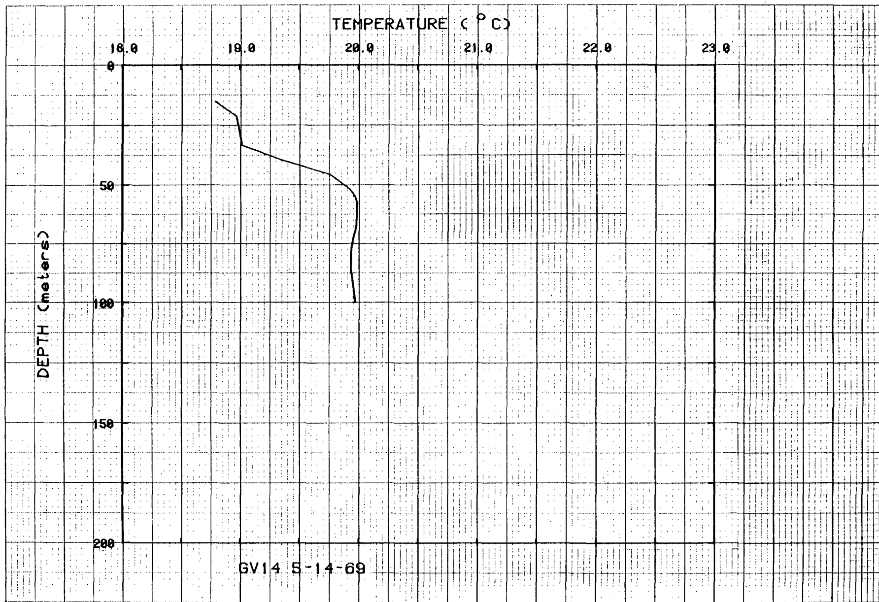
Figure 22. Temperatures for hole GV14.
