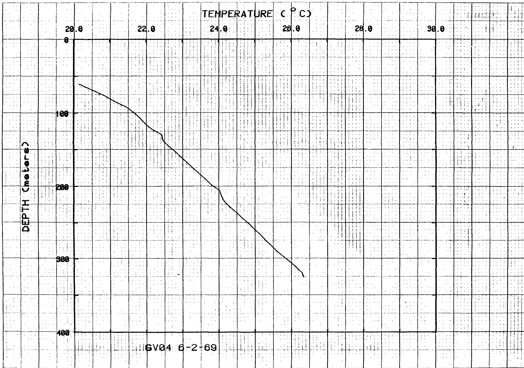
Figure 13. Temperatures for hole GV04.
