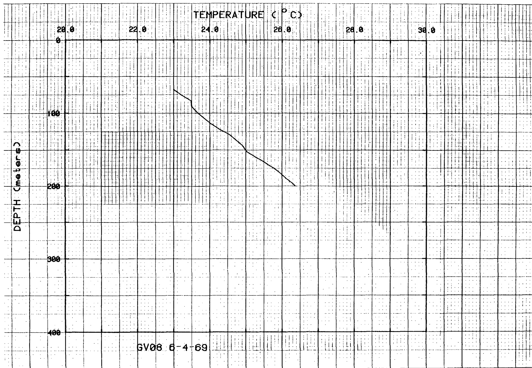
Figure 17. Temperatures for hole GV08.
