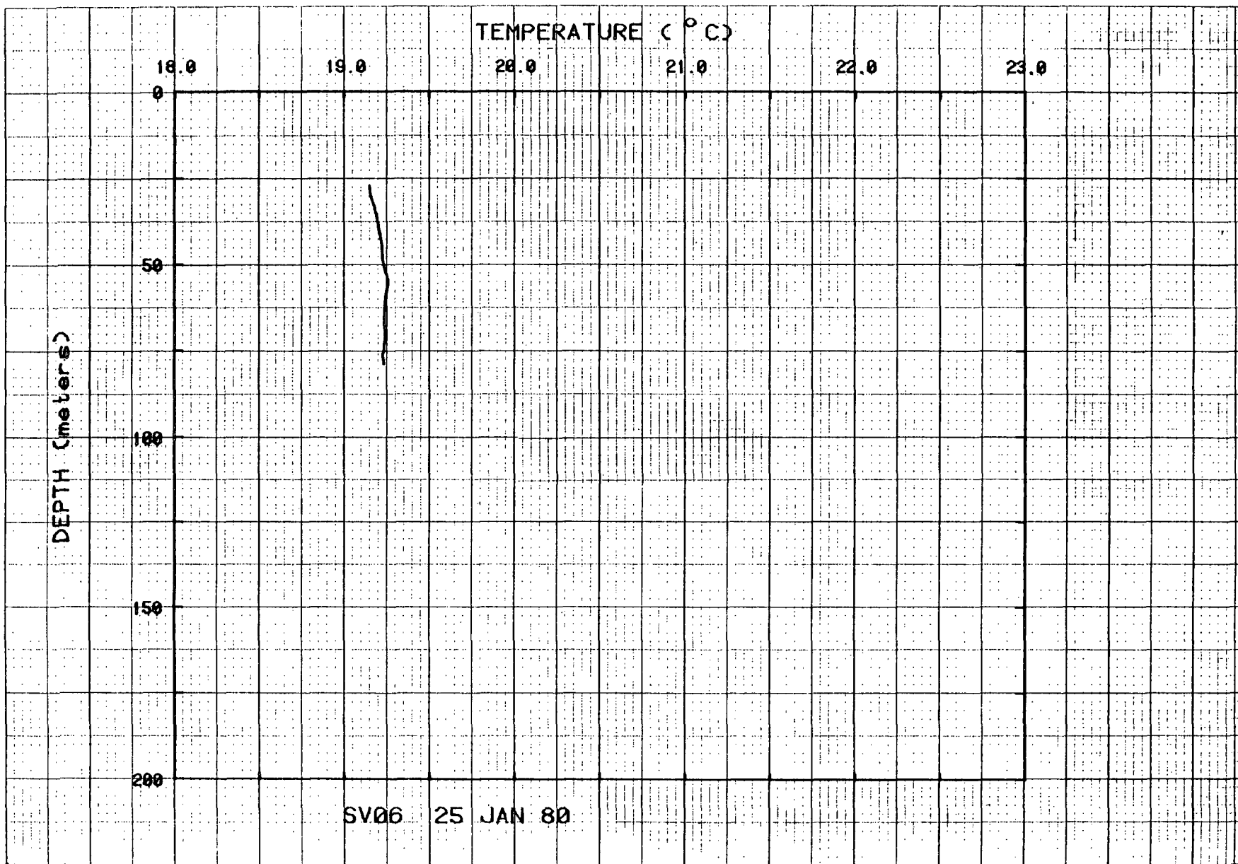
Figure 71. Temperatures for hole SV06.
