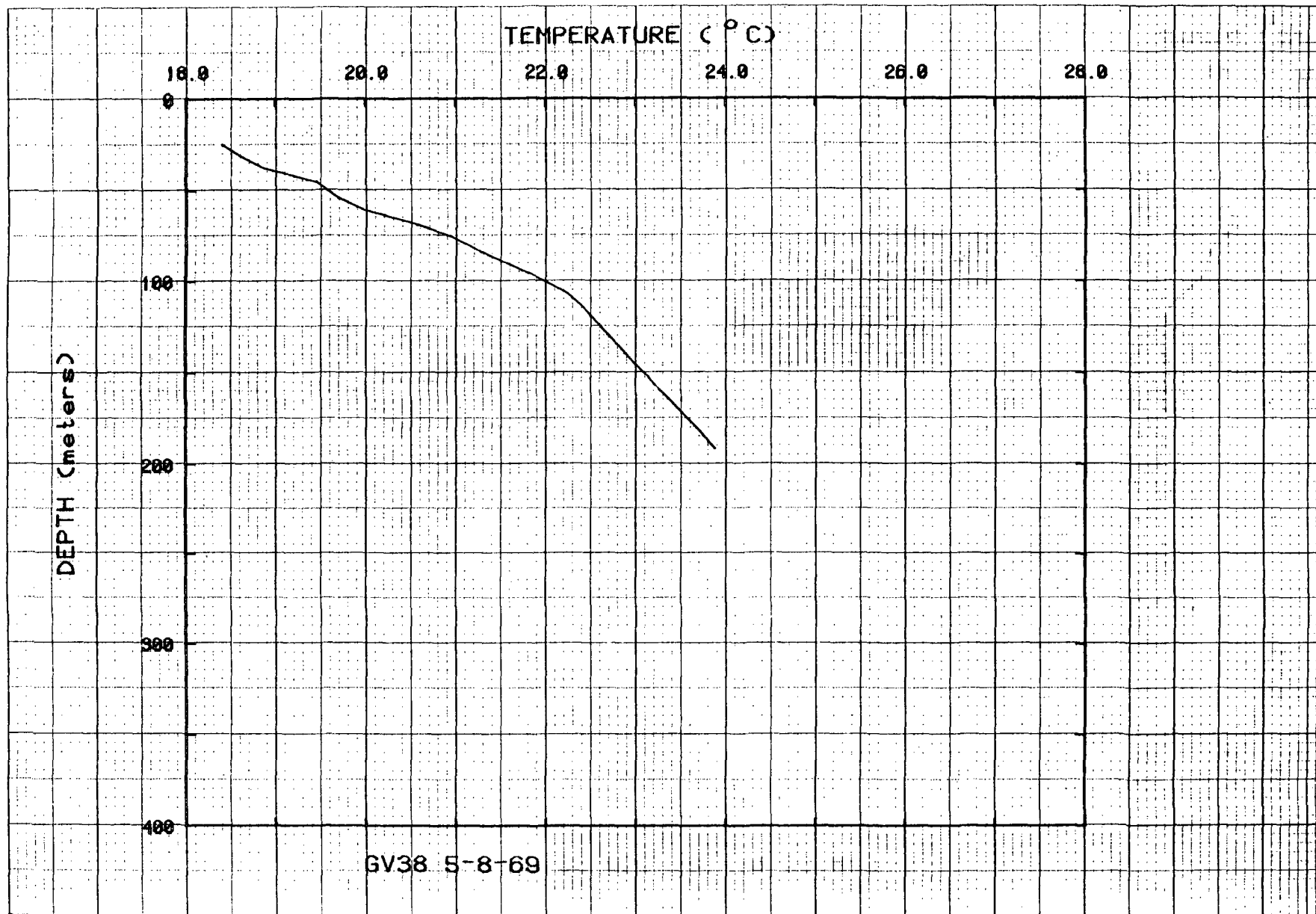
Figure 45. Temperatures for hole GV38.
