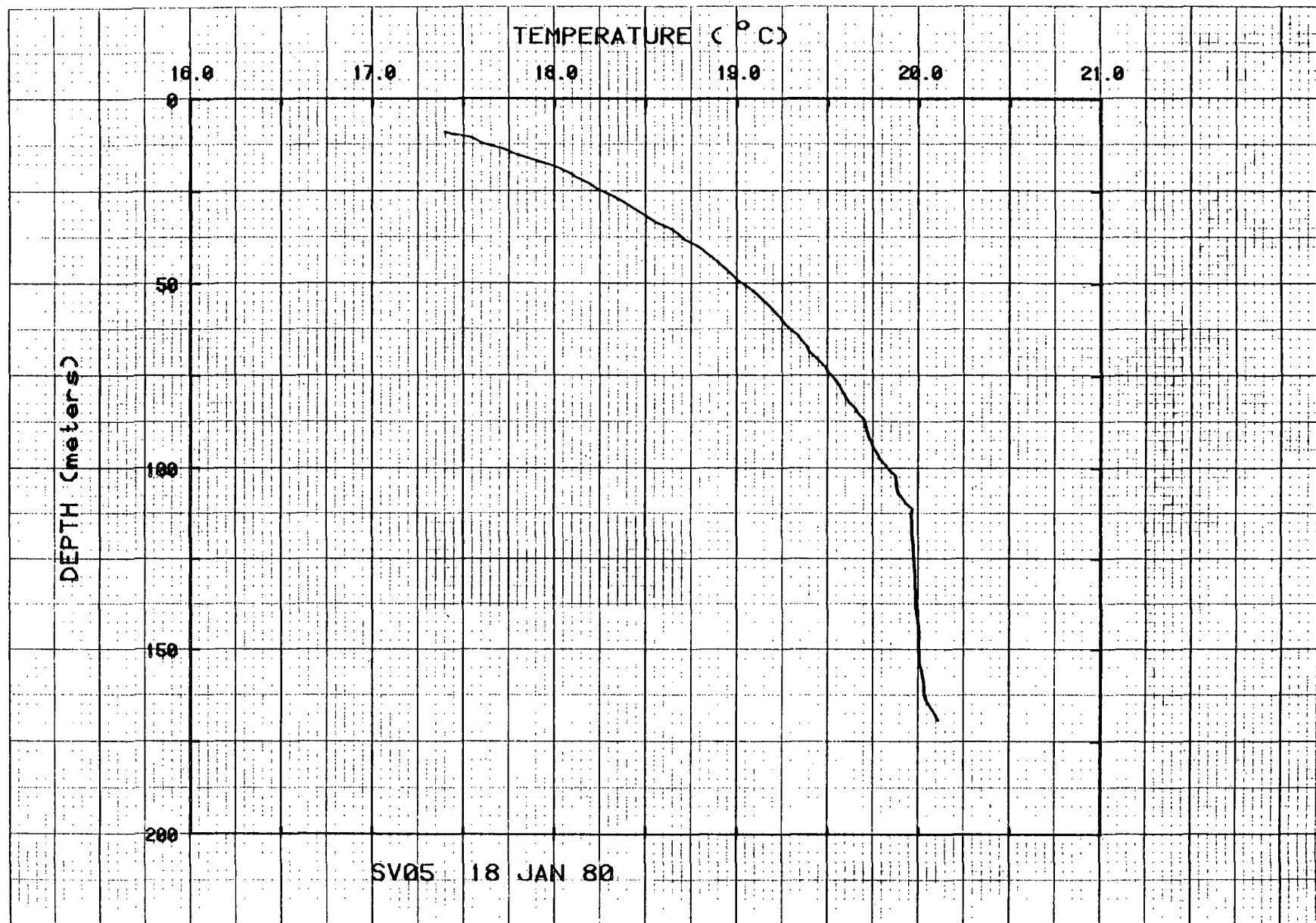
Figure 67. Temperatures for hole SV05.
