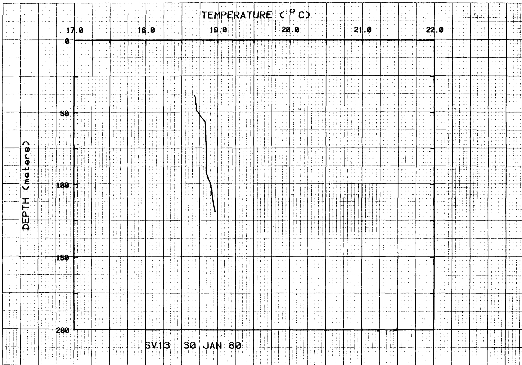
Figure 64. Temperatures for hole SV13.
