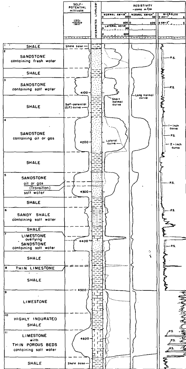
Numbers on column indicate depth in feet. AM, AD refer to electrical circuits employed in obtaining the respective resistivity curves.
