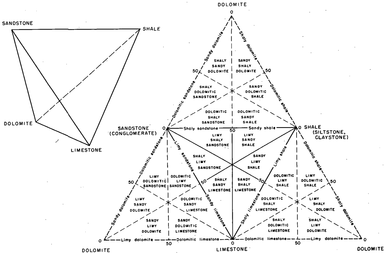
Figure 11. Tetrahedral diagram illustrating classification of commonly associated carbonate and siliceous clastic rocks in drill cuttings.
