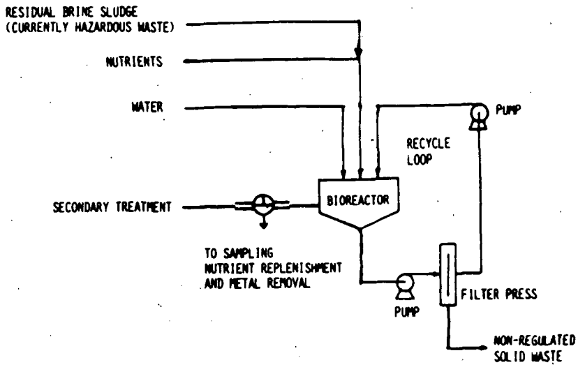
Figure 1. Block diagram for a fluidized bed bioreactor
