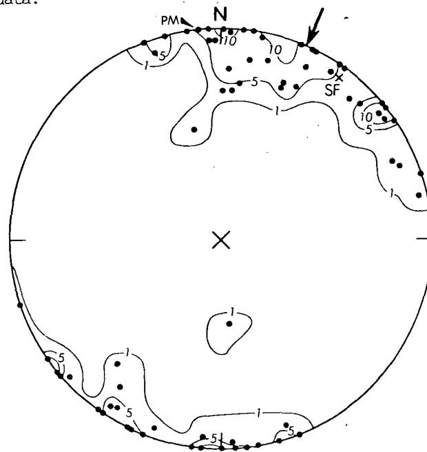
Figure 2.—Stereoplots showing distribution and orientation of P axes for 51 events, 1970-75, excluding aftershocks of 1973 Point Mugu sequence. PM, Point Mugu main shock; SF, 1971 San Fernando main shock (not contoured). Contours, 1 percent, 5 percent, and 10 percent per 1 percent area; lower hemisphere projection. Arrow at N. 24° E. normal to San Andreas fault. See table 4, chapter A for data.
