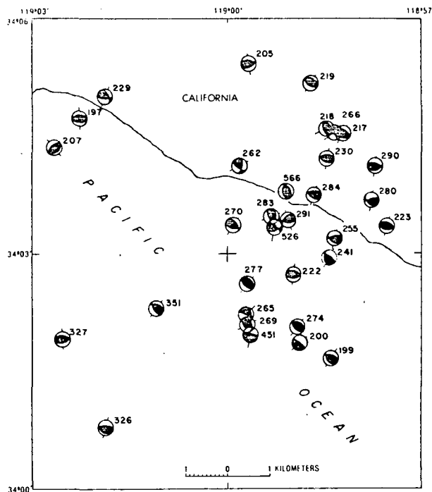
Figure 6.—Focal mechanisms for 1973 Point Mugu earthquake (No. 197) and aftershocks. Numbers indicate sequence of events (see table 2, Chap. A). Compressional quadrants dark, dilatational quadrants light; lower focal hemisphere. Bar shows orientation of P axis. Diagrams located at epicenter of event. Location and area of map shown on plate 2.
