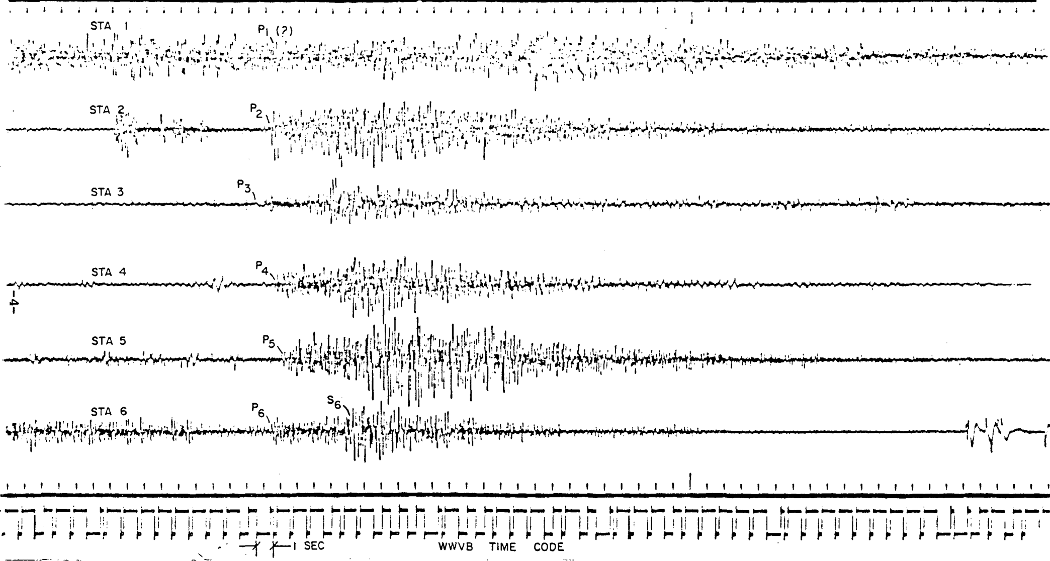
FIGURE 3. Craine Creek cluster microearthquake (NW NEV 1: Event #48).
