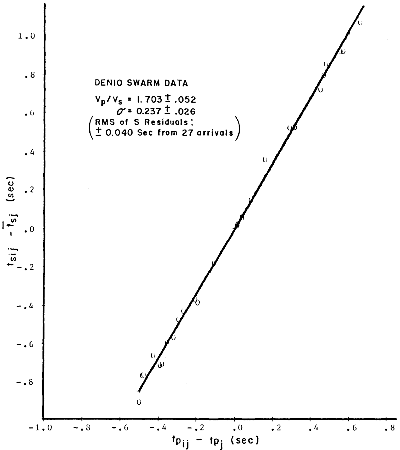
FIGURE 6. Reduced Wadati diagram for V_p/V_s determinations from seven Denio events. t_{p_{ij}} and t_{s_{ij}} are the respective P and S arrival times at the i th station from the j th event. \bar{t}_{p_j} and \bar{t}_{s_j} are the mean P and S times for the j th event.
