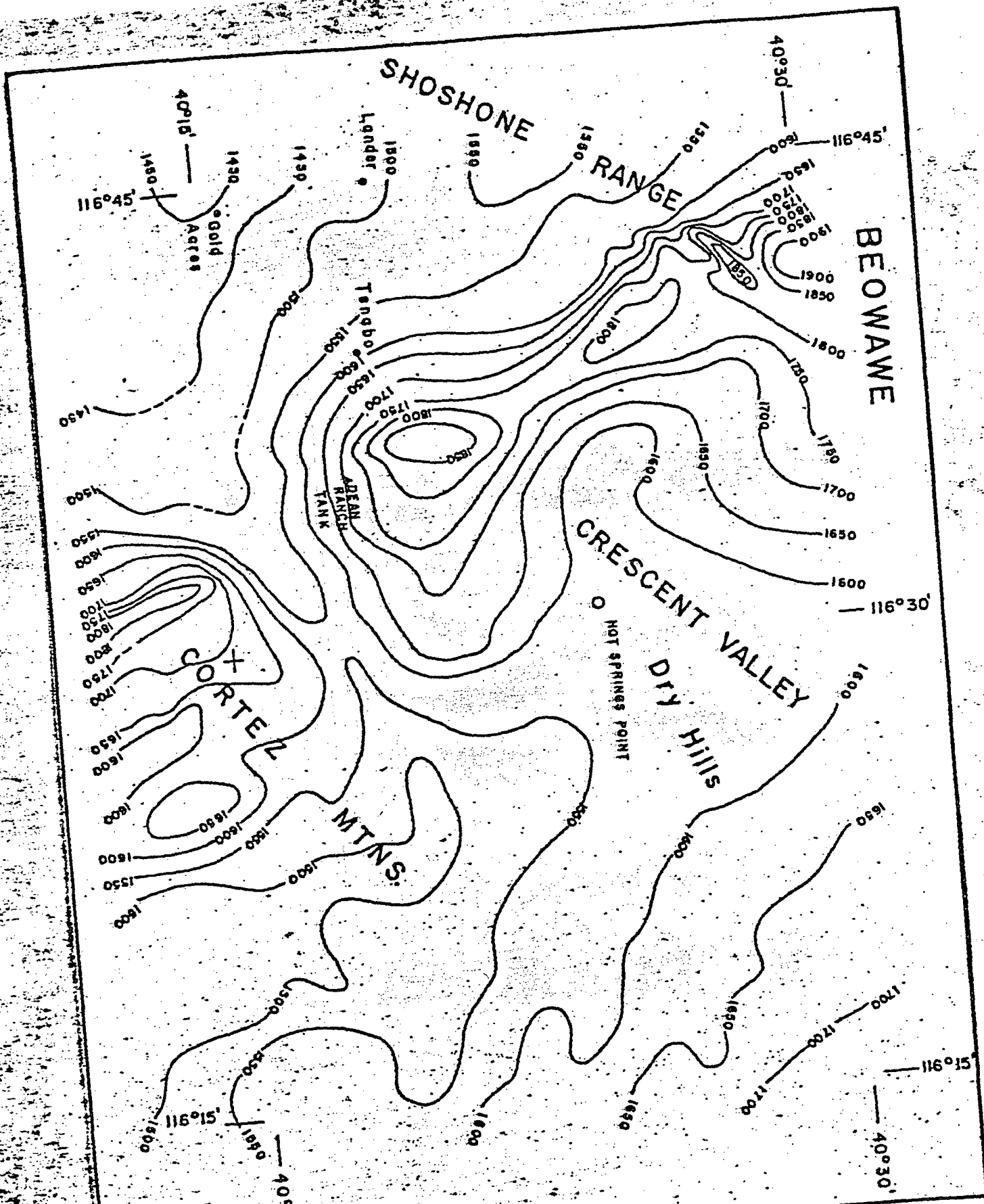
Figure 2. Aeromagnetic map of the Dry Hills and Central Crescent Valley area. Magnetic contours show total intensity magnetic field of the earth in gamma. Contour interval is 50 gammas. Scale is 1:250,000 (after Philbin, et al., 1963).
