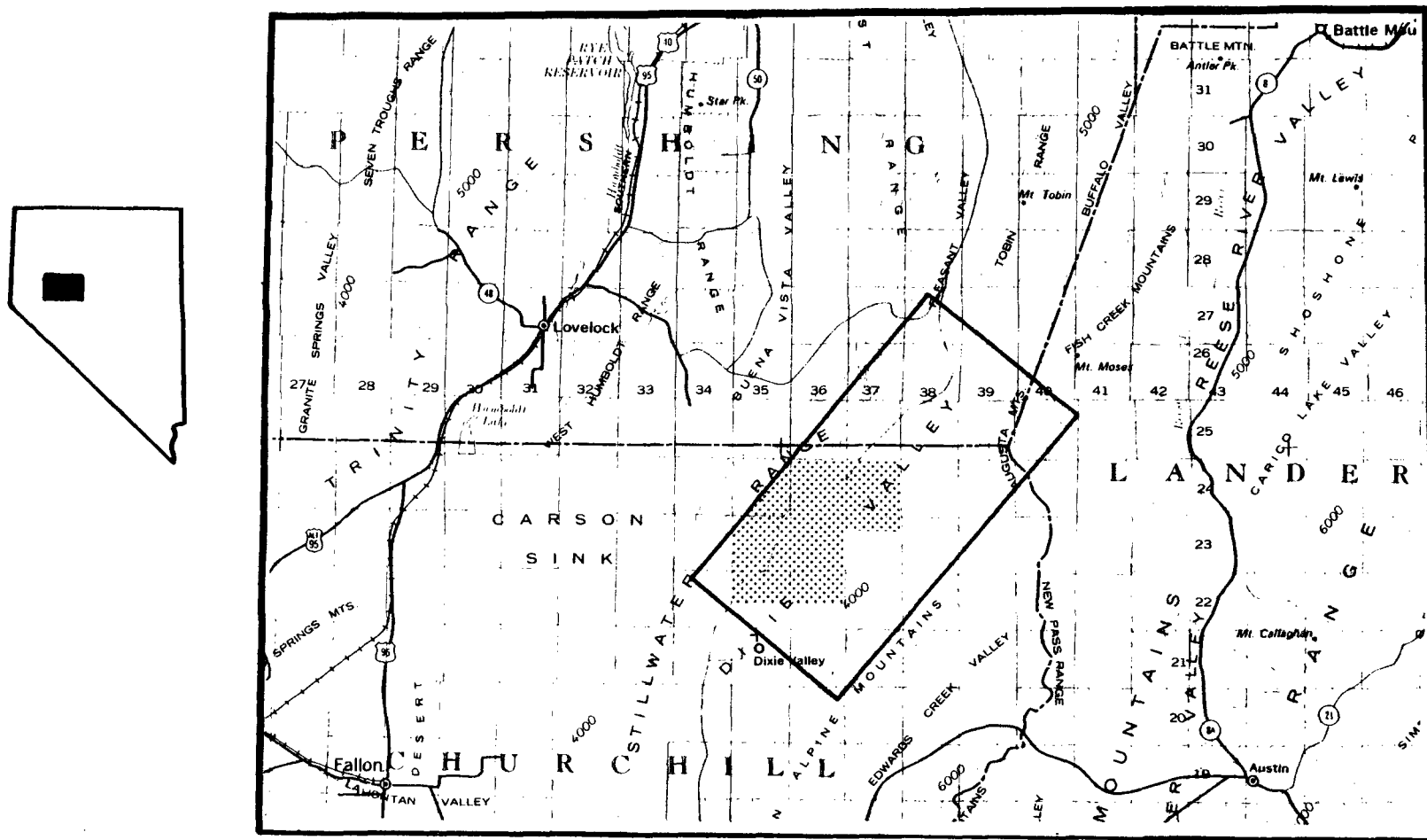
Figure 1-1. Index map of Dixie Valley study region. Shaded area of State shown enlarged. Area encompassing soil geochemistry and petrochemistry studies is shown (in pattern) within the Dixie Valley prospect area; refer to Plate I for detail.
