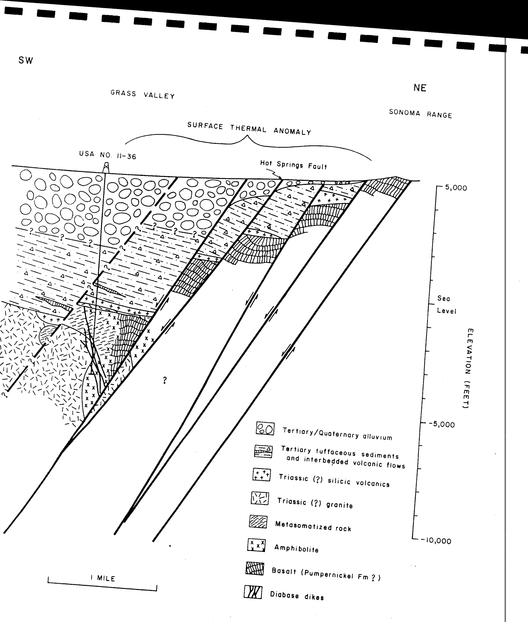
FIGURE 5. Hypothetical cross-section through USA No. 11-36. Line of section shown in figure 1.
