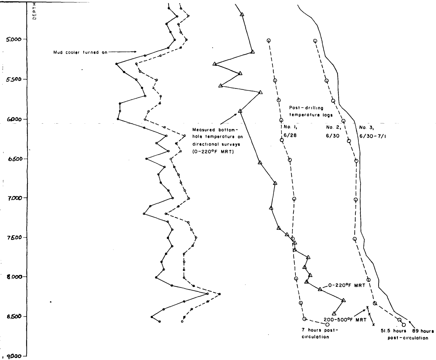
FIGURE 3. Temperature data for USA No. 11-36.
