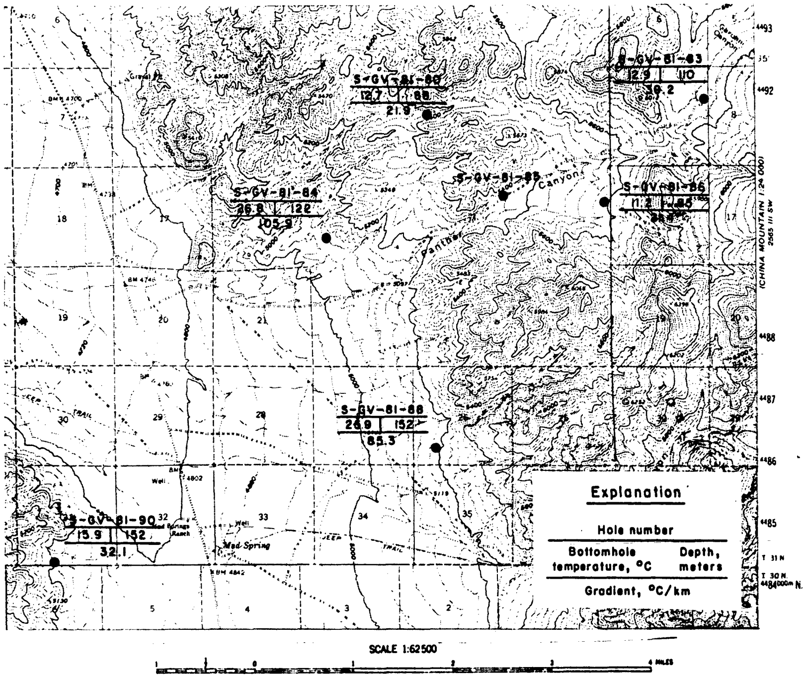
Figure 1: Locations, depths, bottom-hole temperatures, and gradients of temperature-gradient holes, Panther Canyon Project, Nevada
