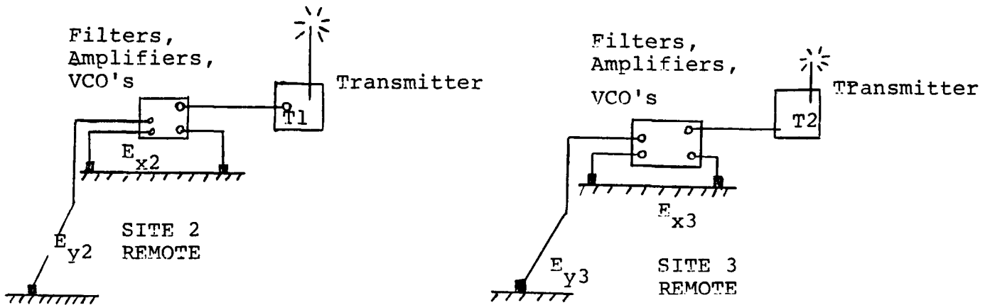
TELLURIC SETUP
