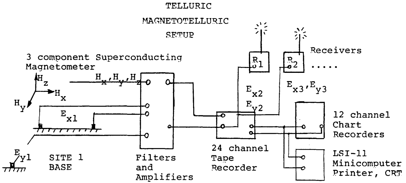
MAGNETOTELLURIC SETUP
