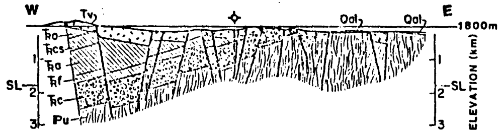
Figure 11. Gravity profile with automatic interpretation for densities (top) after Rerkman (1980) compared with geologic cross-section (bottom) after Pilkington, 1980.
