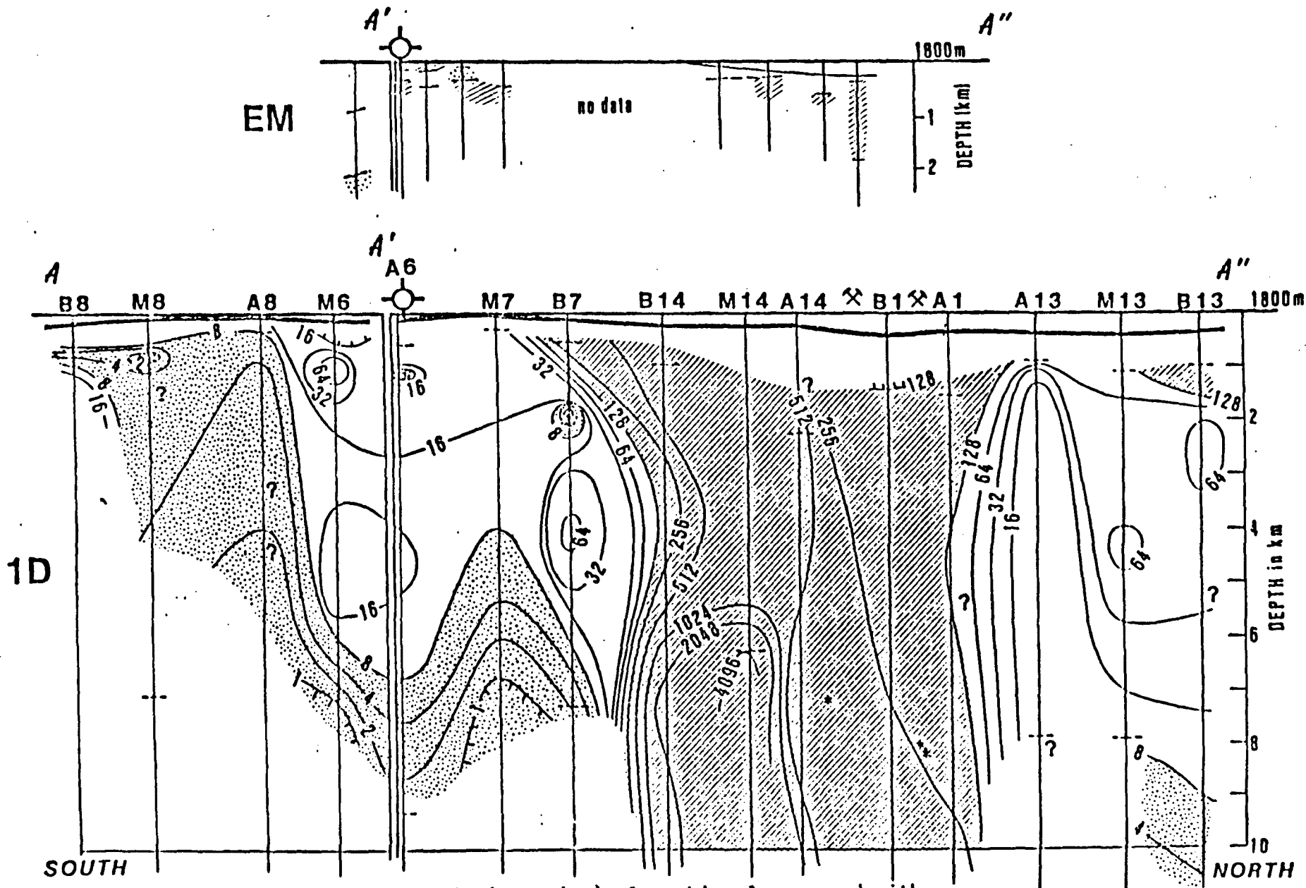
Figure 15. MT section (T mode, 1D inversion) along Line A compared with available EM data, after Lange, 1980.
