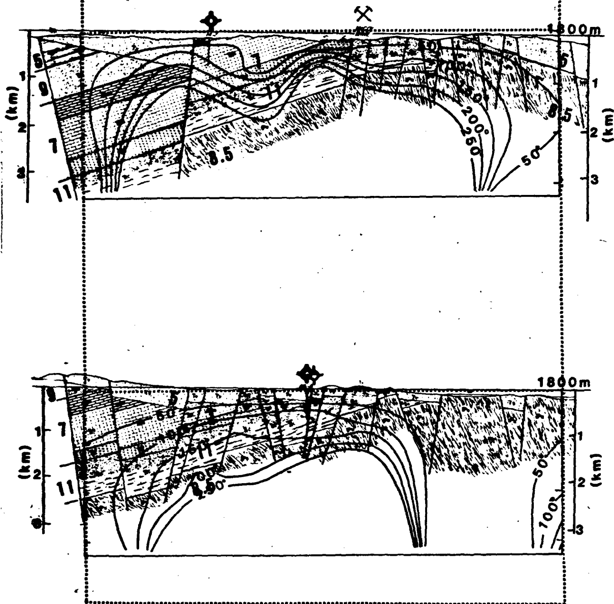
Figure 28. Three-dimensional downward continuation with extended aquifers (Tra limestone at well 14-7 and Trc conglomerate at well 66-8) superimposed on geologic sections, after Lange, 1981.
