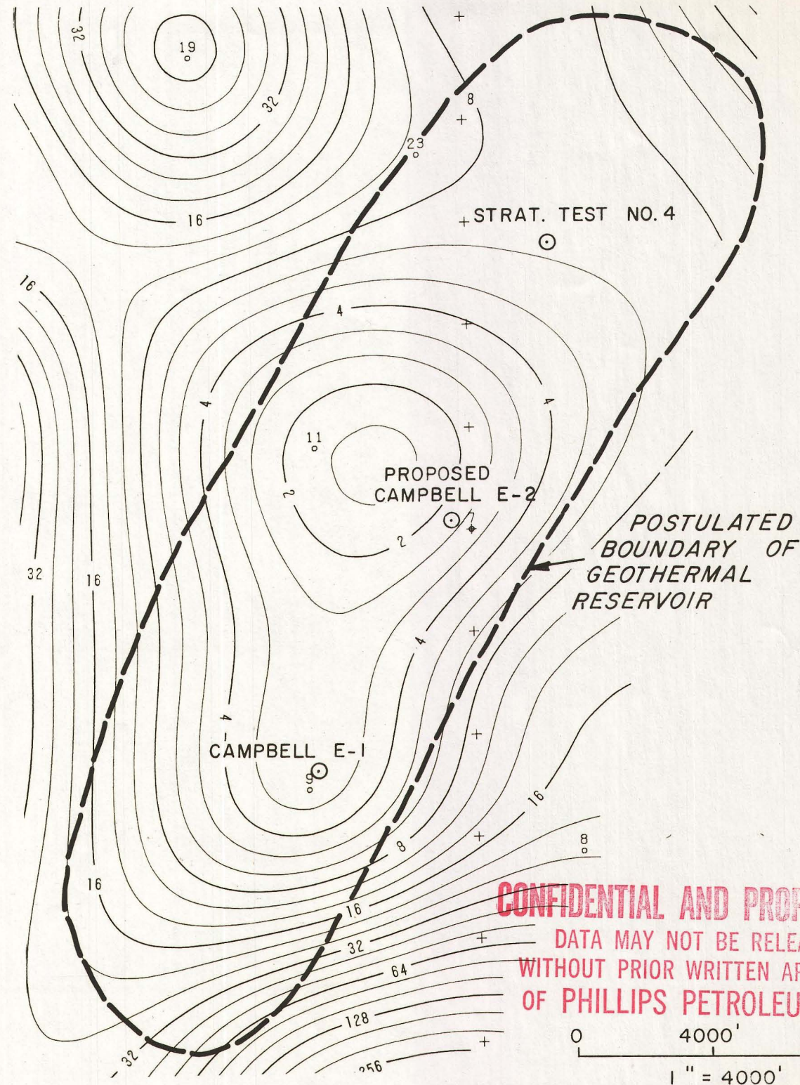
MAGNETOTELLURIC SLICE MAP AT A DEPTH OF 3000' - HUMBOLDT HOUSE PROSPECT PERSHING COUNTY, NEVADA
