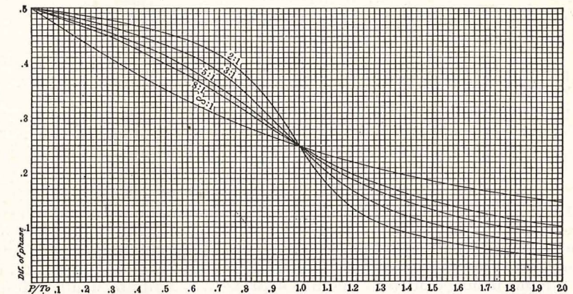
FIGURE 7.—Differences in phase for linear displacements—applicable to direct recording seismographs. (From report of the California Earthquake Commission.)
