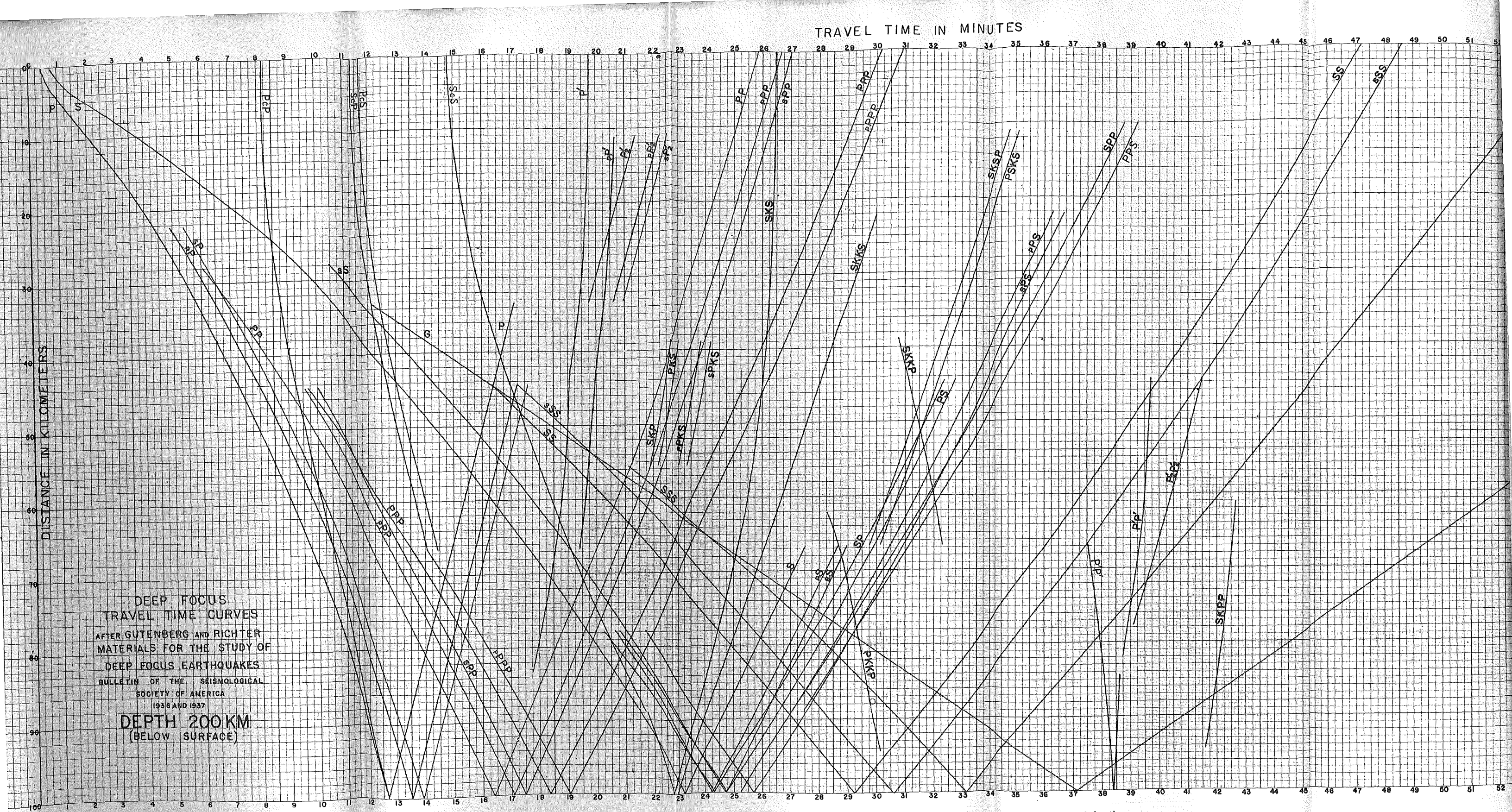
FIGURE 14. Gutenberg-Richter travel-time chart for 200 km. focal depth.
