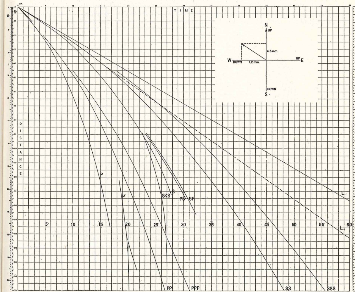
FIGURE 1.—A simplified form of travel-time chart showing approximate travel times of principal phases for shallow focus earthquakes. Insert illustrates method of computing direction of ground motion from impulsive iP phase.
