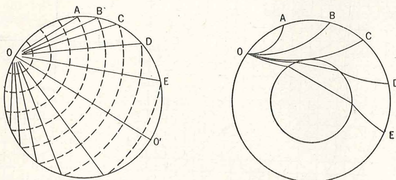
FIGURE 2.—Radiation of waves in a uniformly elastic sphere and in the earth. The diagram on the left illustrates the straight rays and spherical wave fronts that would result from a surface disturbance in an elastic, homogeneous and isotropic sphere. The diagram on the right shows how seismic rays are bent toward the center of the earth because of increase of velocity with depth. The effect of the earth's core in deflecting the rays is also illustrated.
