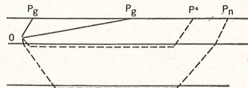
FIGURE 5.—Paths of principal local shock waves in crustal layers according to Jeffreys.
