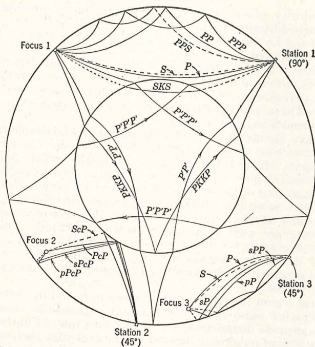
FIGURE 4.—Paths of some of the more important body waves for shallow and deep focus earthquakes. Three foci are indicated. (From L. D. Leet's Earth Waves)
