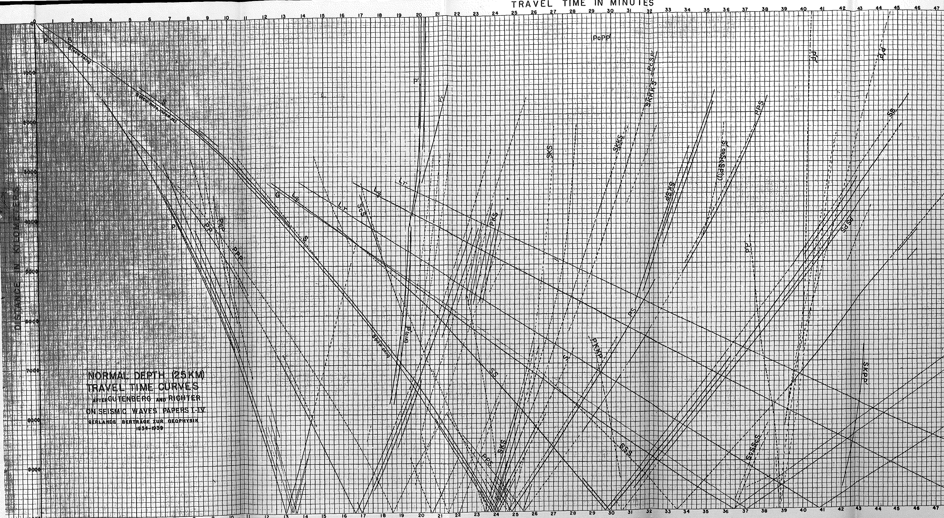
FIGURE 12. Gutenberg-Richter travel-time chart for normal focal depths.
