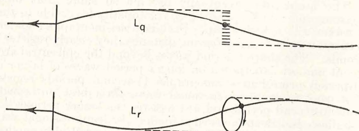
FIGURE 3.—Earth particle motions in surface waves. The upper diagram shows the horizontal earth particle motion transverse to the direction of propagation in the case of L_q waves. The lower diagram shows the retrograde character of the earth particle motion (in the vertical plane) in the case of L_r waves.
