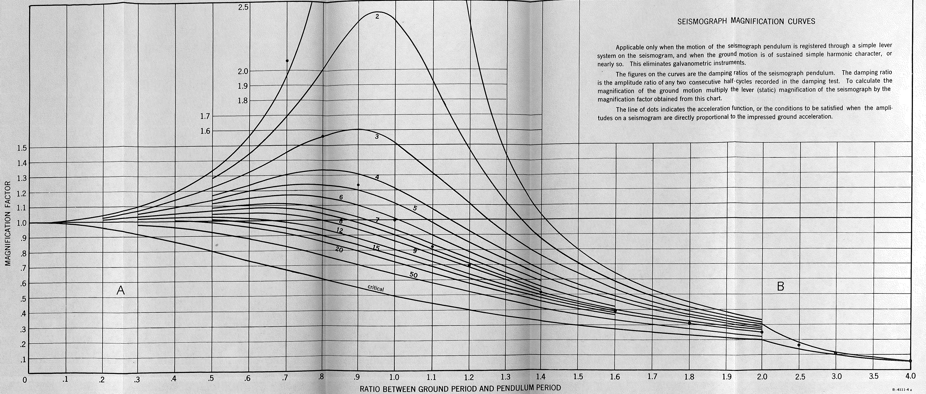
FIGURE 6. Magnification curves for direct recording pendulums with varying damping ratios.
