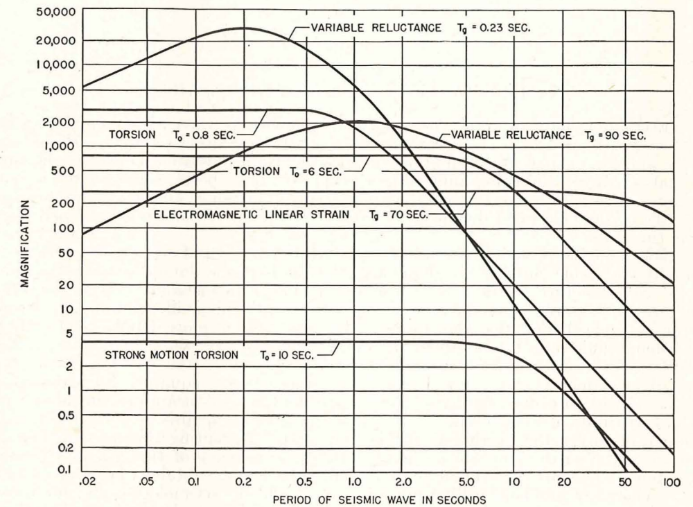
FIGURE 9.—Magnification curves for Benioff, linear strain, and torsion pendulum seismographs at Seismological Laboratory of the California Institute of Technology.
