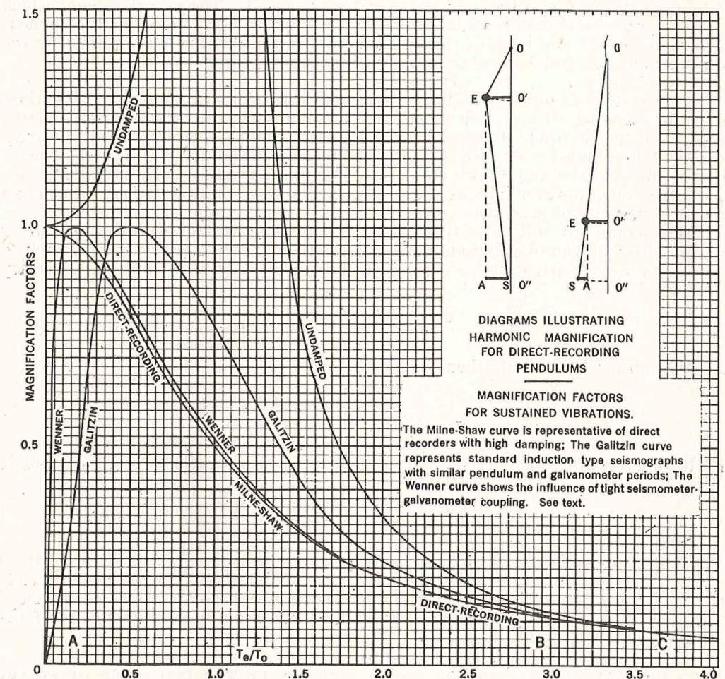
FIGURE 8.—Magnification curves for various types of seismographs with insert illustration harmonic magnification.
