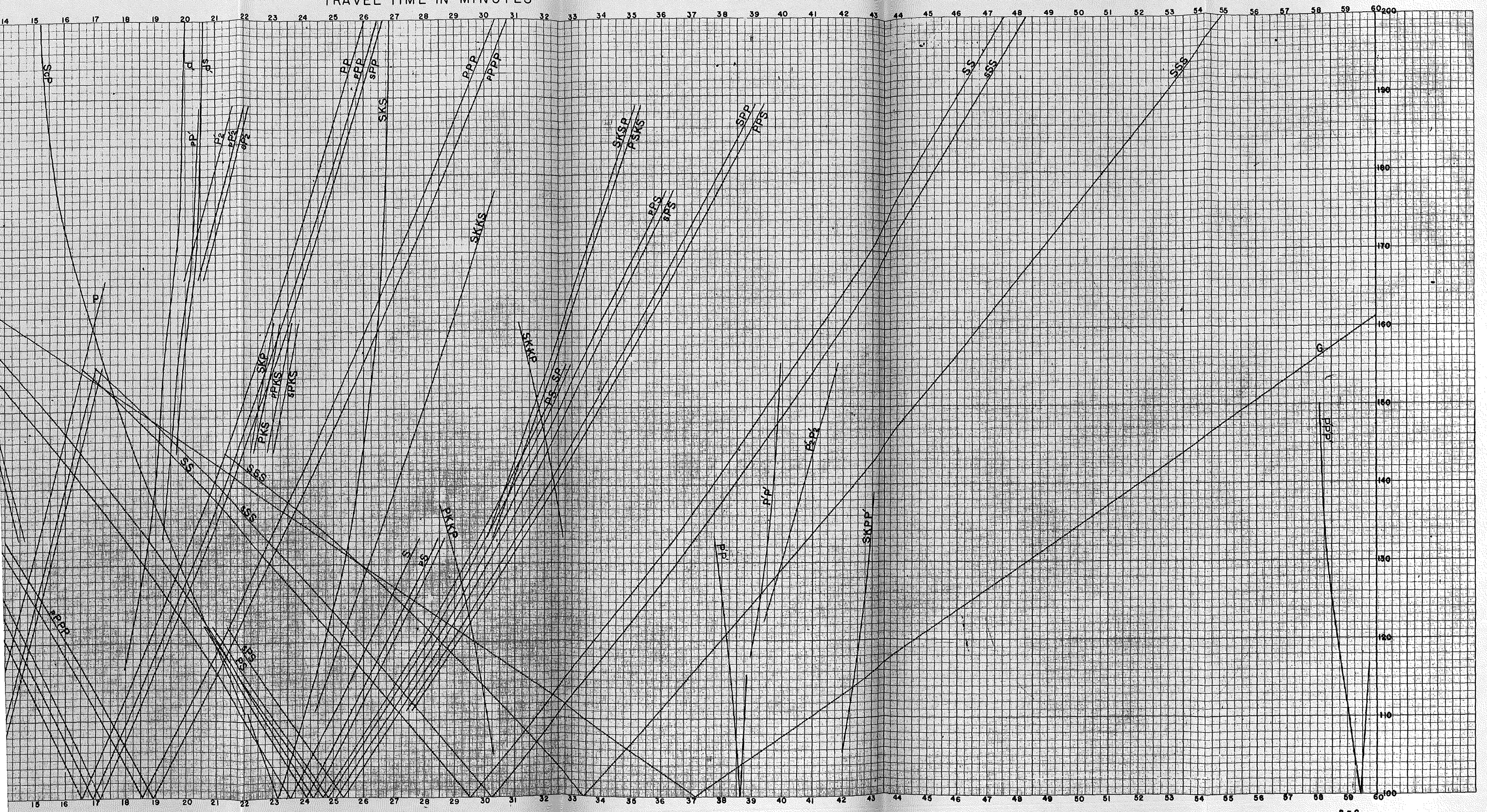
FIGURE 13. Gutenberg-Richter travel-time chart for 100 km. focal depth.
