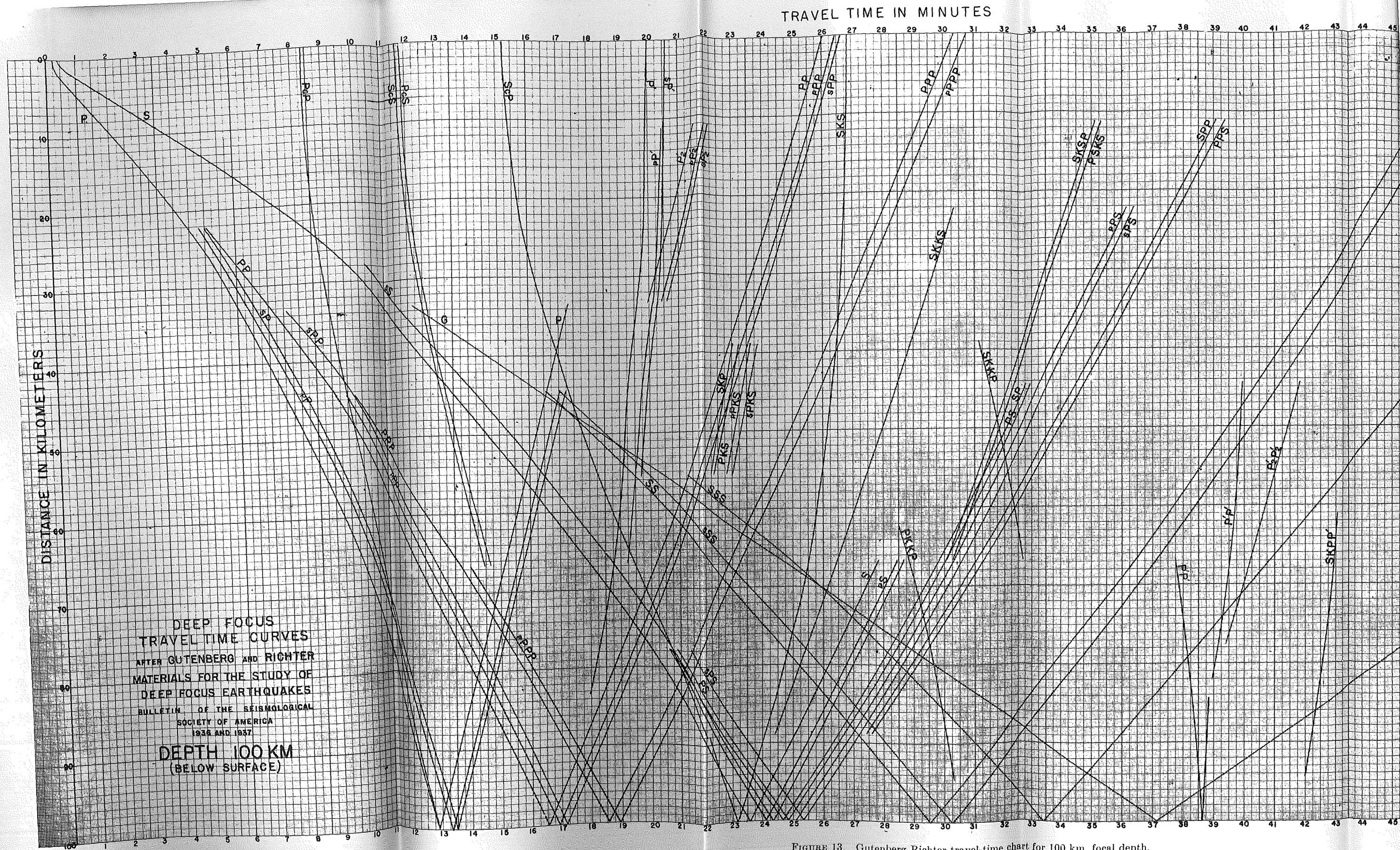
FIGURE 13. Gutenberg-Richter travel-time chart for 100 km. focal depth.
