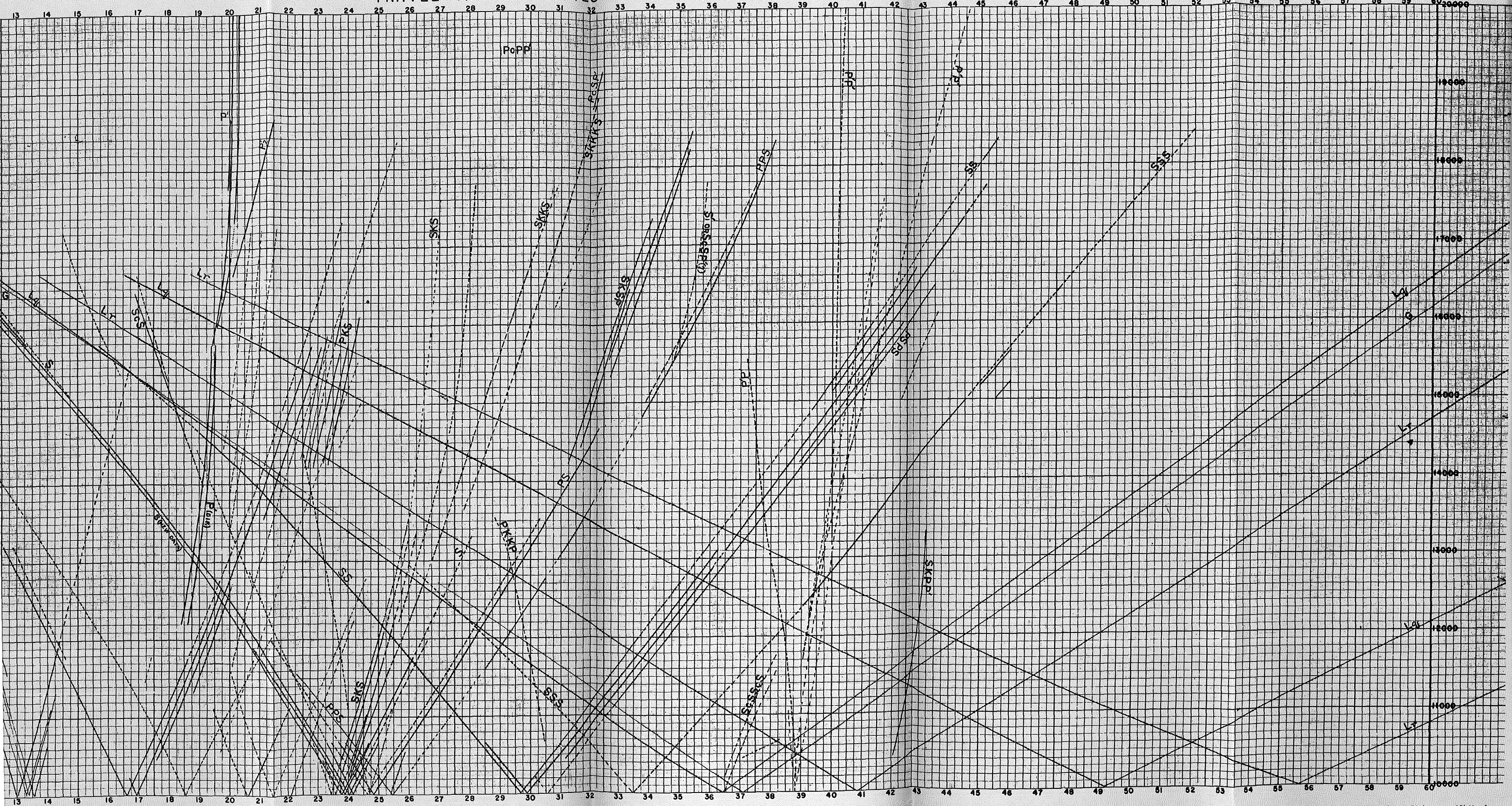
FIGURE 12. Gutenberg-Richter travel-time chart for normal focal depths.
