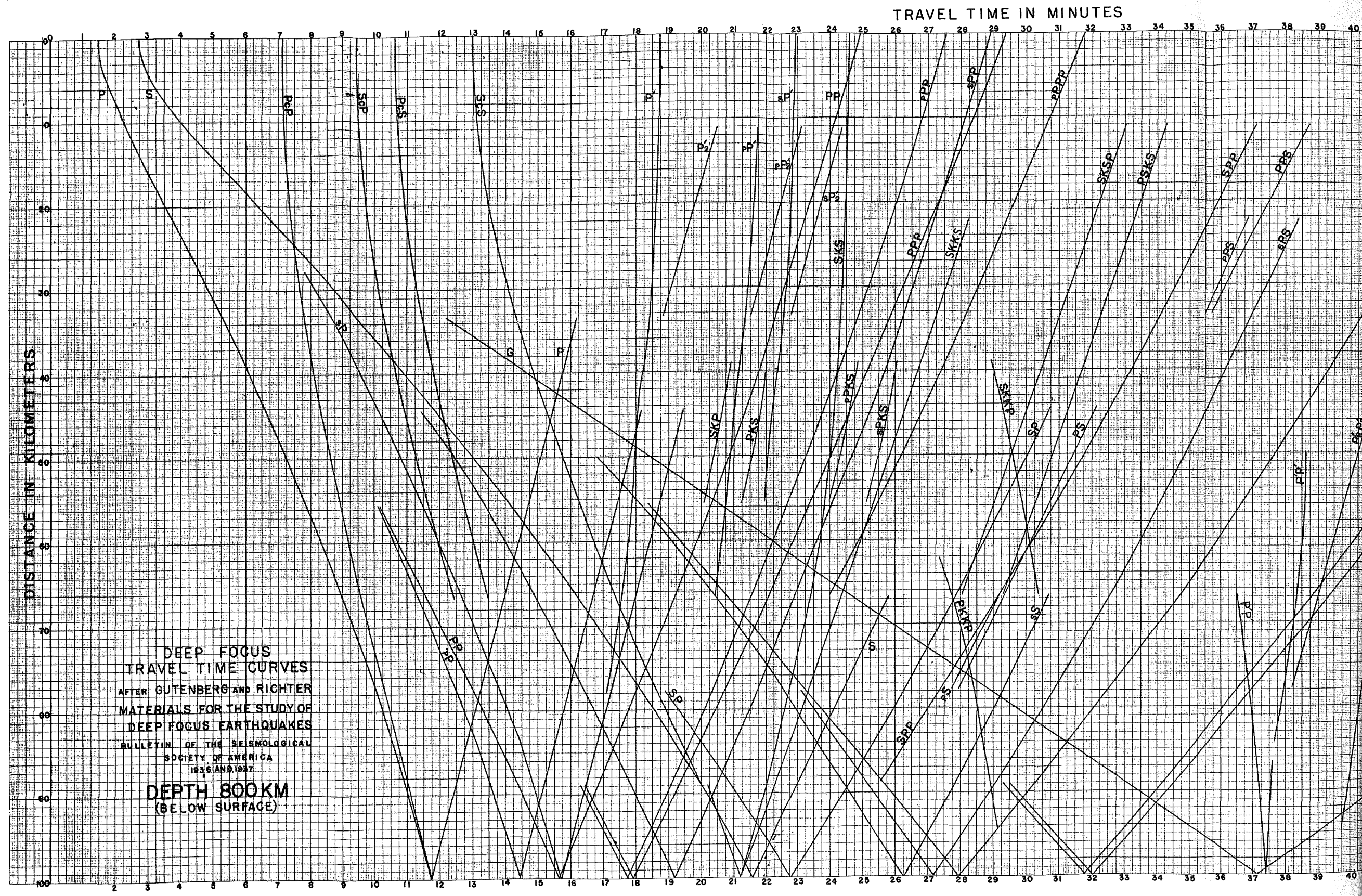
FIGURE 15. Gutenberg-Richter travel-time chart for 800 km. focal depth.
