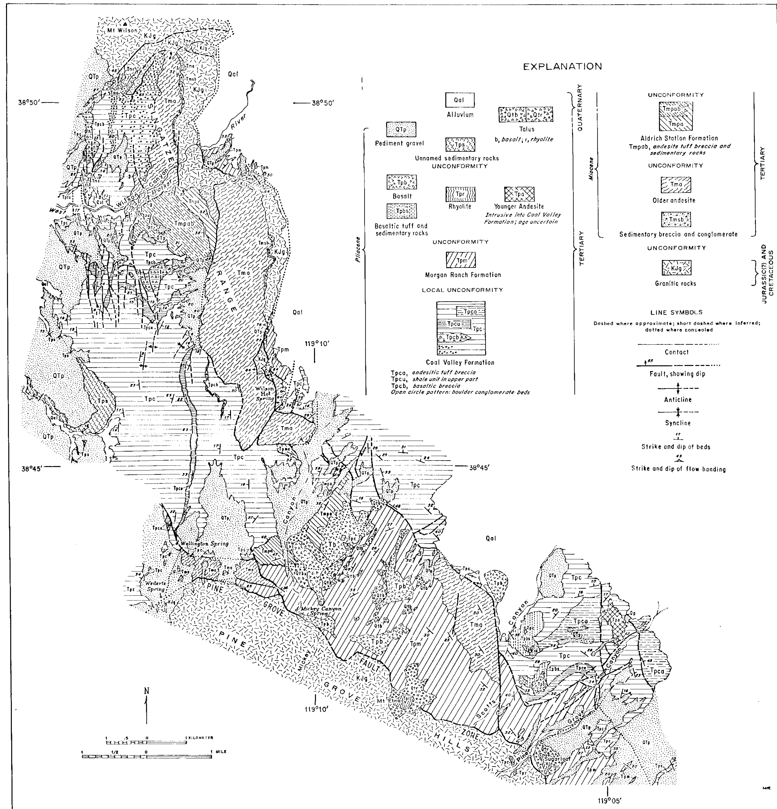
Figure 3. Geologic map of the northern Pine Grove Hills and southern Singatre Range, Lyon County, Nevada.
