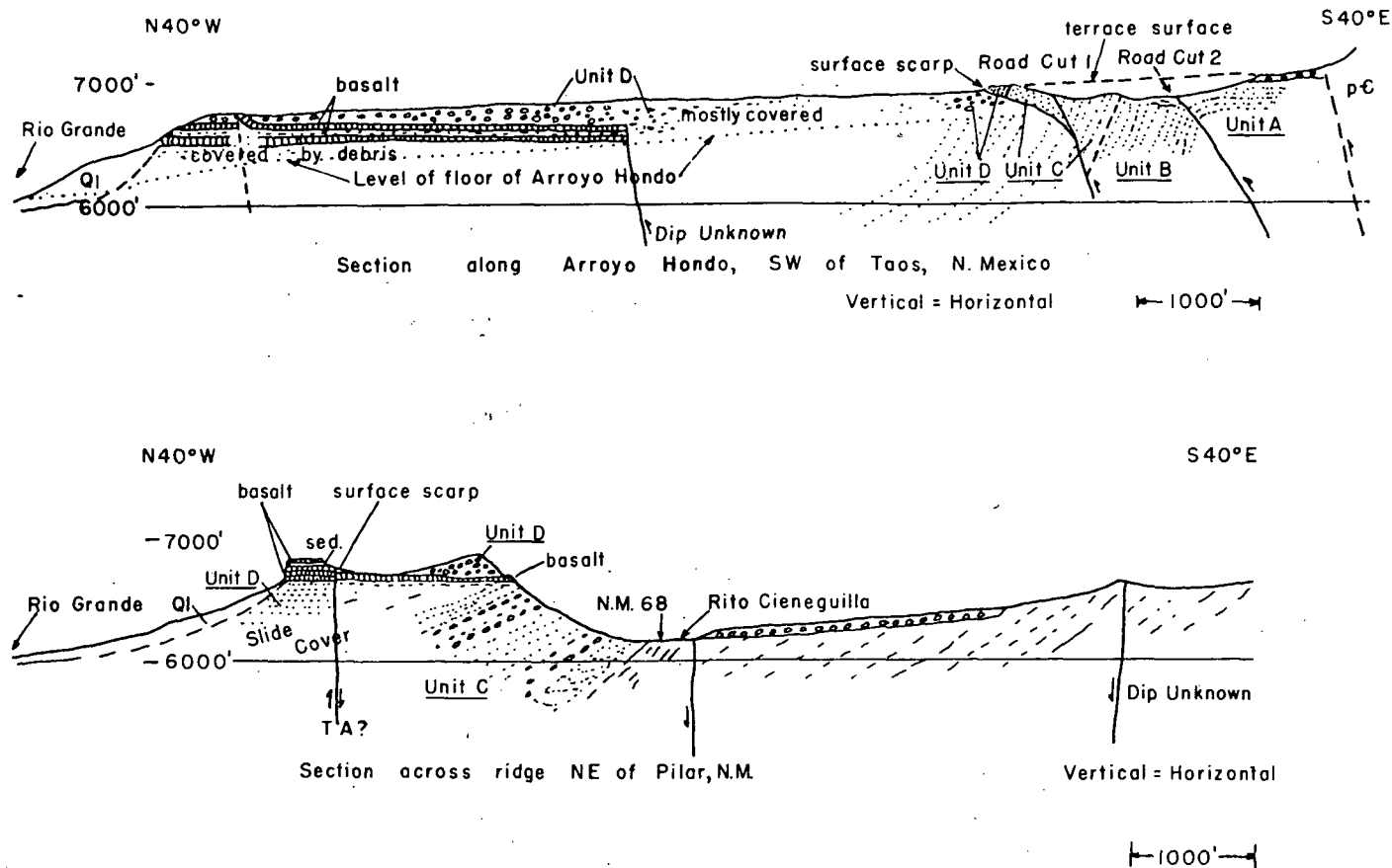
Figure 5. Cross sections across Embudo fault (surface scarp) at Hondo Canyon and Pilar. Units and roadcuts on Hondo Canyon section are those of Figure 4. Basalts are part of Servilleta Formation. Lower Servilleta Formation underlies basalt. Dips of beds east of Rito Cieneguilla show approximate structure pending detailed study. Dip of Embudo fault at Pilar is unknown because of landslide cover and pipeline debris. Surface scarp is down to south in the section and reverses to north side down about 1000 ft (300 m) northeast along strike.
