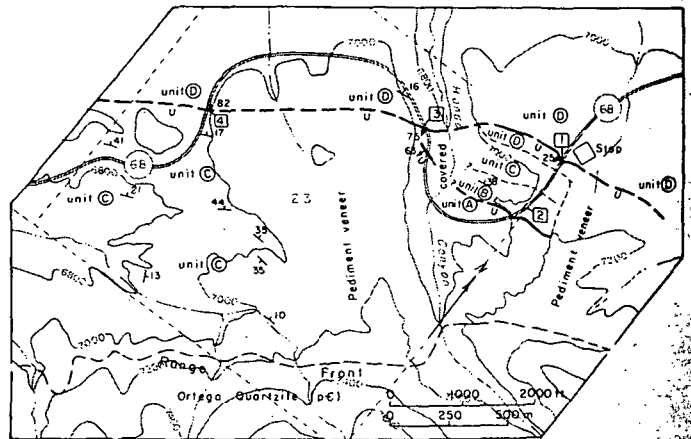
Figure 3. Sketch map of Hondo Canyon segment of Embudo fault. Base adapted from U.S. Geological Survey Taos Southwest quadrangle. Trace of main fault is marked by a topographic scarp across all geologic units. Map units A-D are those described in text; probable formation names: A, B—Chama-el rito Member of Tesuque Formation (Santa Fe Group); C—Ojo Caliente Sandstone of Tesuque Formation (Santa Fe Group); D—upper Servilleta Formation. Roadcut sections of Figure 4 are numbered boxes. Diamond indicates field trip stop, day 1, at roadside park overlook of Rio Grande Gorge. Modified from Hawley (1978, fig. N31).
