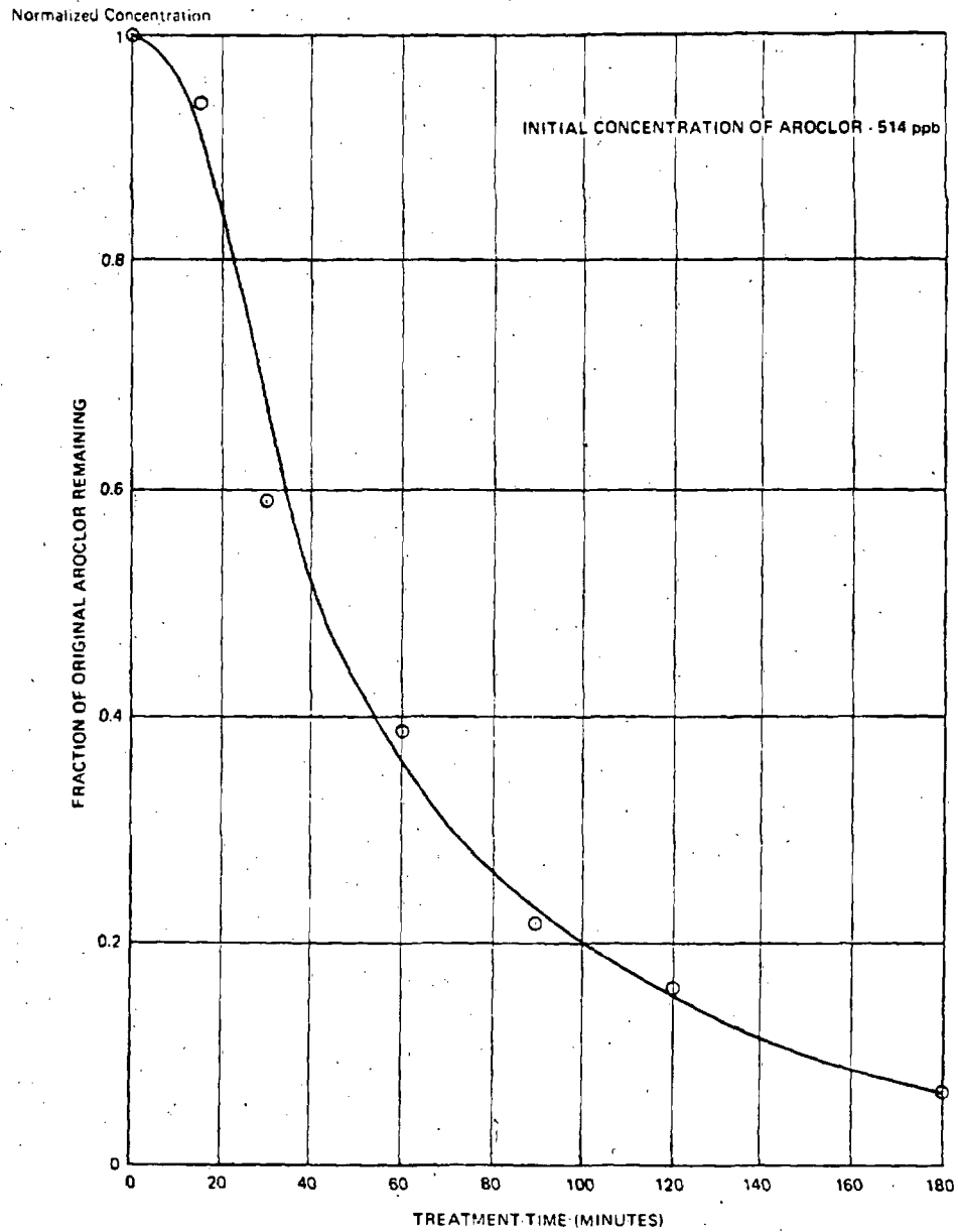
Figure 2.2.2.4.1-2. AROCLOR 1254 DESTRUCTION BY UV-ASSISTED OZONATION
