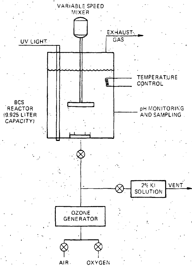
Figure 2.2.2.4.1-1. LAB SCALE APPARATUS FOR REACTION AND MASS TRANSFER STUDIES AT HOUSTON RESEARCH, INC.
