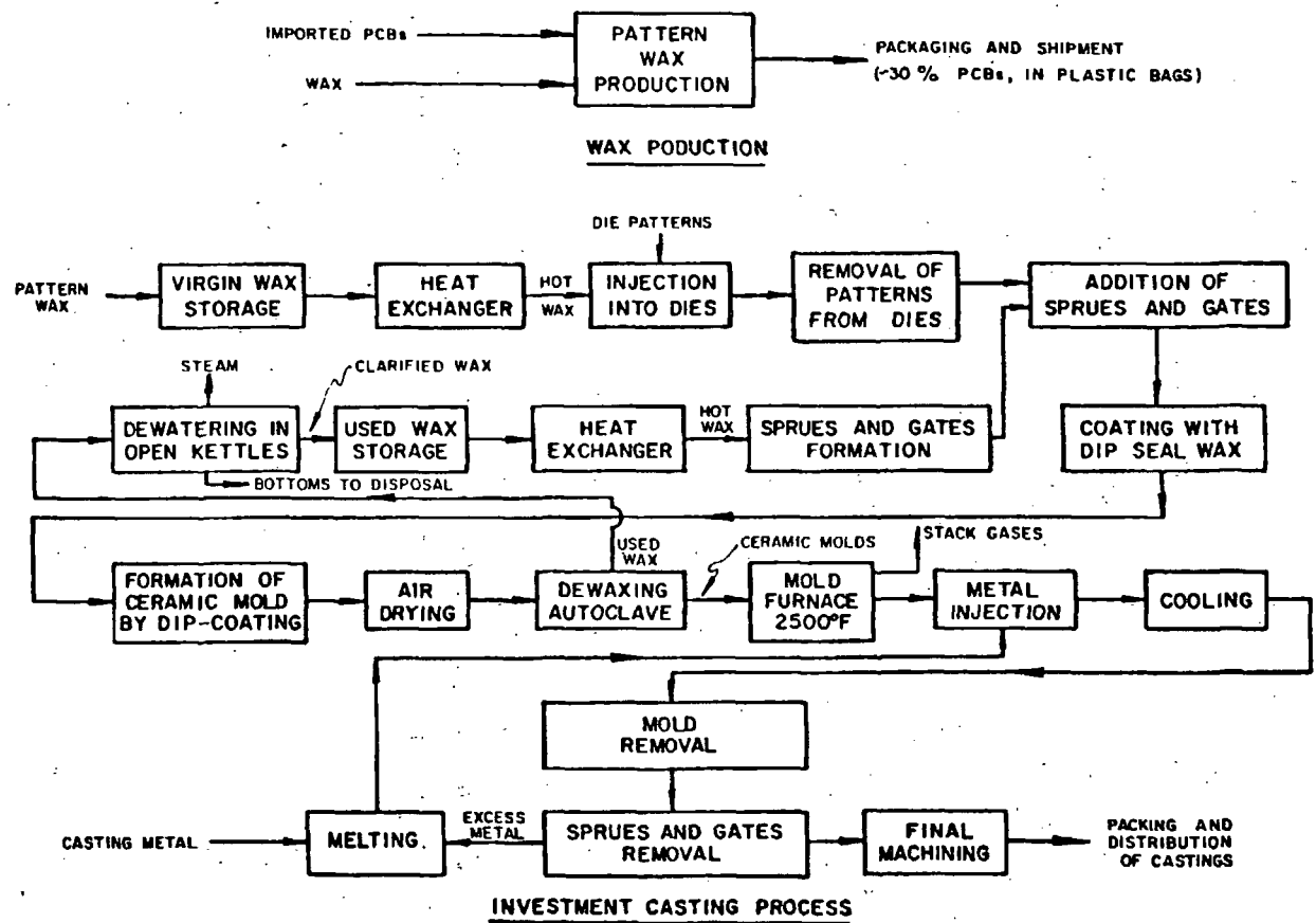
FIGURE 3.3.2.2-1 FLOW CHART OF PCB 8 USAGE IN INVESTMENT CASTING
