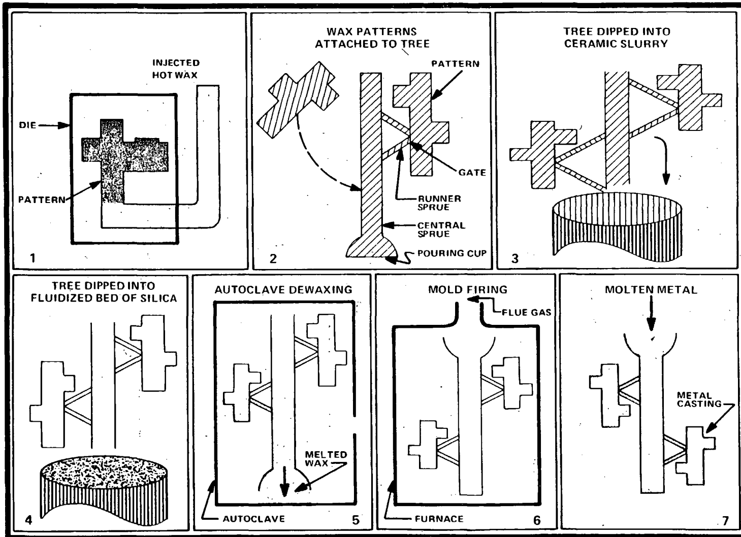
Figure 3.3.2.1-1. INVESTMENT SHELL PROCESS
