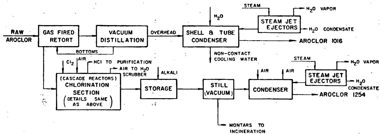
FIGURE 2.1-1B. DISTILLATION OF CRUDE PRODUCTS-MONSANTO KRUMMRICH PLANT
