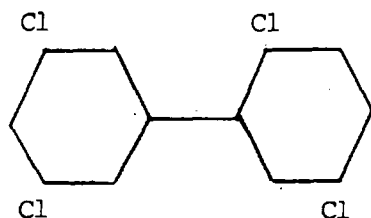
2,3',5,5'-tetrachlorobiphenyl
