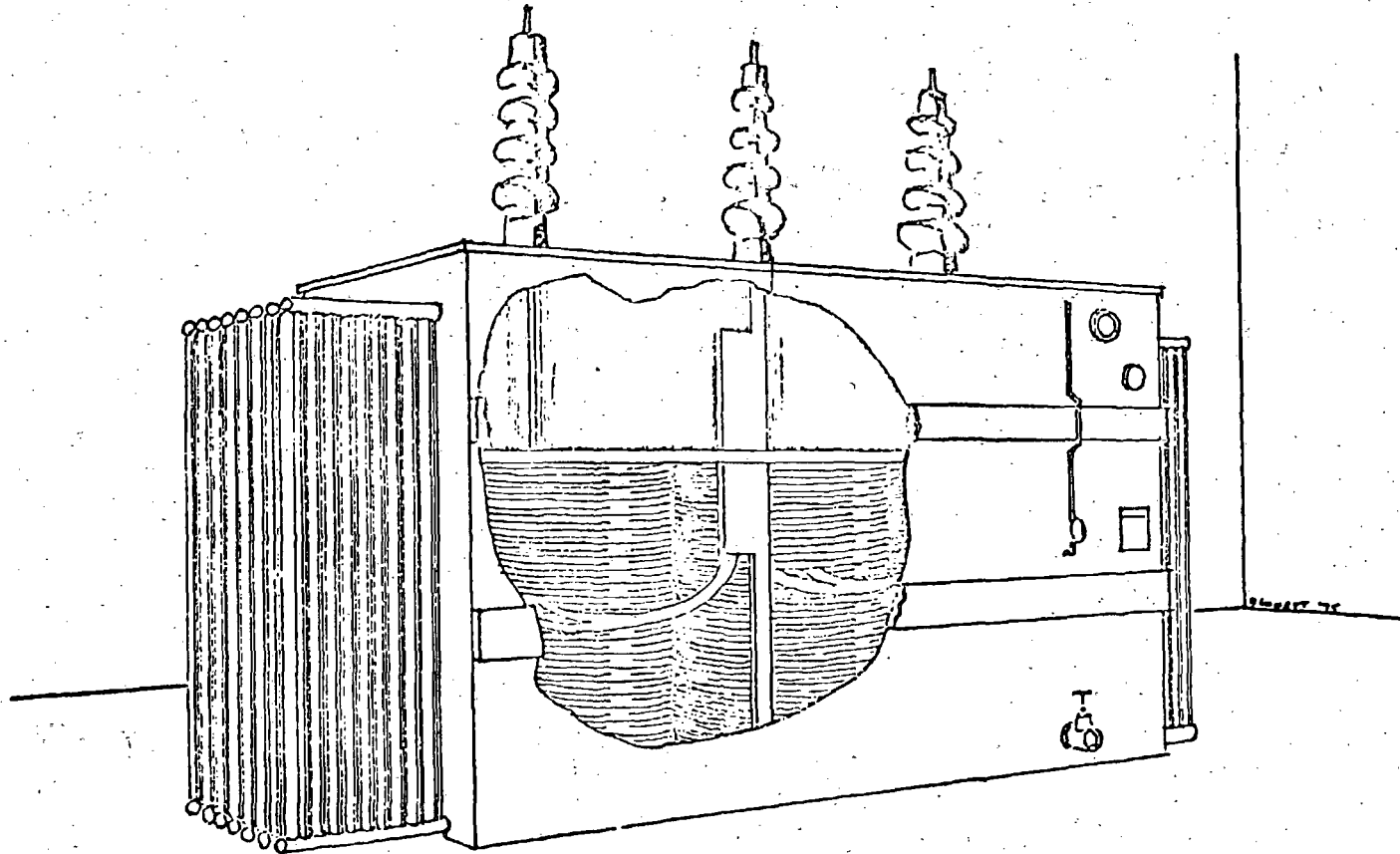
FIGURE 3.2.1-1. SUBSTATION TRANSFORMER
