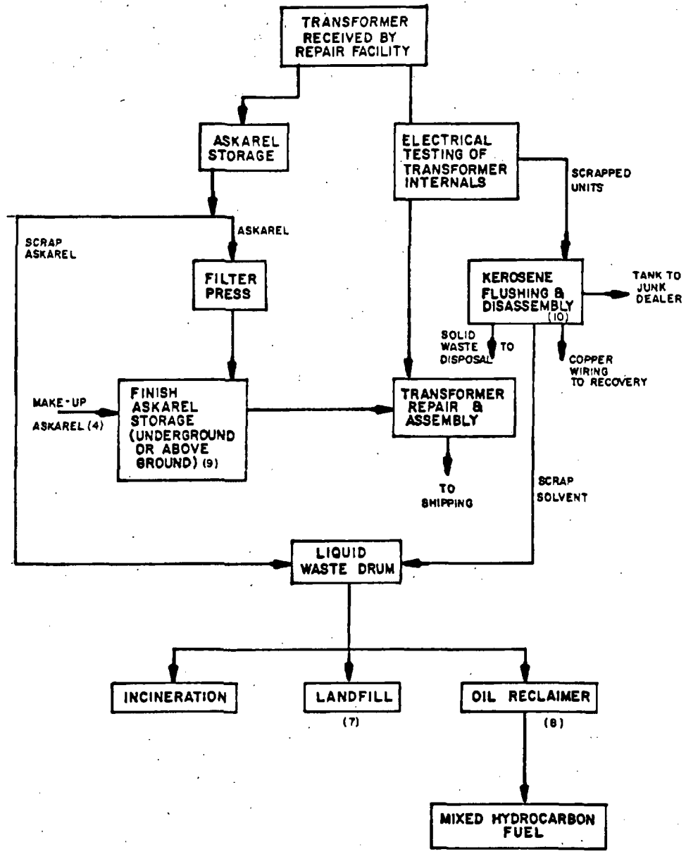
FIGURE 3.2.2.2-2. TRANSFORMER REPAIR
