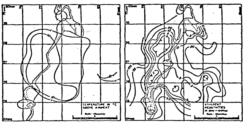
A. TEMPERATURE AT 15m DEPTH B. APPARENT RESISTIVITY SURVEY USING WENNER CONFIGURATION A = 180m.
