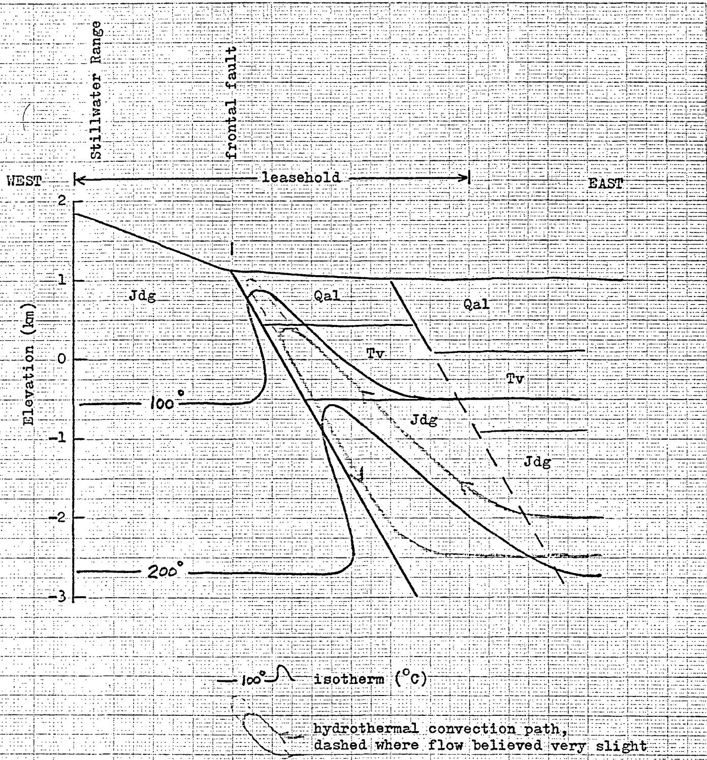
Plate 15. Schematic model of hydrothermal convection and temperature gradient, Quest leasehold and vicinity, Dixie Valley, Nevada. Section transverse to plane of frontal fault.
