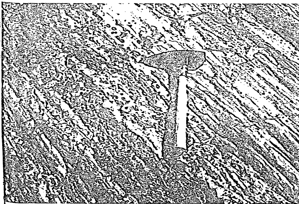
Figure 4. Grooves on a slickensided fault surface in Dixie Valley. The length of the hammer head is
