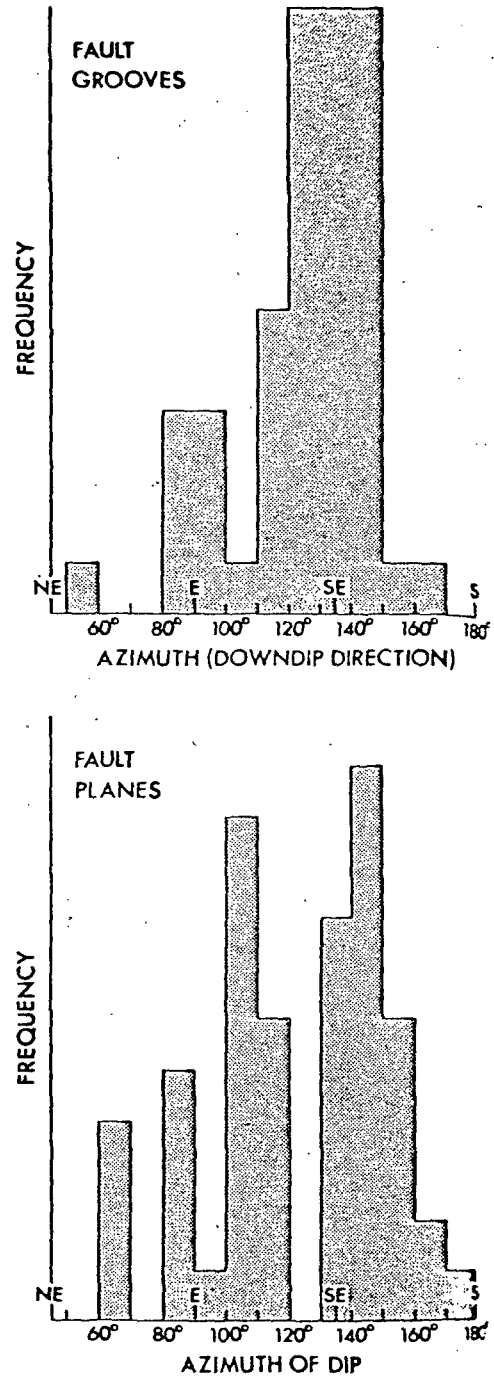
Figure 5. Histograms of the azimuths of fault plane grooves (above) and fault plane dips (below) on the western side of Dixie Valley. Fifty-four measurements for each are represented.
