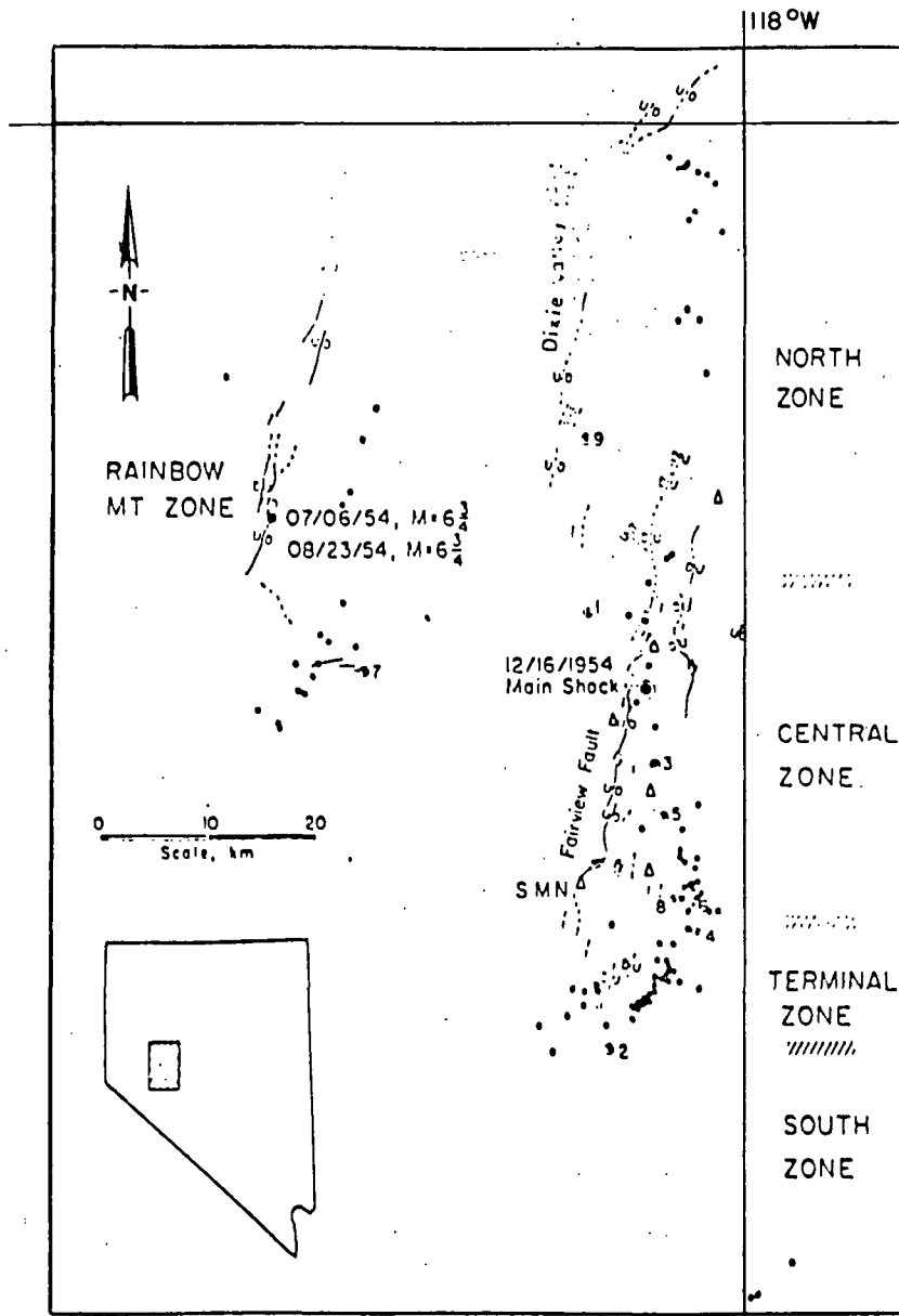
Rainbow Mountain-Dixie Valley-Fairview Peak area, showing fault breaks mapped by Tocher (1956) and Stenmons (1957), epicenters of large earthquakes in 1954 (large double circles), reismograph stations used in field studies (open triangles), earthquakes located during field studies (small double circles), and earthquakes located by analysis of data from the statewide seismic net (small closed circles).
