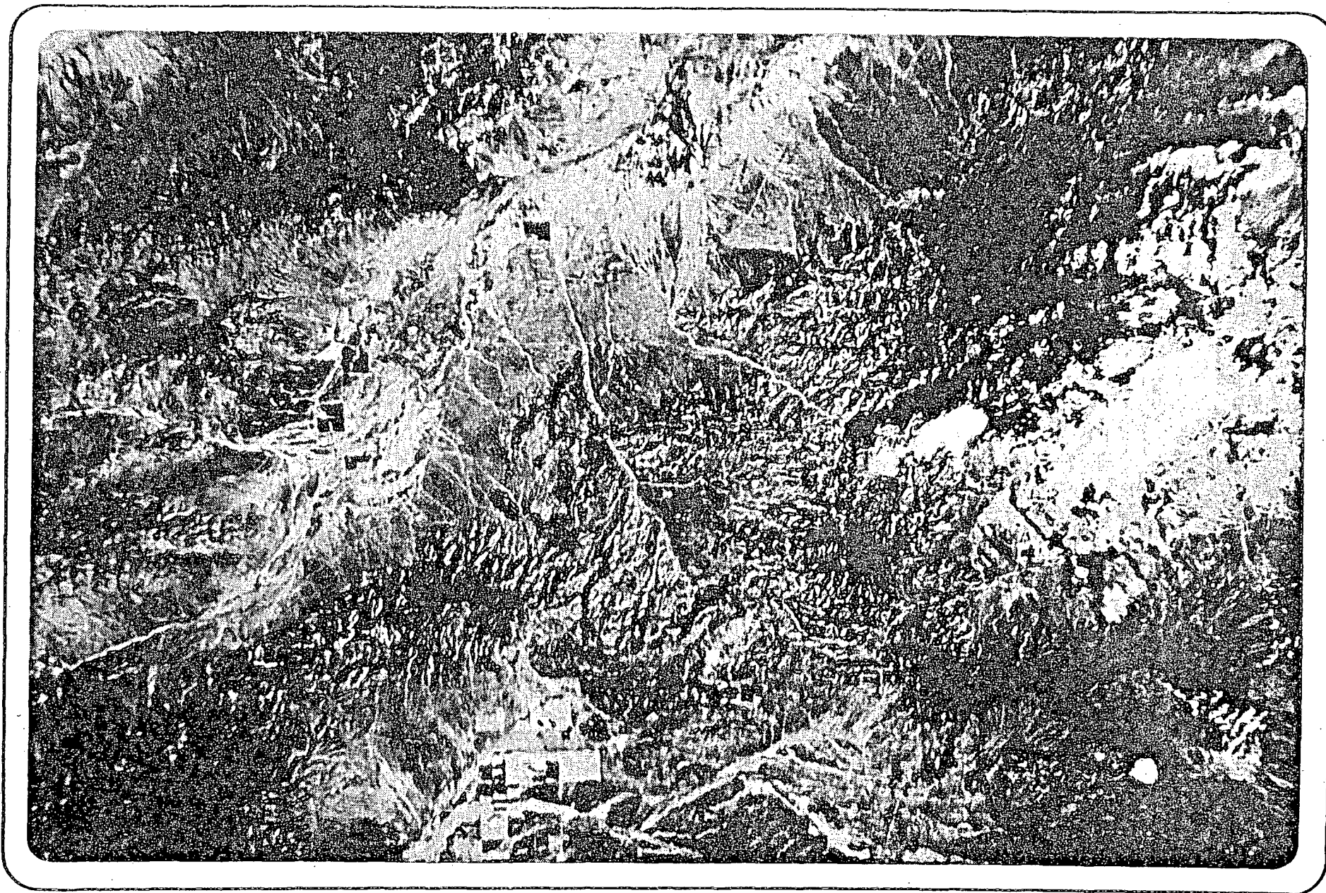
5R. Partial Landsat image showing the ring in center surrounding the McCoy prospect. Hole in the Wall wash drains the ring and empties into Dixie Valley on the west
