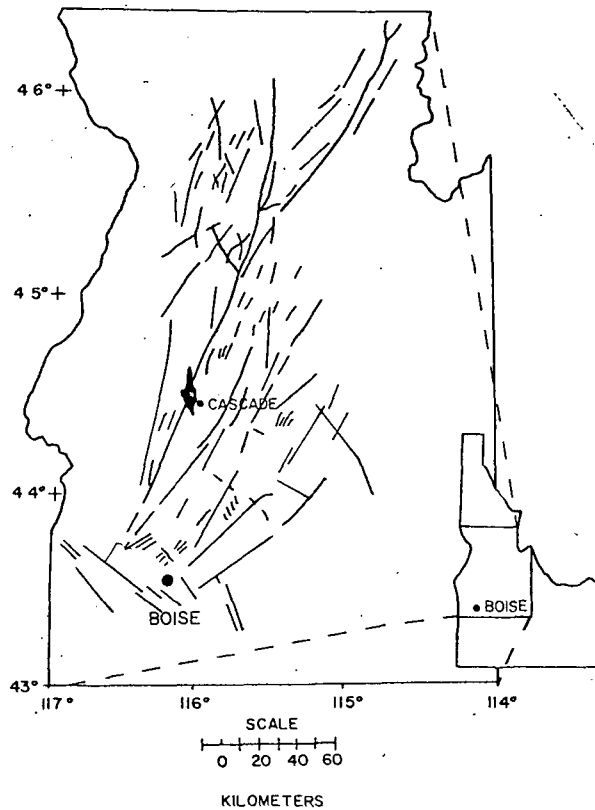
Fig. 2. Map showing major Landsat features in a portion of west central Idaho (modified from Day [1974]).
