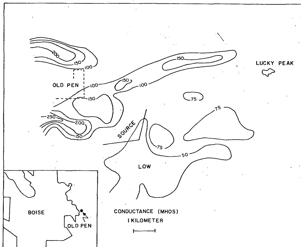
Fig. 4. Total longitudinal conductance map for a portion of the Boise area. The longitudinal conductance assumes cylindrical current spreading. Several major structural trends are prominent.
