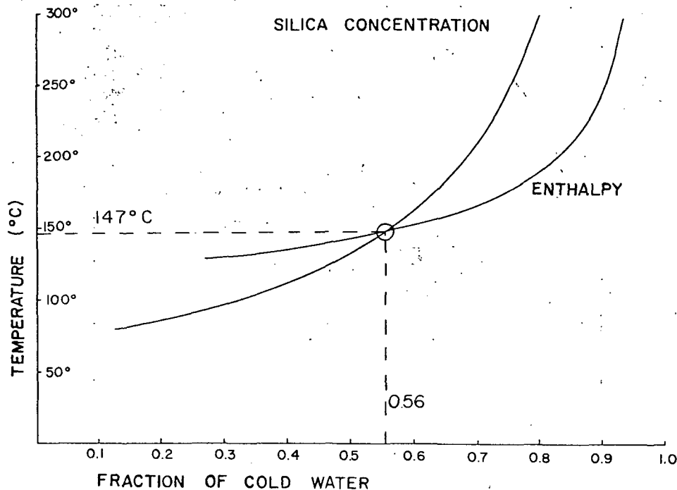
Fig. 8 Graph illustrating a mixing model calculation of a silica predicted temperature for the undiluted reservoir at Cabarton Hot Springs at the south end of Cascade Reservoir. The predicted reservoir temperature is 147^{\circ}\text{C} with 56% cold-water dilution for the spring.
