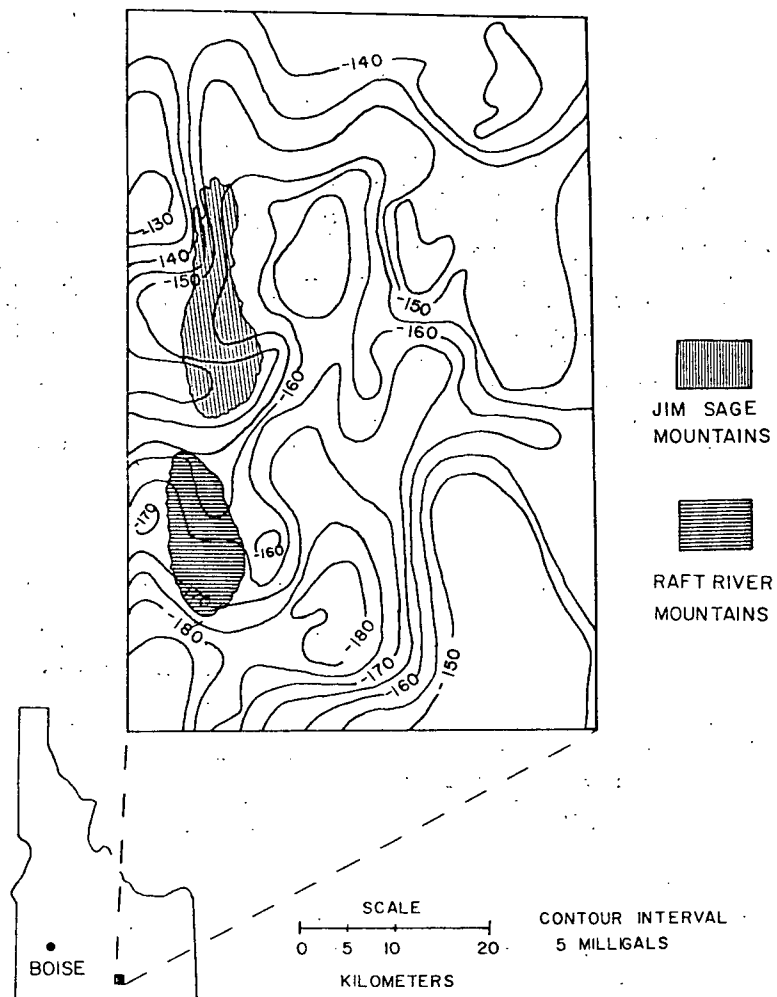
Fig. 10. Gravity map of the Raft River Valley. The Narrows structure separates the Jim Sage Mountains from the Raft River Mountains. The Bridge fault is along the eastern flank of the Jim Sage Mountains. Gravity data is from Mabey et al. [1974].
