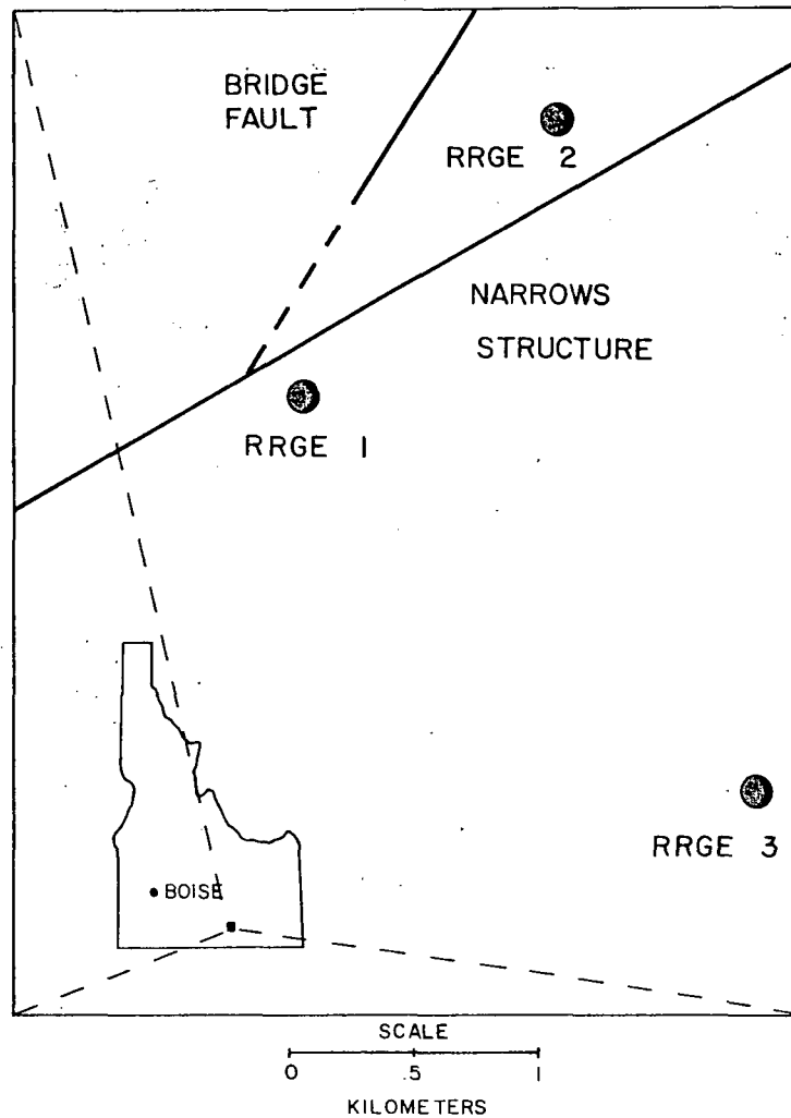
Fig. 9. Schematic map of the Bridge fault, the Narrows structure, and RRGE 1, 2, and 3. The Bridge fault is along the eastern flank of the Jim Sage Mountains, and the Narrows structure separates the Jim Sage Mountains from the Raft River Mountains (Fig. 10).
