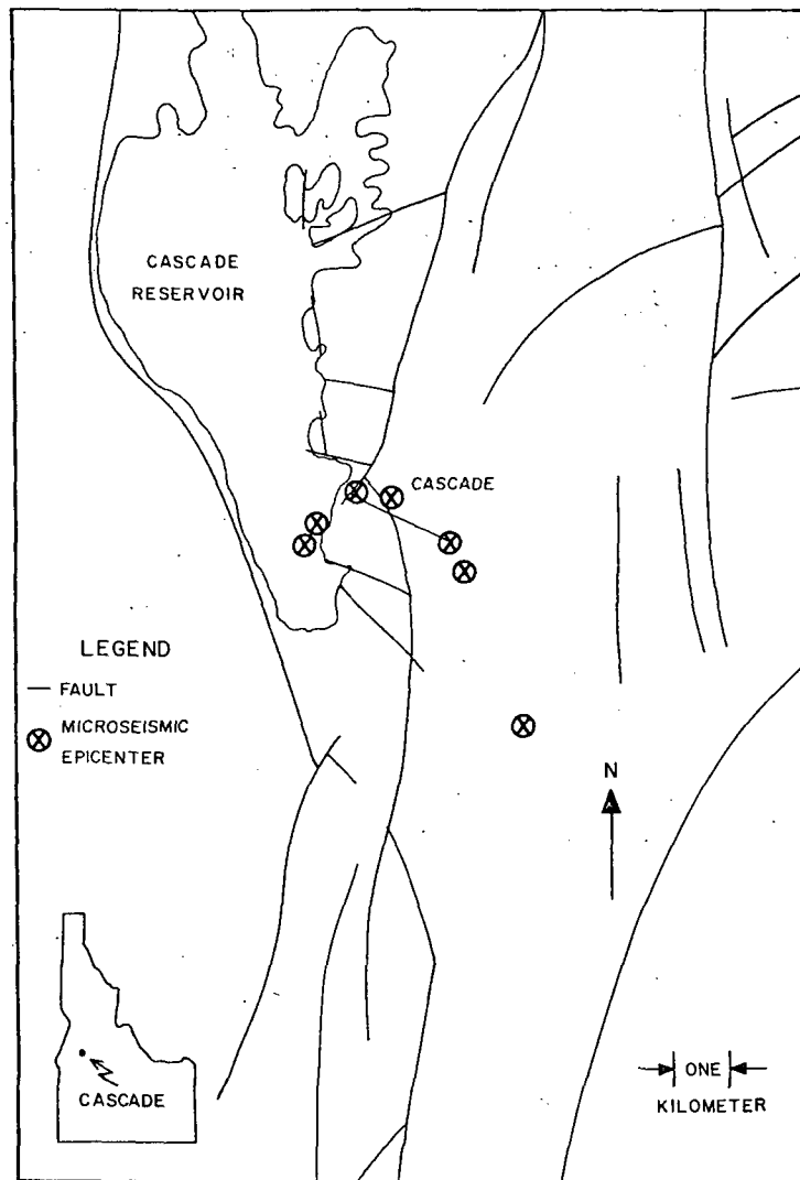
Fig. 7 Map of the Cascade area showing relationship between mapped faults and microseismic events recorded in one 8-day period.
