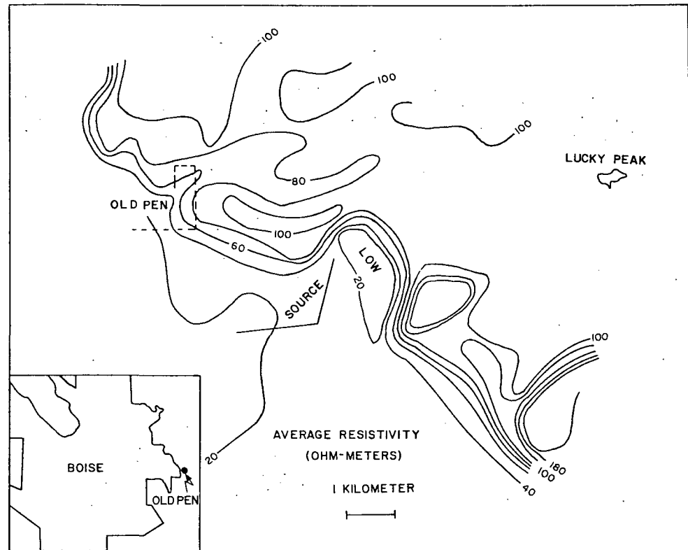
Fig. 3. Average resistivity map for a portion of the Boise area. The average resistivity is obtained by determining the apparent resistivity with the rotating bipole source and roving dipole receiver. A number of structural trends are clearly shown by the contours.
