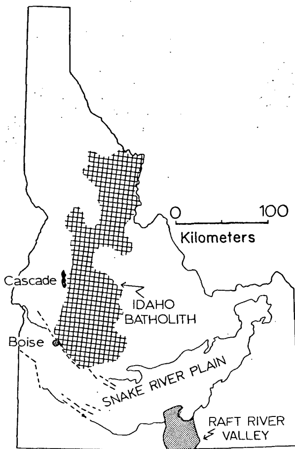
Fig. 1. Index map showing locations of the three (Boise, Cascade, and Raft River) geothermal areas to be discussed and their spatial relationships to the Idaho Batholith and the Snake River Plain.
