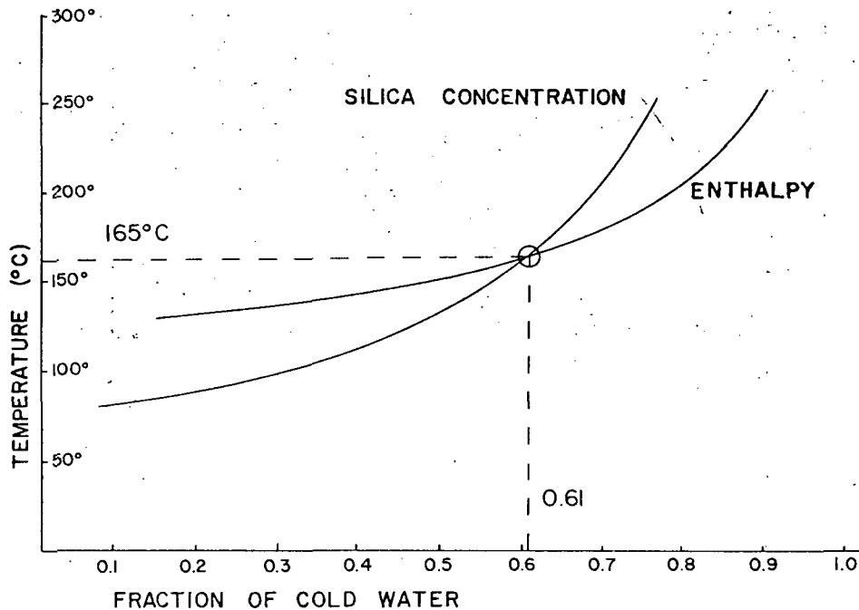
Fig. 6 Graph illustrating a mixing model calculation of a silica predicted temperature for the undiluted reservoir at Boise. The predicted temperature is 165°C with 61% dilution for the water produced.
