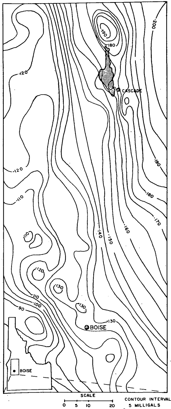
Fig. 5 Regional gravity map of a portion of west central Idaho showing the apparent lack of shallow intrusives [Mabey et al. 1974].
