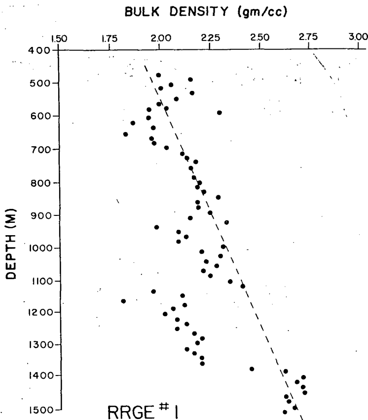
Fig. 11. Plot of bulk density from density log versus depth for RRGE 1. The general trend is that density increases with depth in a sedimentary sequence because of increasing compaction and decrease of porosity. The graph then shows a decrease in porosity with depth until the productive zone (1150 to 1370 m) is encountered [Applegate et al., 1976].
