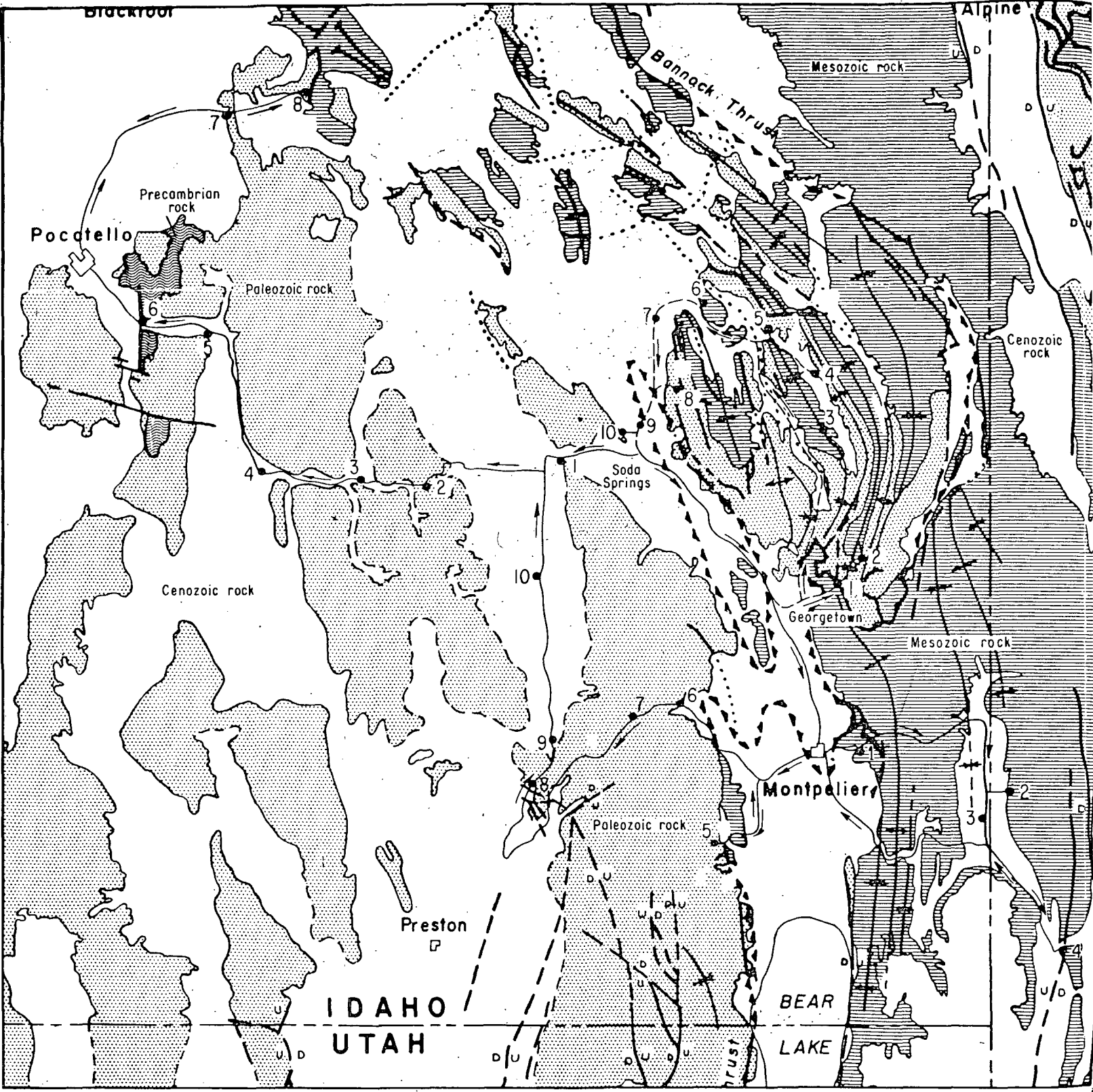
from Anatomy of The Western Phosphate Field, 15th Ann. by Conf. of Intermountain Assoc. of Geol.
