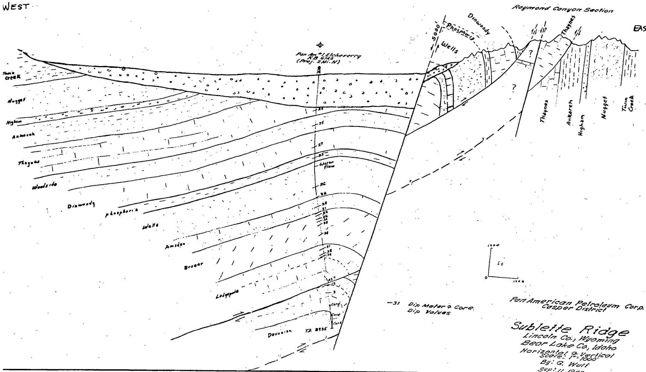
STOP #3 West to East Geologic Cross Section SUBLETTE ANTICLINE
