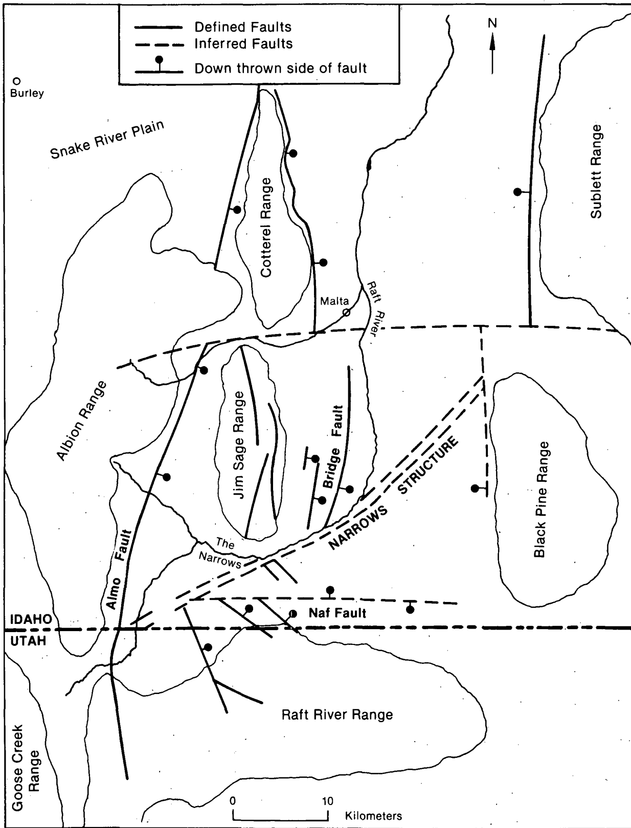
Figure 1. Generalized geological map of the Raft River valley region.
