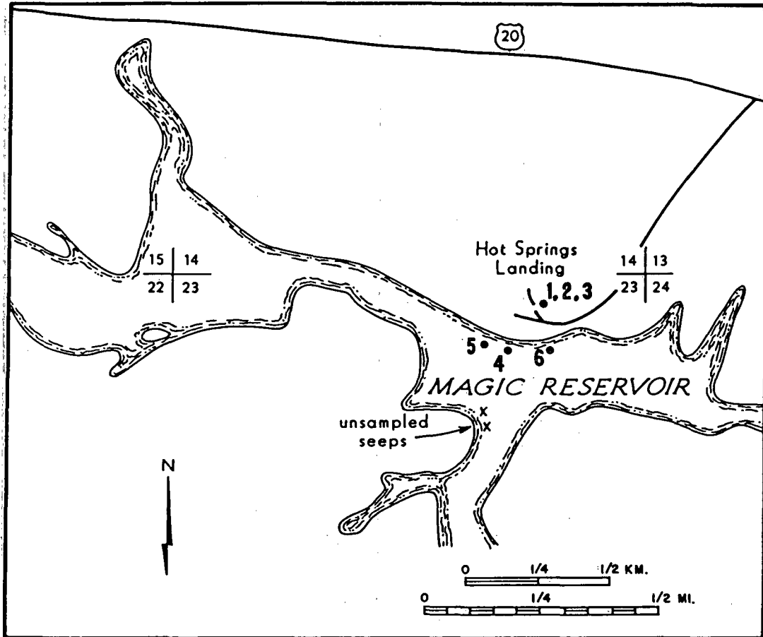
FIGURE 3. WATER SAMPLE SITES, MAGIC RESERVOIR AREA
