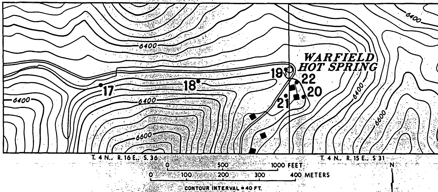
FIGURE 6. WATER SAMPLE SITES, WARFIELD HOT SPRING AREA
