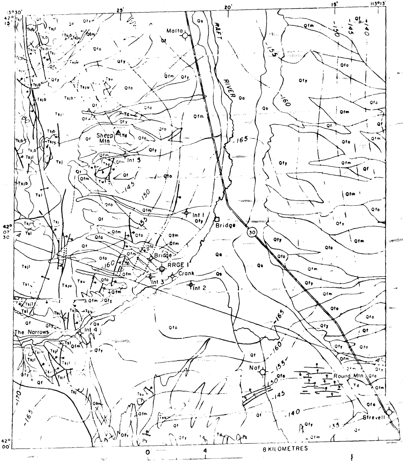
Figure 2.--Geologic and gravity map of the southern Raft River Valley
