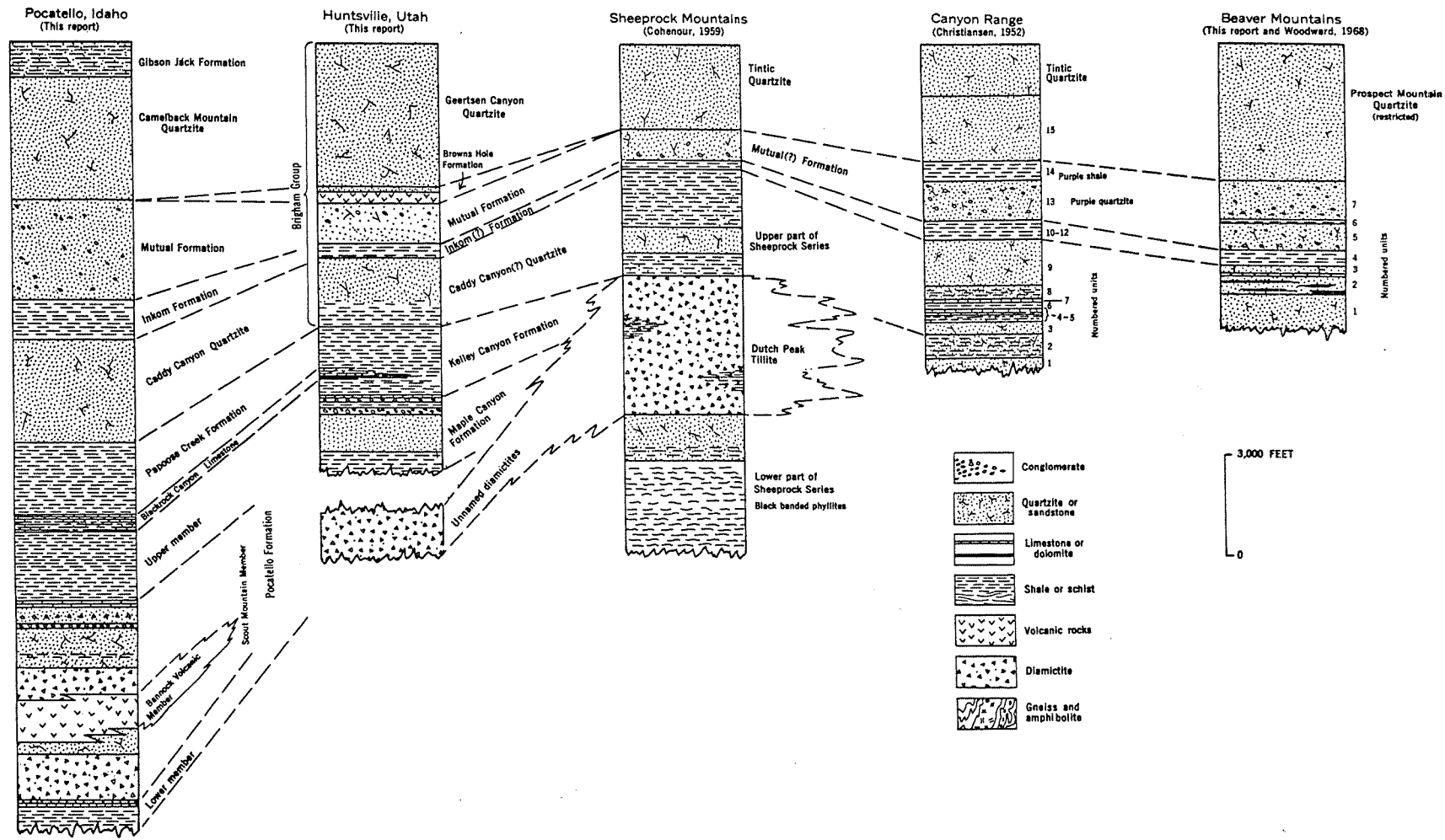
Figure 7. North-south correlation of younger Precambrian and basal Cambrian rocks from Pocatello, Idaho, to Beaver Mountains, Utah.
