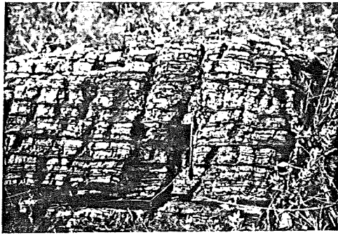
Figure 6. Tan-weathering laminated dolomite at base of Kelley Canyon Formation, near Huntsville, Utah.
