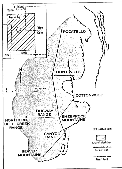
Figure 1. Index map showing location and tectonic setting of stratigraphic sections described.
