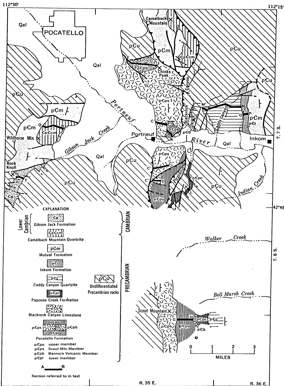
Figure 2. Map of area near Pocatello, Idaho, showing location of type sections for newly described Precambrian and Cambrian units.
