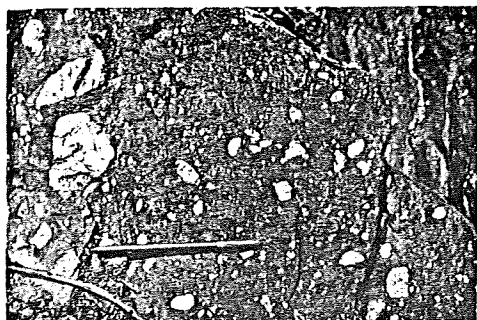
Figure 4. Diamictite consisting of subrounded to subangular clasts of quartzite, granitic rocks, and carbonates in a black fine-grained matrix. Exposures are in Willard thrust sheet north of Willard Peak, Utah.
