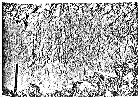
Figure 5. Argillite member of Maple Canyon Formation near Huntsville, Utah. Crenulated bedding is nearly vertical, parallel to schistosity dips 30° to left.
