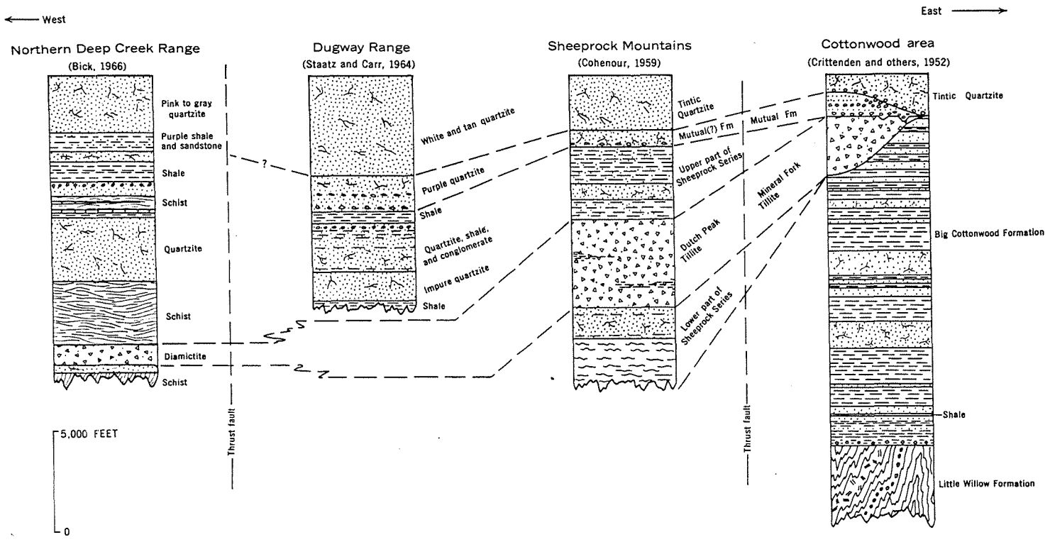
Figure 8. East-west correlation of younger Precambrian and basal Cambrian rocks in western Utah.
