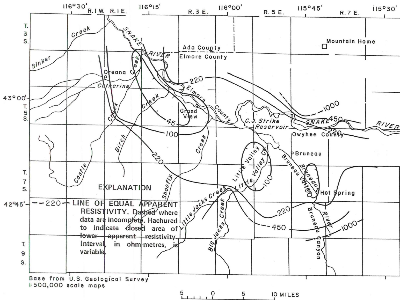
FIGURE 21. Apparent resistivity map at 270 hertz.
