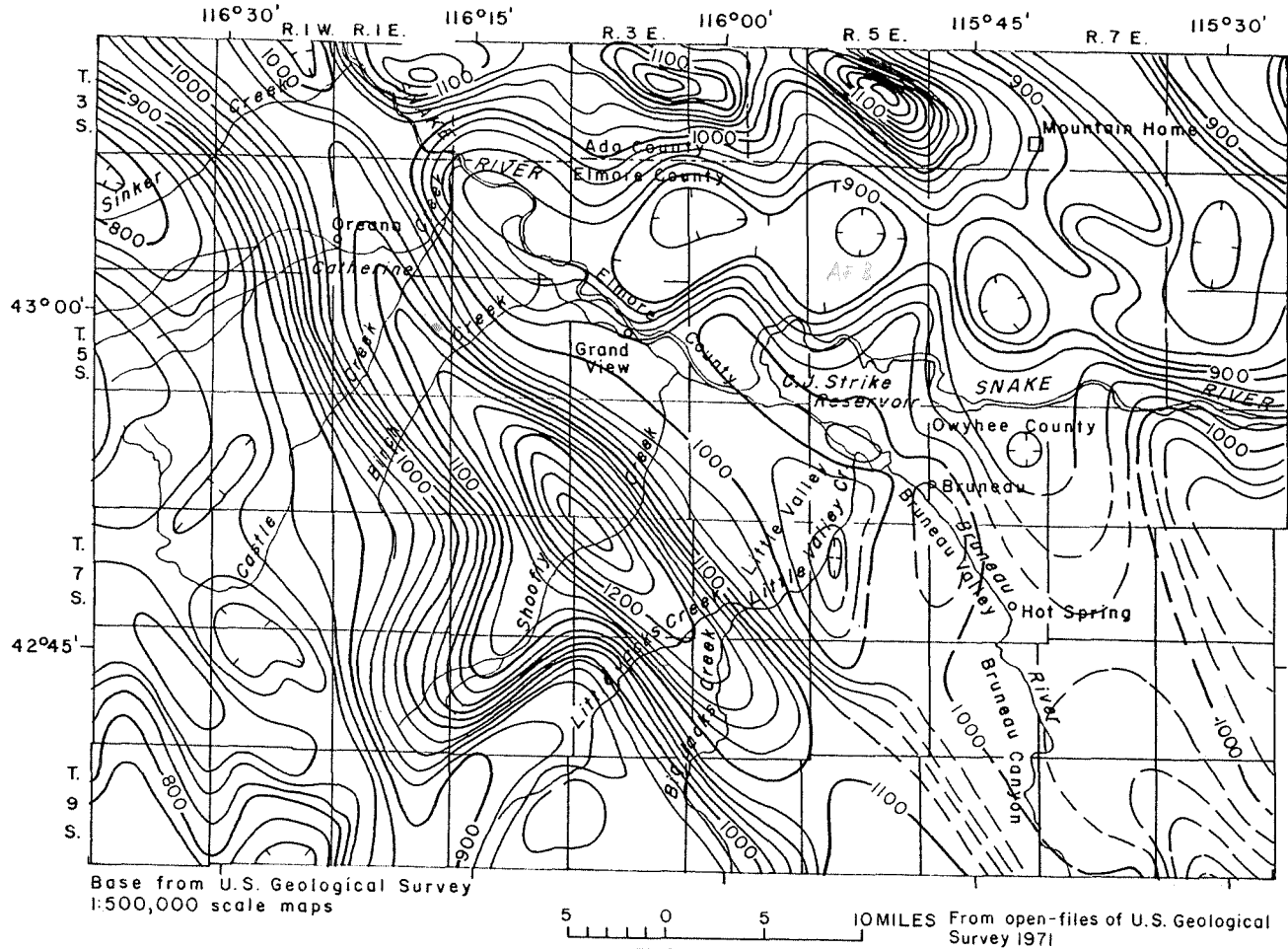
FIGURE 8. Aeromagnetic map.
