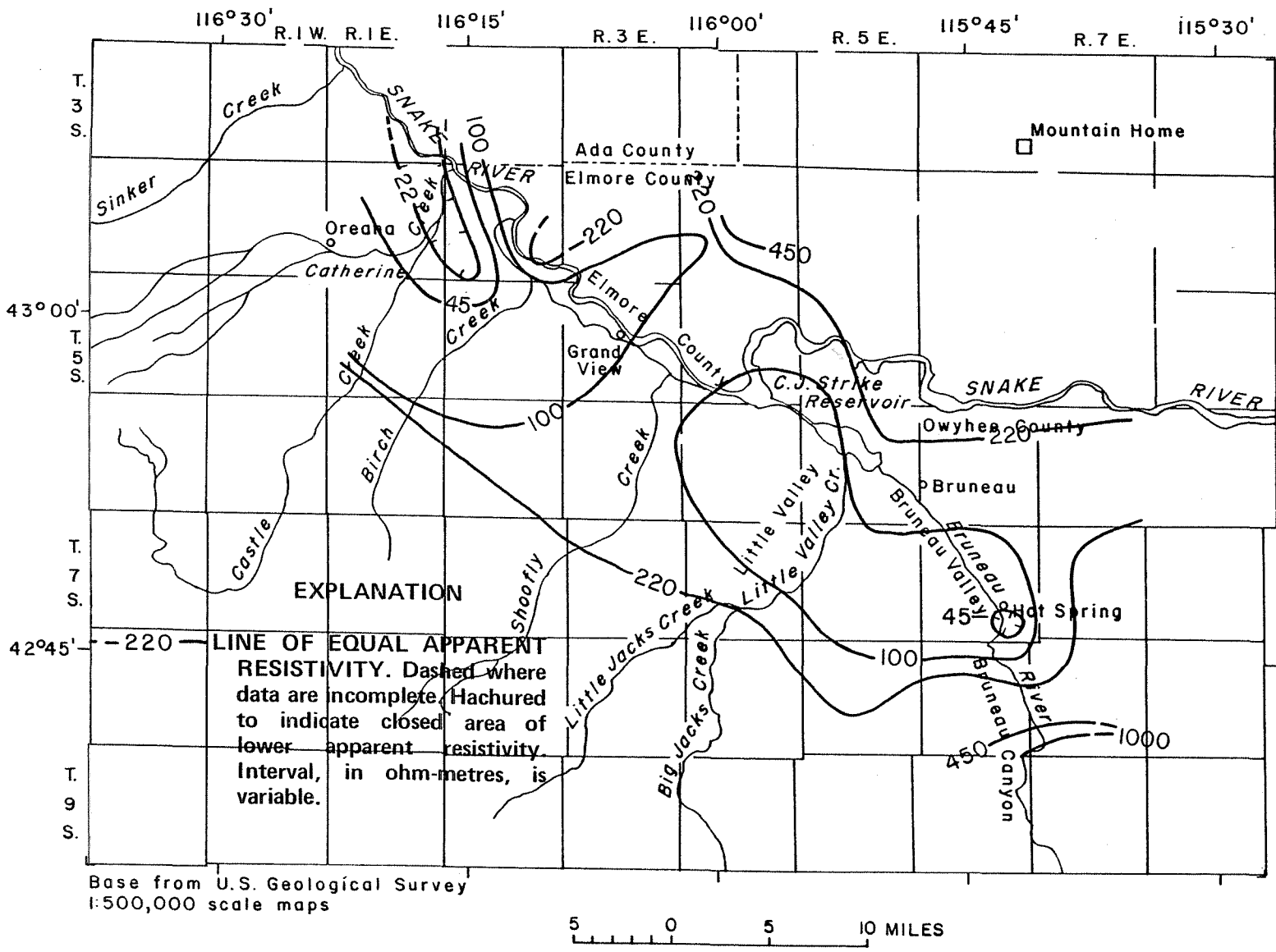
FIGURE 22. Apparent resistivity map at 700 hertz.
