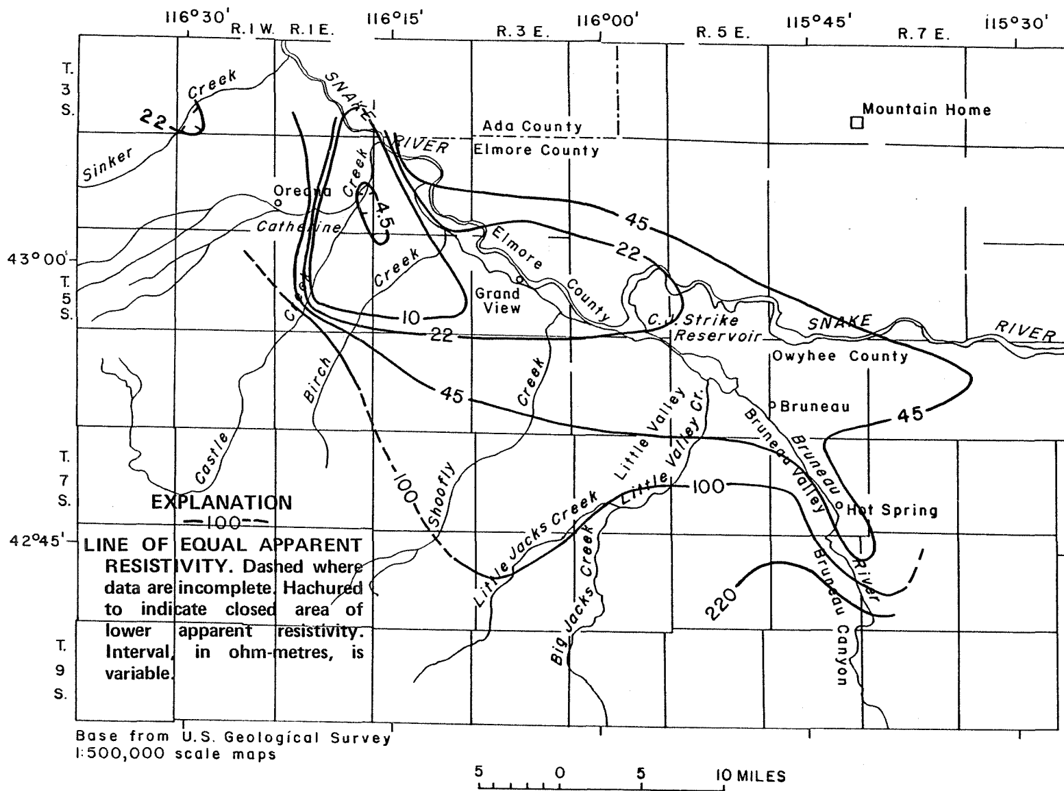
FIGURE 14. Apparent resistivity map at 8 hertz.
