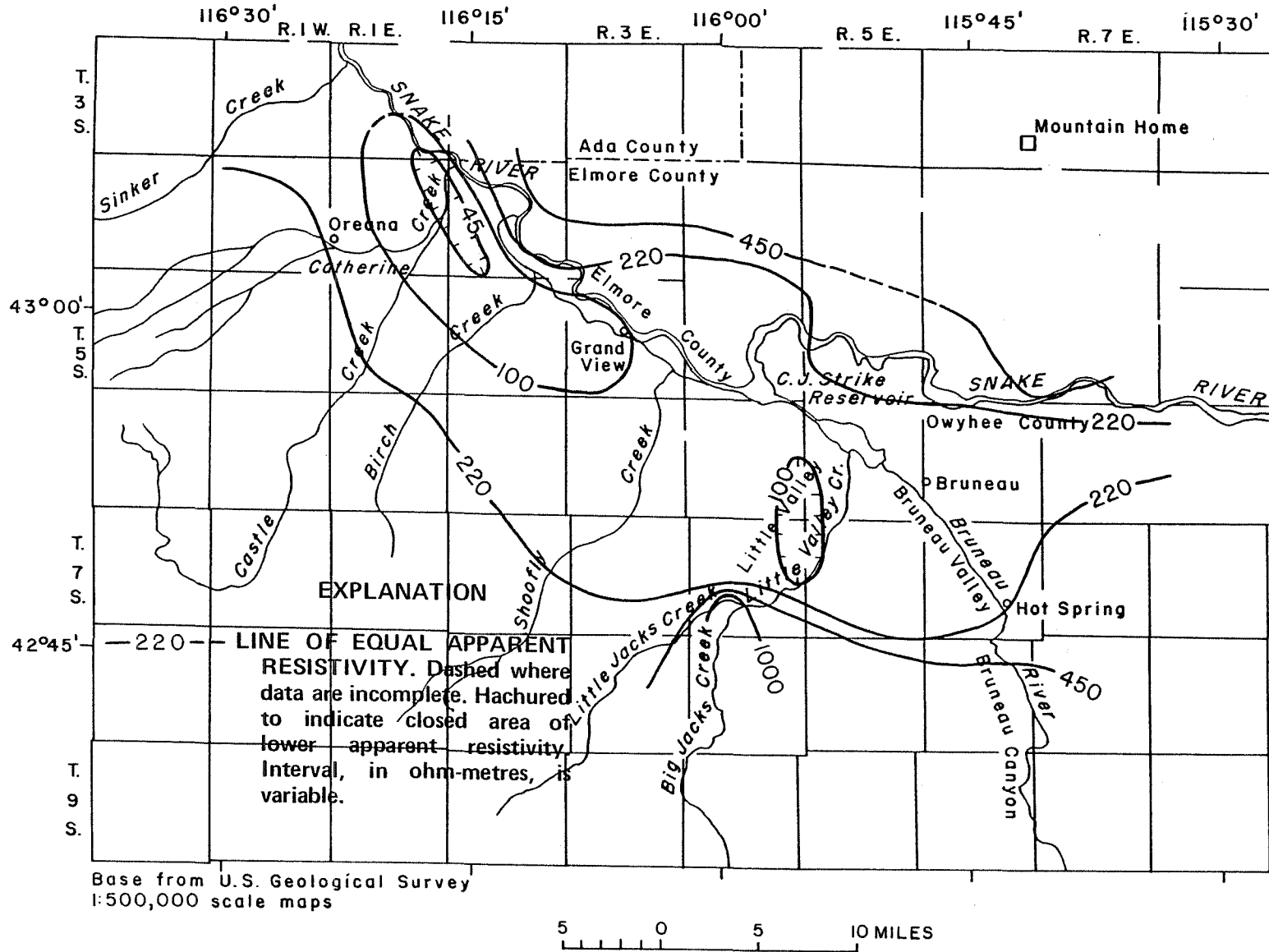
FIGURE 20. Apparent resistivity map at 86 hertz, electric line east-west.
