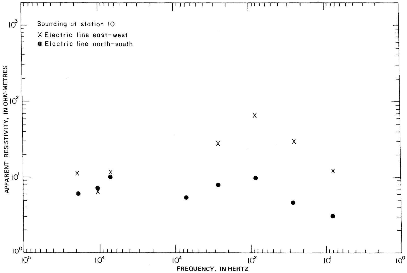
FIGURE 18. Apparent resistivities at station 10.
