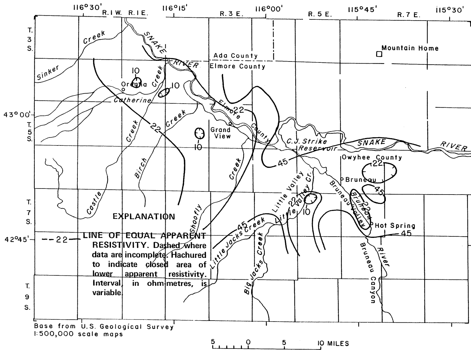
FIGURE 24. Apparent resistivity map at 18,600 hertz.
