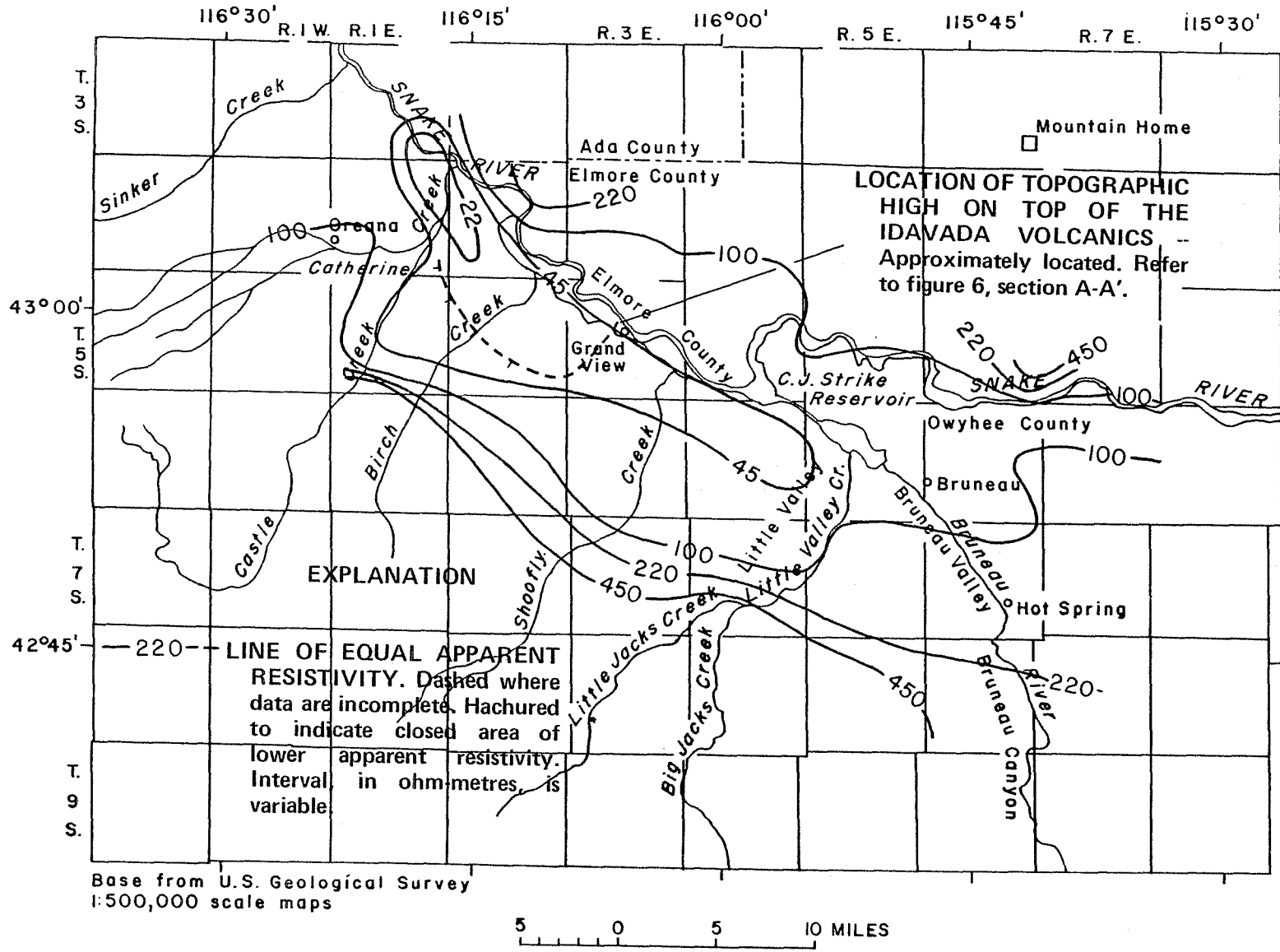
FIGURE 16. Apparent resistivity map at 26 hertz, electric line east-west.
