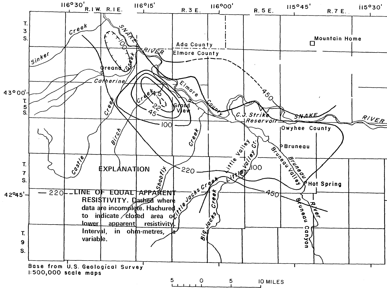
FIGURE 19. Apparent resistivity map at 86 hertz, electric line north-south.
