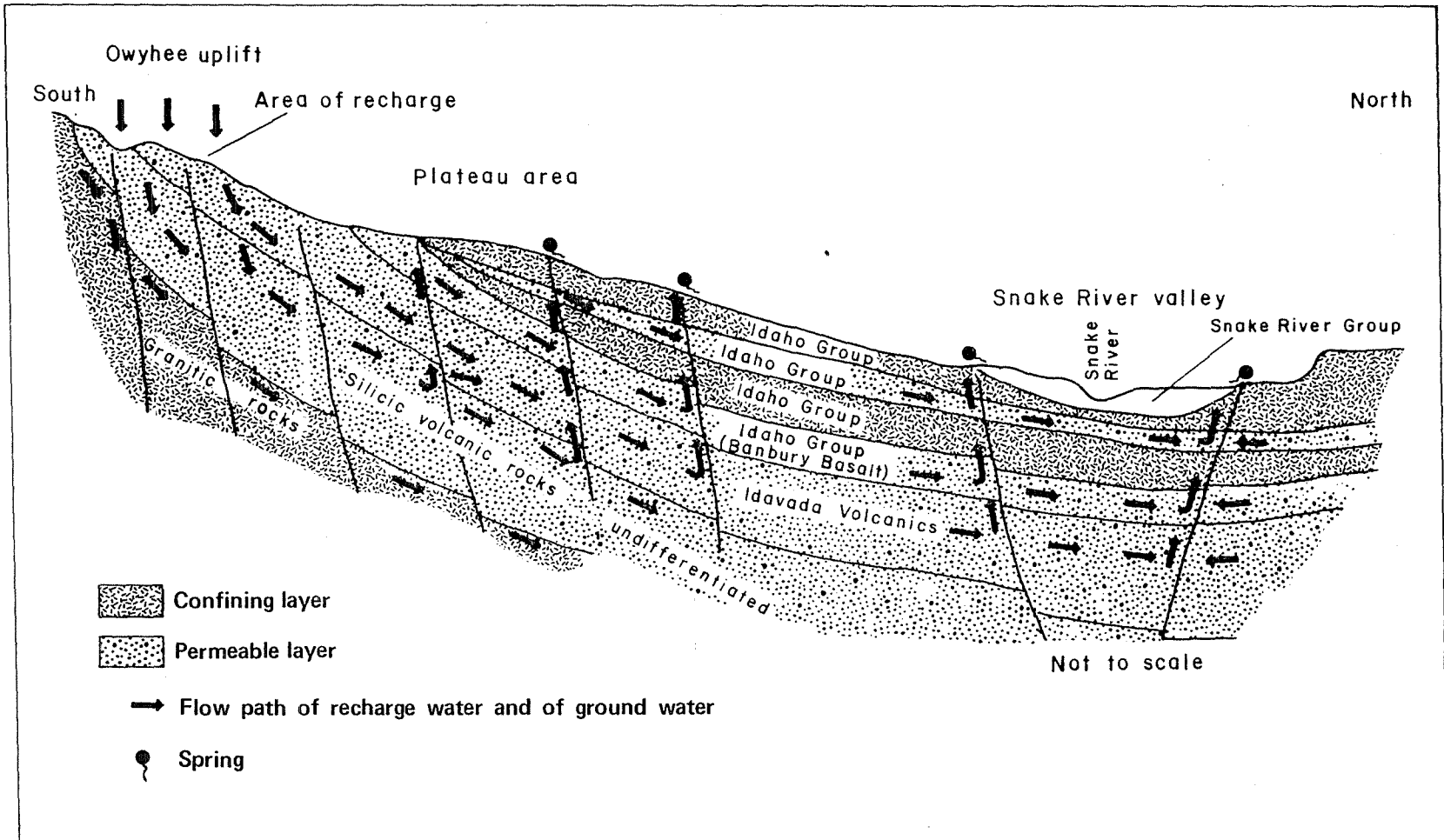
FIGURE 5. Idealized hydrogeologic section showing general relation of geologic units, recharge, and ground-water movement.
