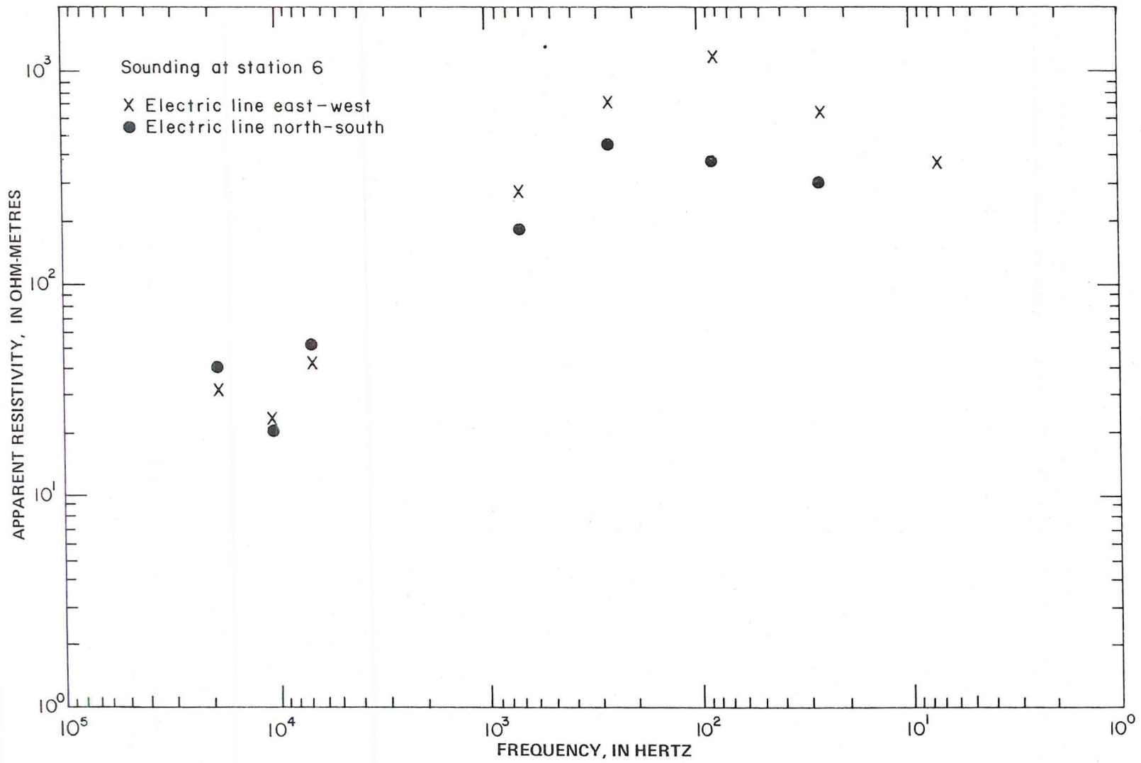
FIGURE 17. Apparent resistivities at station 6.
