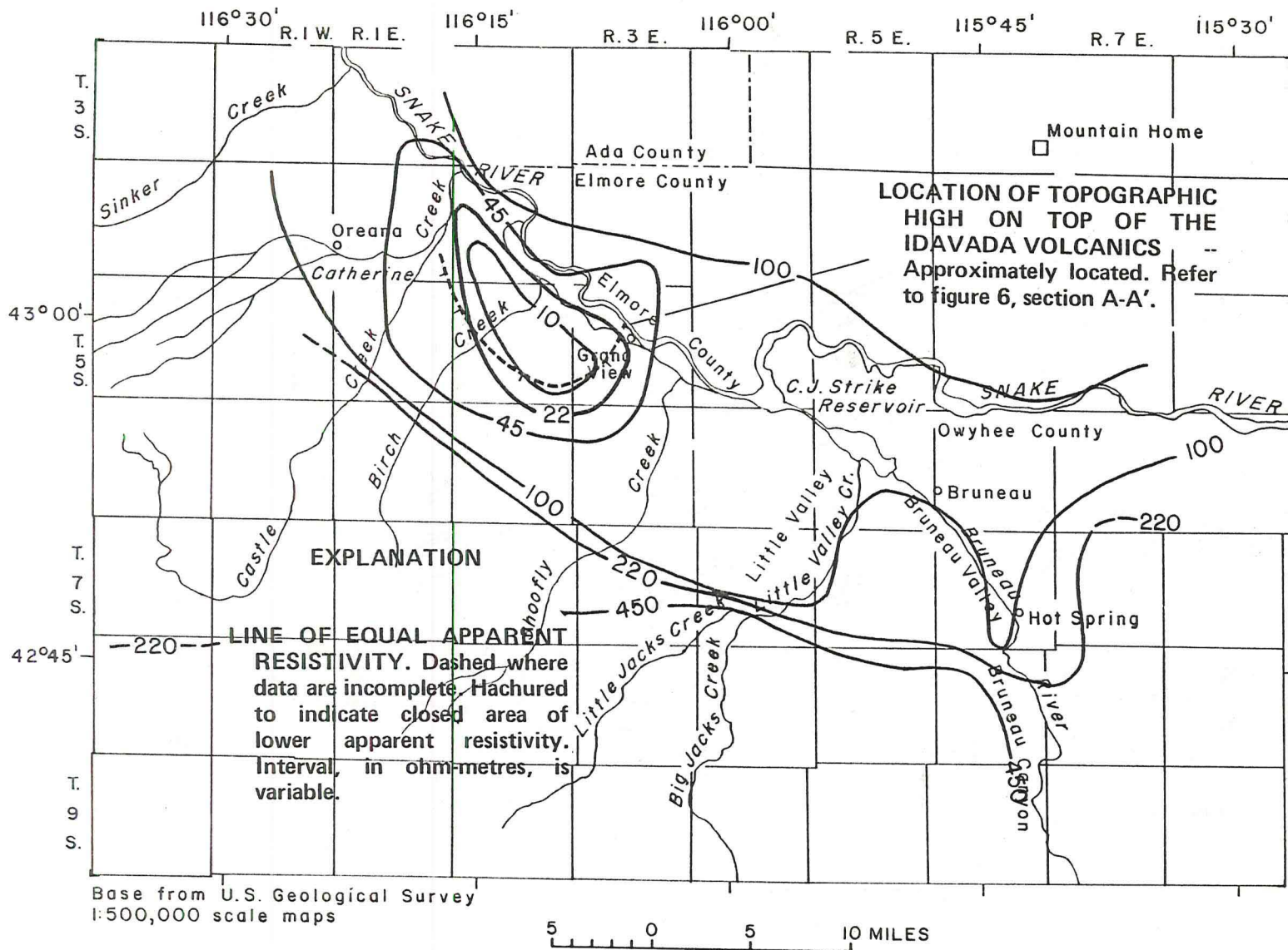
FIGURE 15. Apparent resistivity map at 26 hertz, electric line north-south.
