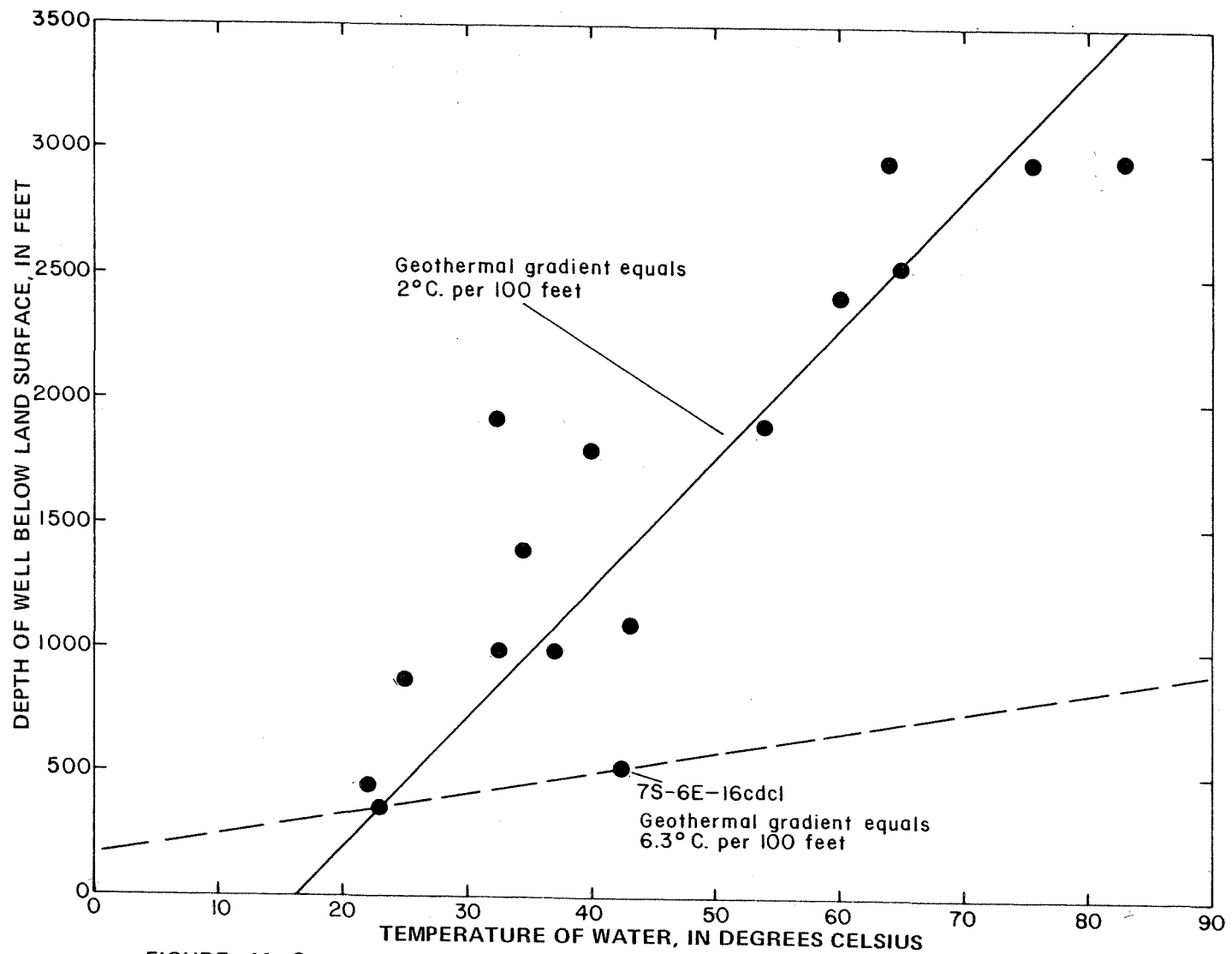
FIGURE 11. Ground-water temperatures with relation to depth in wells having at least 60 percent of the upper part of the well cased.
