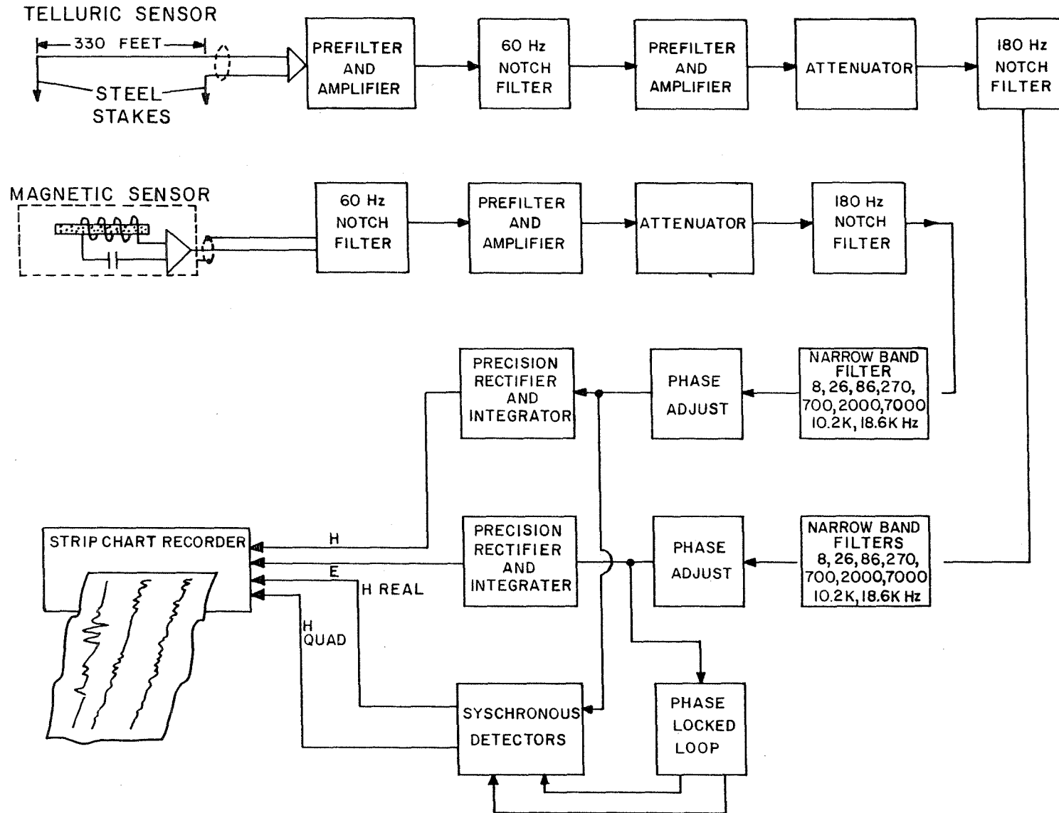
FIGURE 12. U.S. Geological Survey AMT (audio-magnetotelluric) system.
