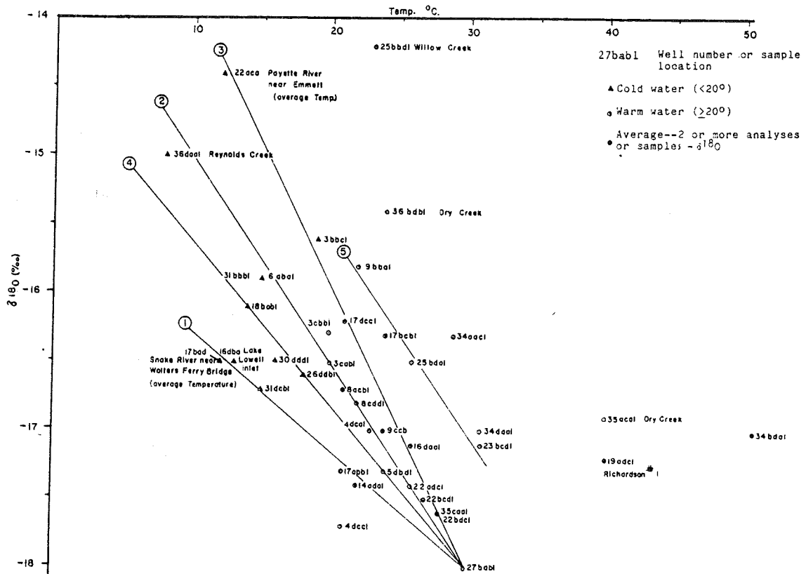
FIGURE 4-6. Measured surface temperatures of selected wells and surface waters versus \delta^{18}\text{O} in the Nampa-Caldwell and adjacent areas of southwestern Idaho.
