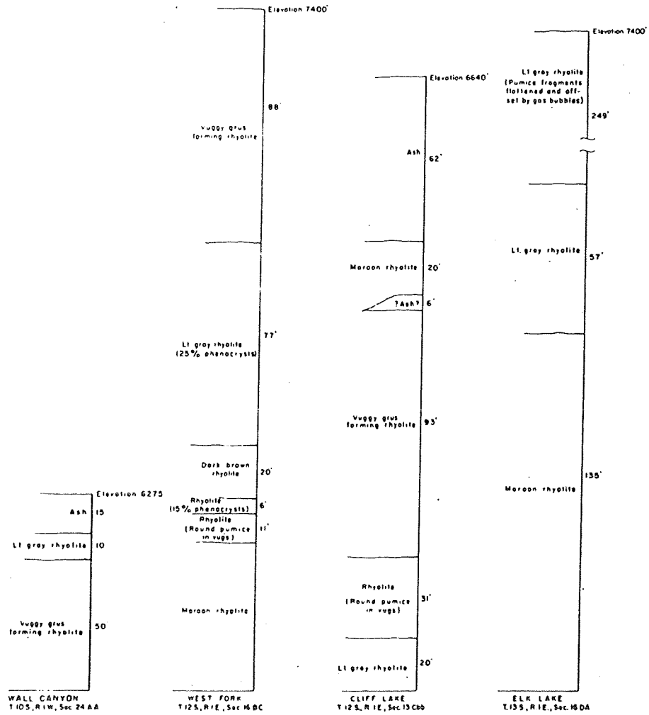
Figure 2. Stratigraphic sections of young volcanic rocks.
