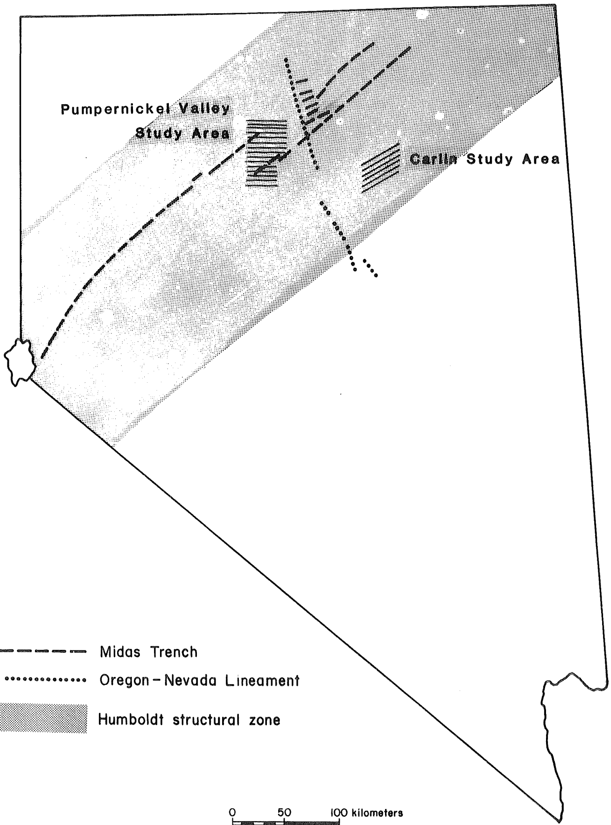
Figure A4. Location and trend of regional structural elements (modified after Rowan and Wetlauffer, 1975, 1981).
