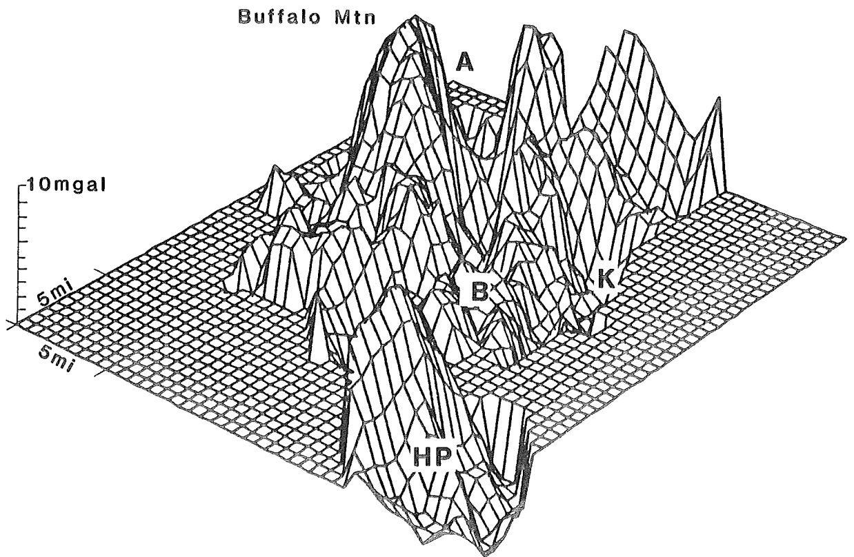
Figure A11. 3-dimension computer generated residual gravity map of Pumpernickel Valley, looking southwest: B, Brooks Spring; HP, Blossom Hot Pot; K, Kemp thermal anomaly (NCAR plot).
