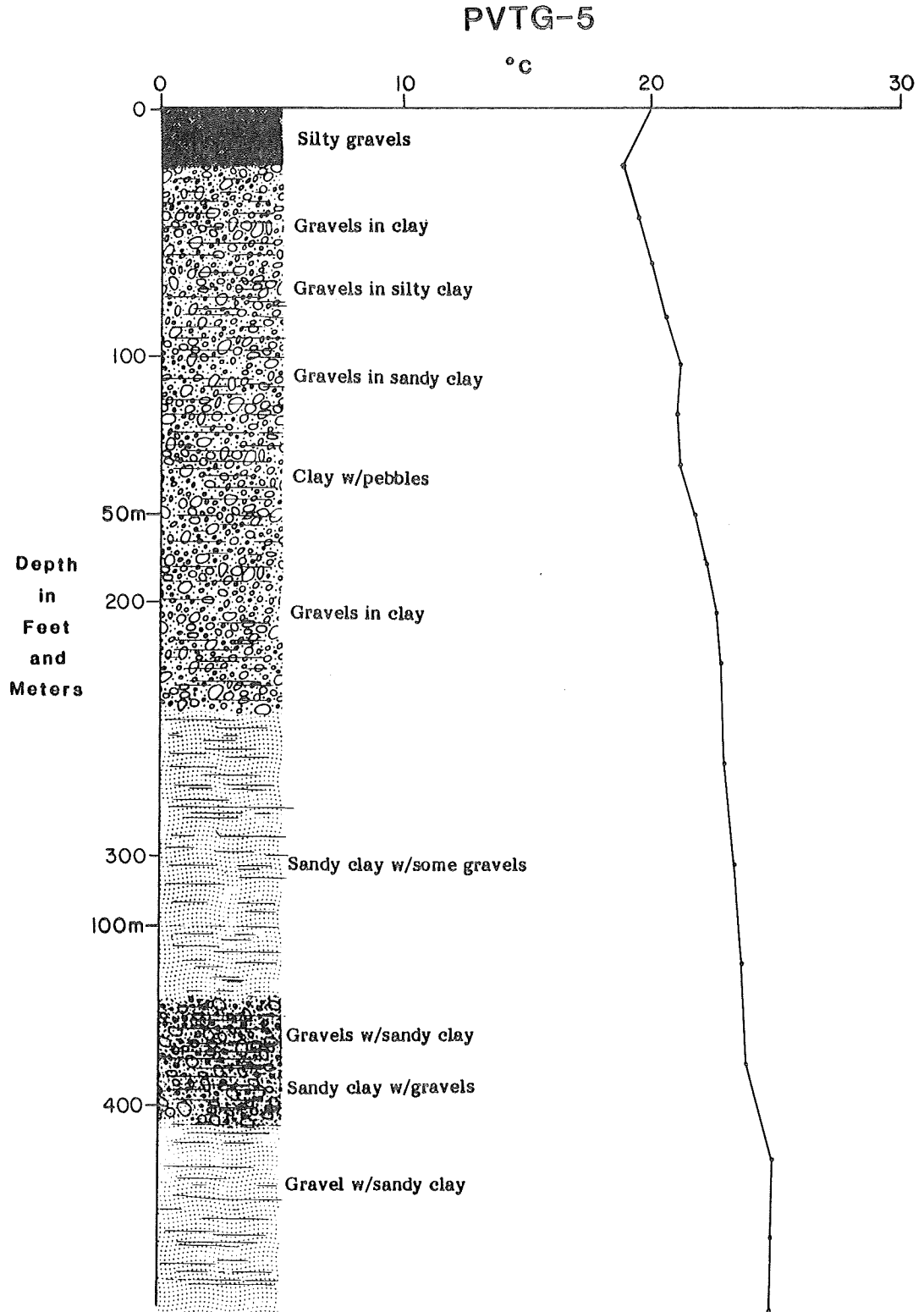
Figure A30. Lithologic log and temperature-depth profile of PVTG-5 in Pumpnickel Valley.
