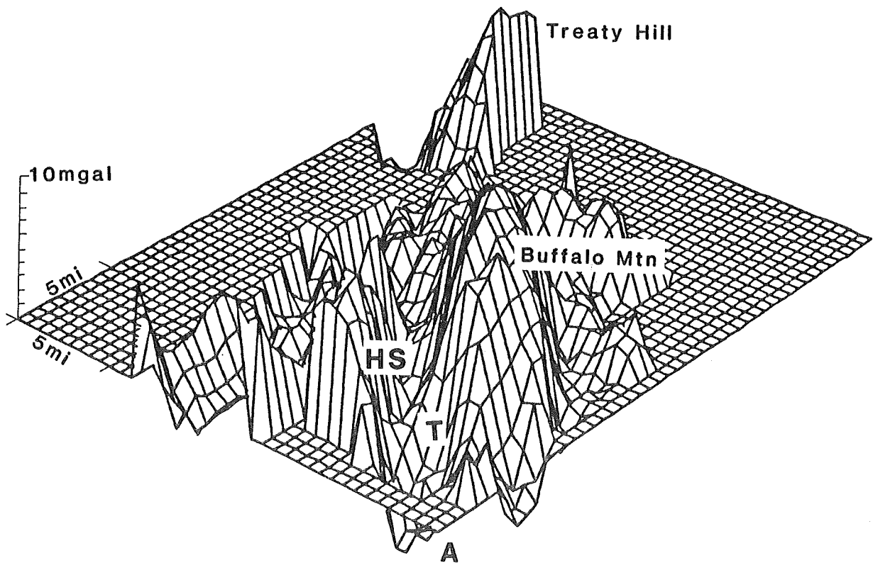
Figure A9. 3-dimension computer generated residual gravity map of Pumpnickel Valley, looking northeast: HS, Hot Springs Ranch; T, Tipton II ranch (NCAR plot).
