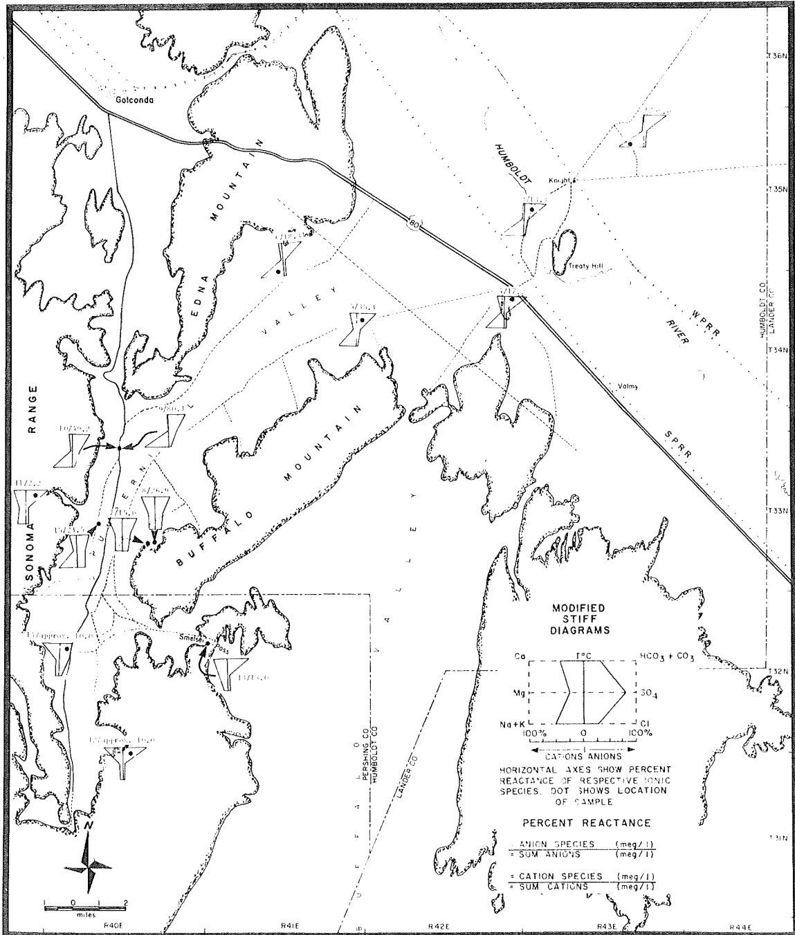
Figure A15. Modified Stiff diagram - Pumpernickel Valley study area.
