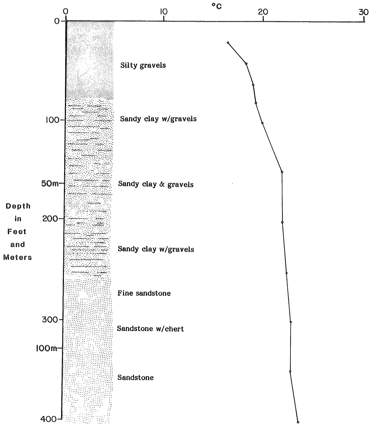
Figure A27. Lithologic log and temperature-depth profile of PVTG-2 in Pumpnickel Valley.
