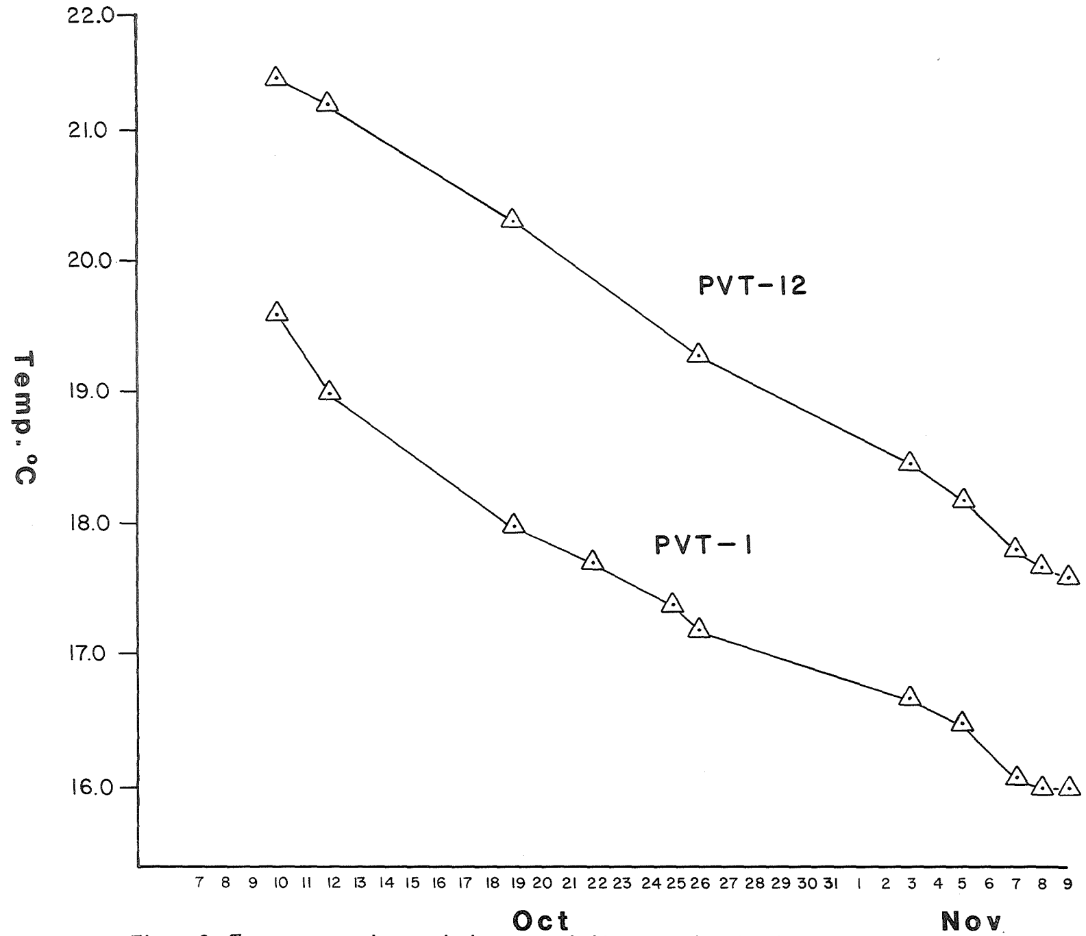
Figure 2. Temperature-time variations recorded by control probes in the Pumpernickel Valley study area.
