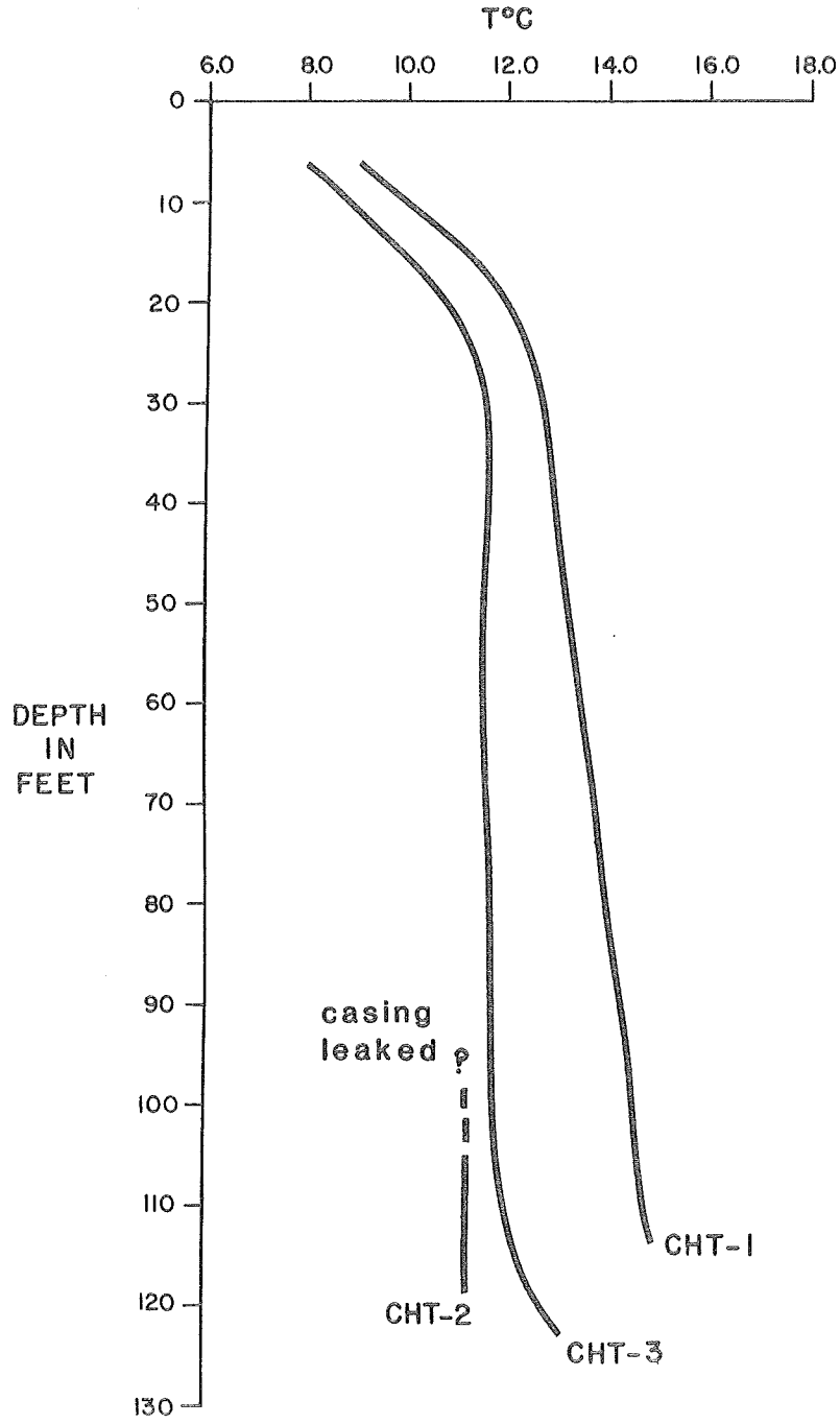
Figure B16. Temperature-depth profiles of CHT-1, 2 and 3 at Carlin; profiles measured on 7 February, 1982.
