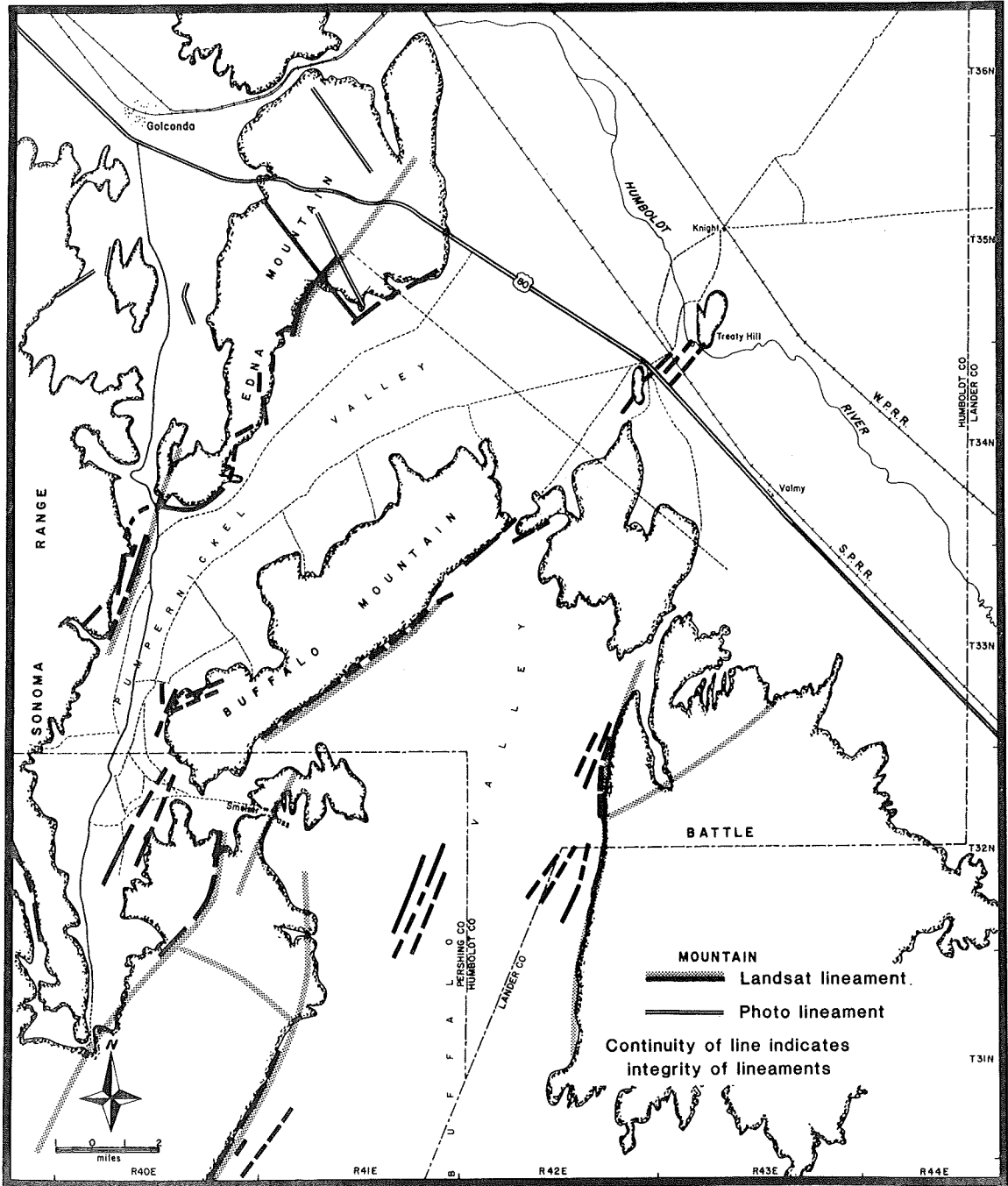
Figure A3. Lineament map of Pumpnickel Valley.
