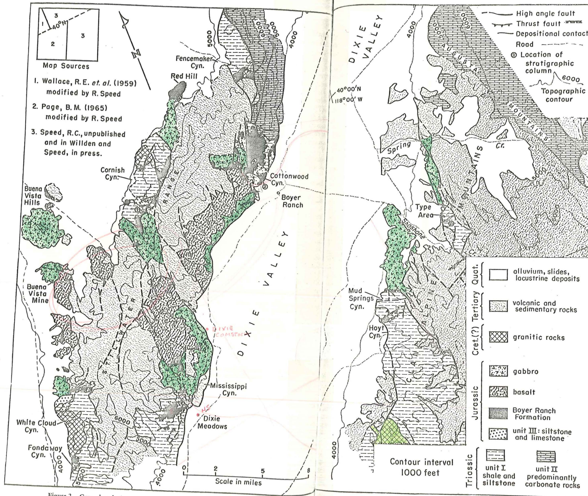
Figure 2. General geologic map of outcrop area of the Boyer Ranch Formation.
