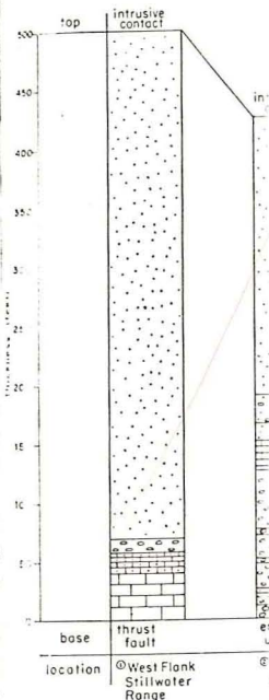
Figure 3. Stratigraphic section locations
