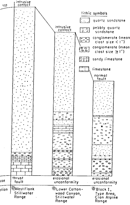
Figure 3. Stratigraphic Sections of Boyer Ranch Formation. Section locations on Figure 2 and Plate 1.
