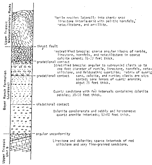
Figure 7. Diagrammatic lithic succession in Boyer Ranch Formation and relations with adjoining units 1 mile north of mouth of Hoyt Canyon, Clan Alpine Mountains.
